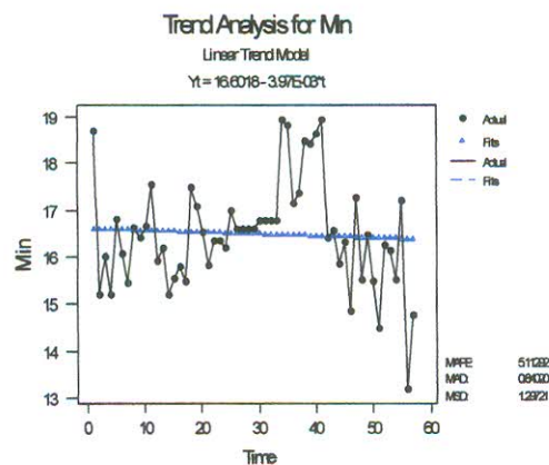
Figure 4.A.5 Trend for minimum monthly ADBT
