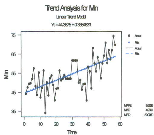
Figure 4.A.13 Trend for minimum monthly ARH
