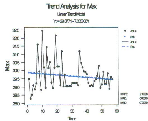
Figure 4.A.6 Trend for maximum monthly ADBT
