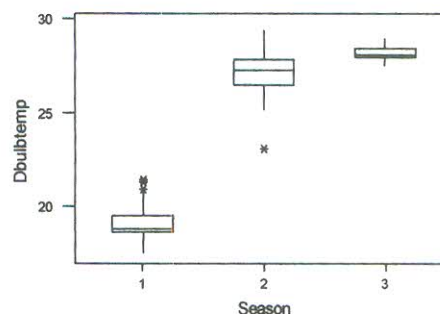
Figure 4.18 Boxplot of seasonal ADBT
