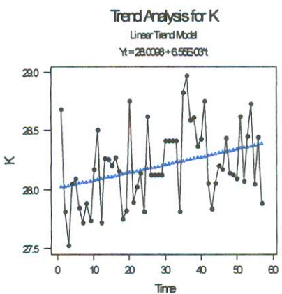
Figure 4.31 Trend of ADBT for Kharif season
