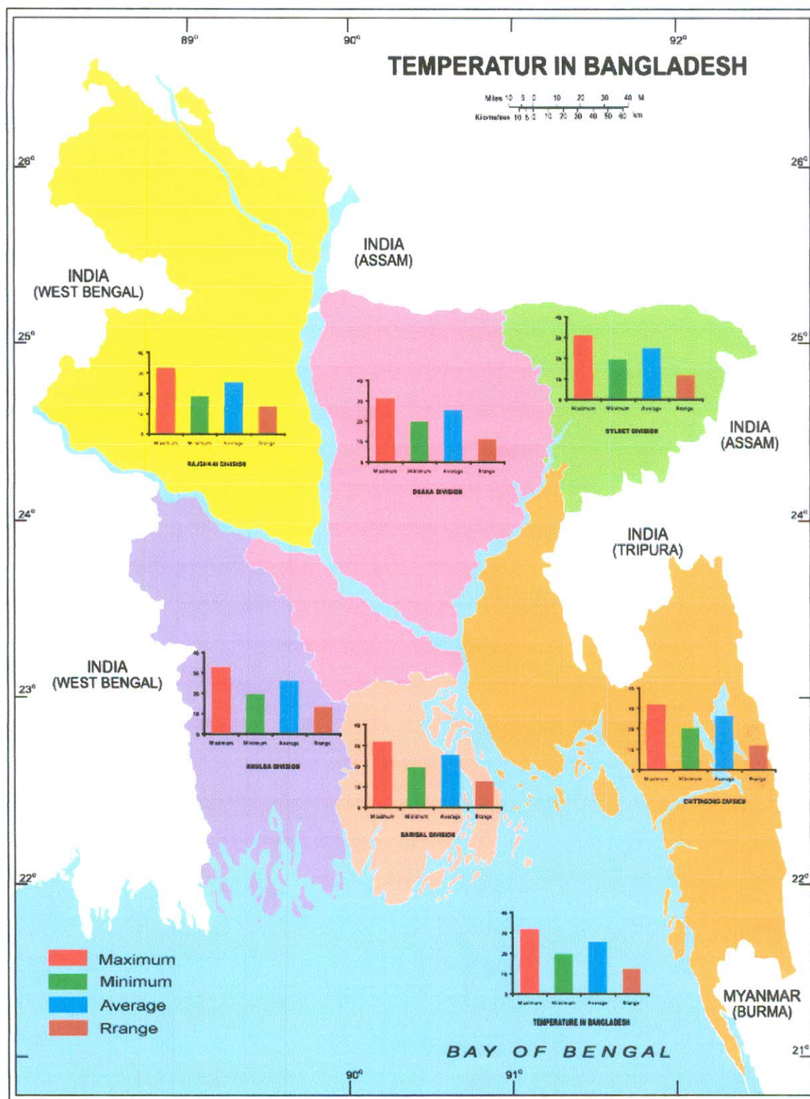
Figure 1 A. 10 Temperature in Bangladesh
