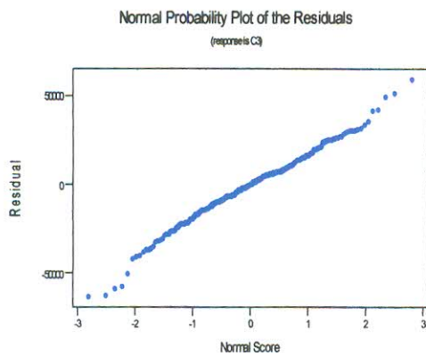
Figure 5.27 Np plot of resid. for ORARH (1981-2004)
