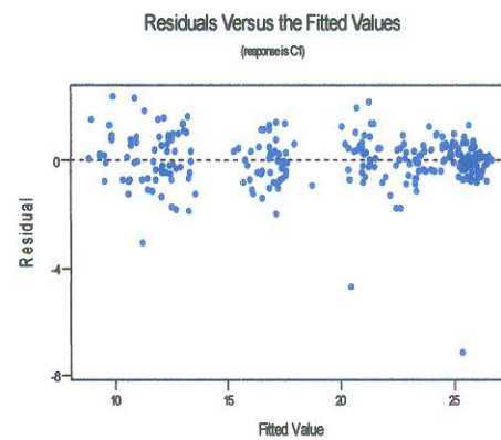
Figure 5.12 Resid. vs the fitted values for AMNT(1981-2004)
