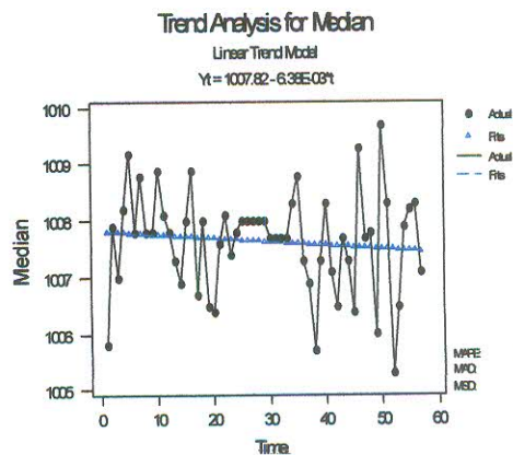
Figure 4.A.36 Trend for median of ASLP
