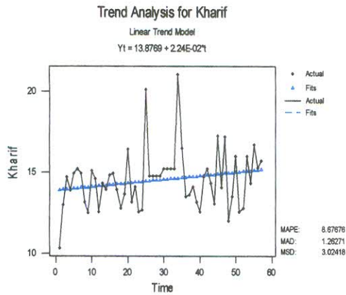
Figure 4.40 Trend of ARH(0-12) in Kharif season
