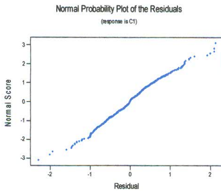
Figure 5.33 Np plot of resid. for AC (1948-2004)
