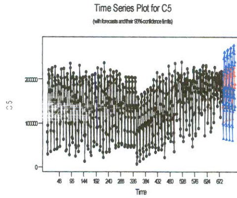
Figure 5.31 48 fore. for ORARH(1948-2004)
