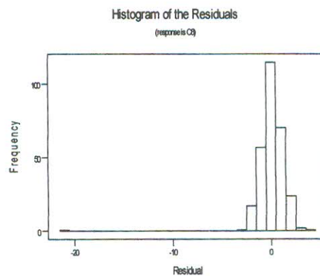
Figure 5.48 Hist. of resid. for ASLP (1948-1972)
