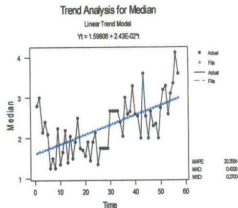
Figure 4.A.32 Trend for median of AC
