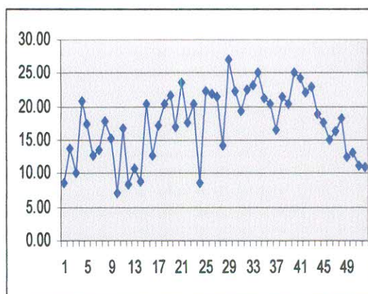
Figure 2.3 Line diagram of WSM for 2005
