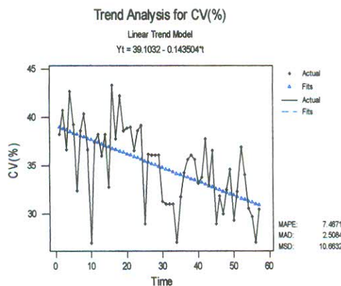
Figure 4.A.19 Trend for CV of ARNT
