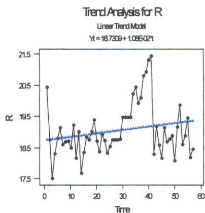
Figure 4.29 Trend of ADBT for Rabi season
