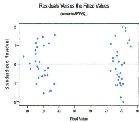
Figure 6.2 SR vs fitted value for original data
