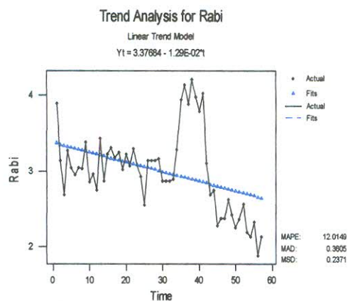
Figure 4.33 Trend of AT (D-W) for Rabi season
