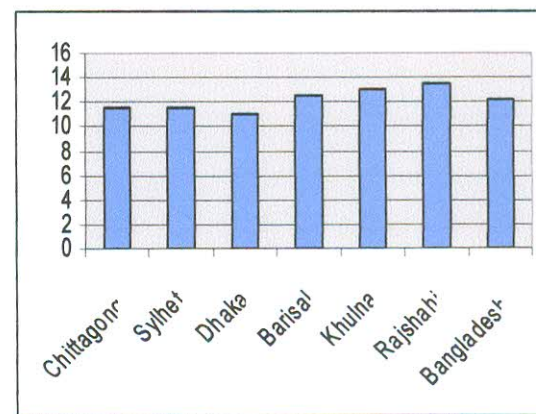
Figure 1.5 ARNT over Bangladesh
