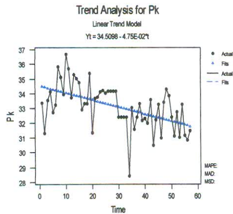
Figure 4.25 Trend of AMXT for Prekharif season
