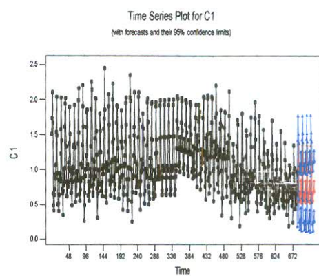
Figure 5.20 48 fore for AT(D-W)(1948-2004)
