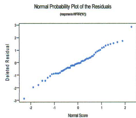
Figure 6.6 Np plot of DR for transformed data
