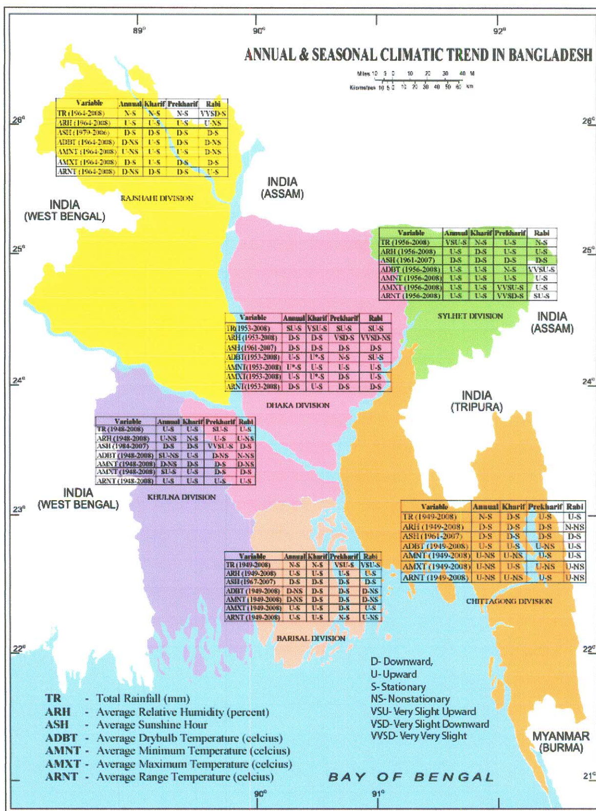
Figure 4.A.53 Annual &amp; Seasonal Climatic Trend in Bangladesh
