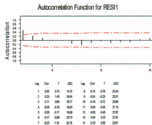
Figure 6.4 ACF plot of SR for original data
