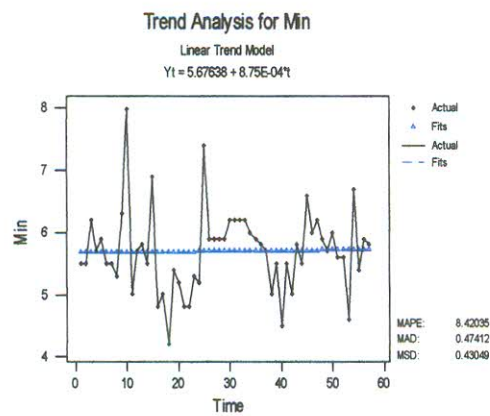
Figure 4.A.3 Trend of minimum for monthly ARNT
