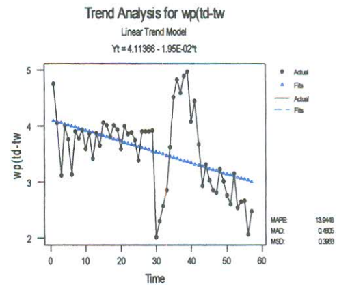
Figure 2.22 TS plot of average AT(D-W) in wp
