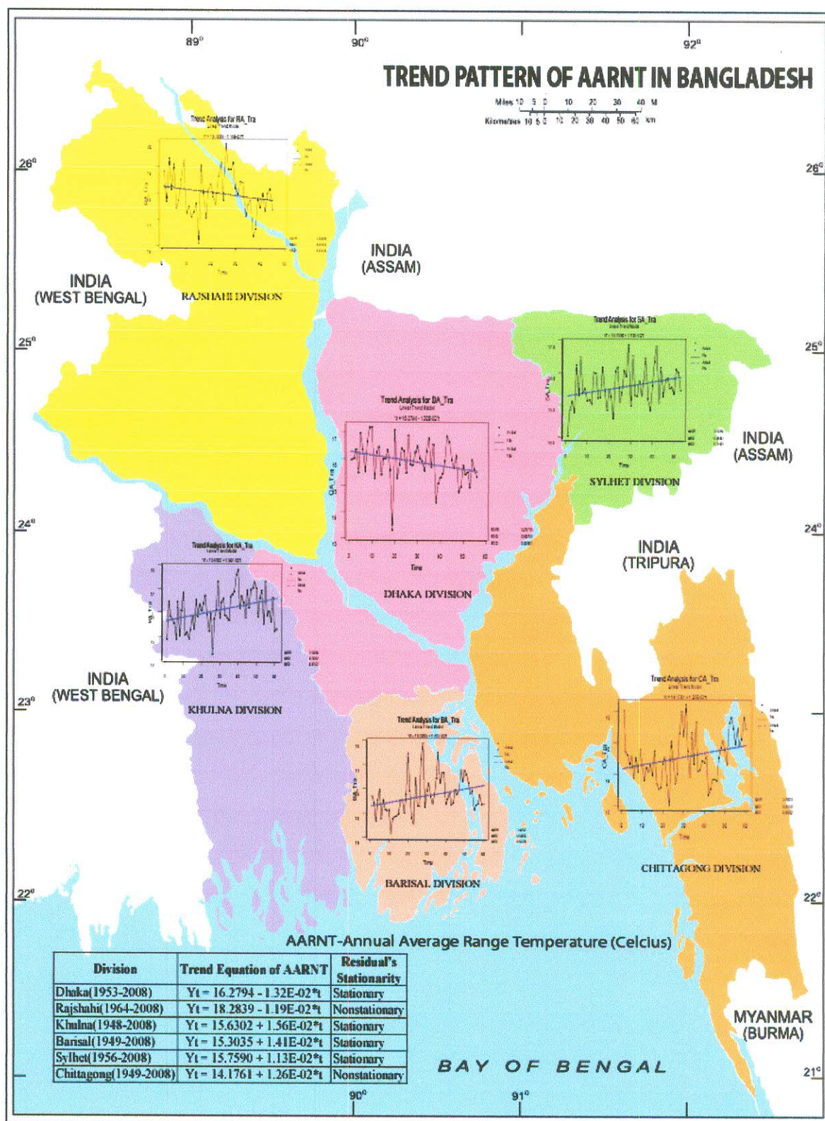
Figure 4. A. 50 Trend Pattern of AARNT in Bangladesh
