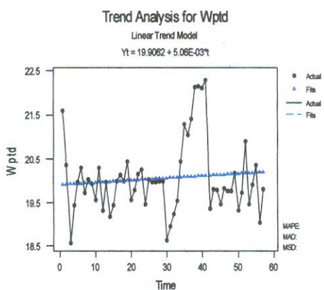
Figure 2.15 TS plot of average ADBT in wp
