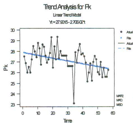
Figure 4.30 Trend of ADBT for Prekharif season
