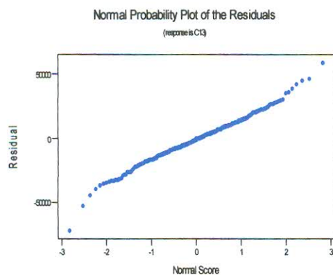
Figure 5.21 Np plot of resid. for ARH (1948-1972)
