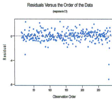
Figure 5.11 Resid. vs order of the data for AMNT (1981-2004)
