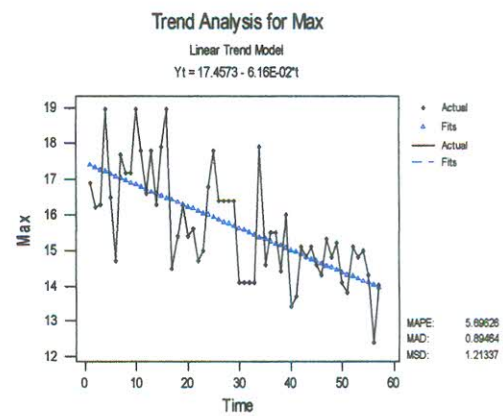
Figure 4.A.4 Trend of maximum for monthly ARNT
