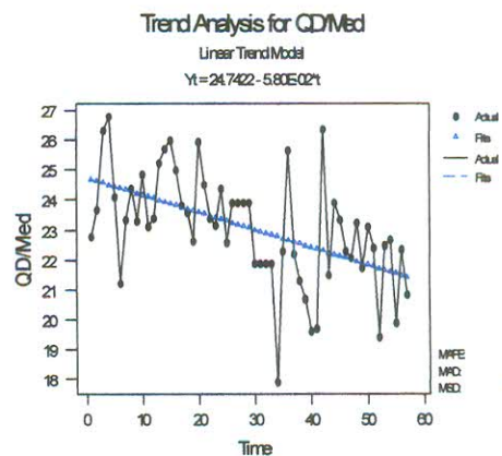
Figure 4.A.20 Trend for QD/Med of AWBT
