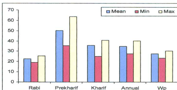
Figure 2.11 Bar Diagram of Evaporation for Seasonal, Annual and WP
