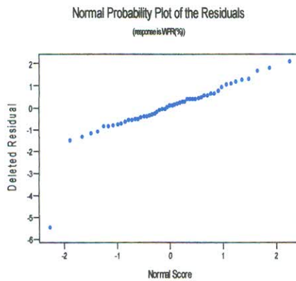
Figure 5.55 NP plot for resid. of LT model
