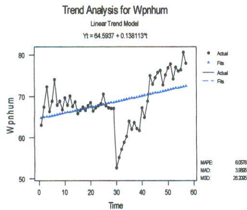
Figure 2.23 TS plot of average ARH in wp
