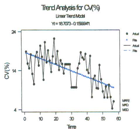
Figure 4.A.25 Trend for CV of ARH
