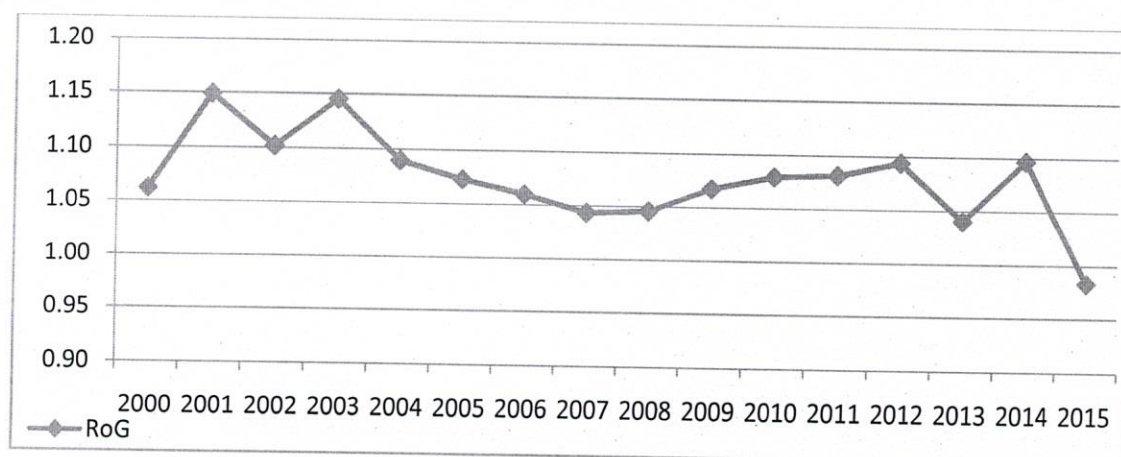
Figure 4.3: Rate of Growth (RoG) of PH literature
