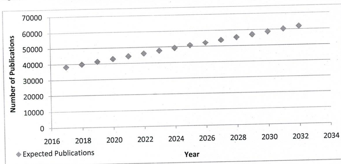
Figure 4.7: Forecasting of growth of PH literature
