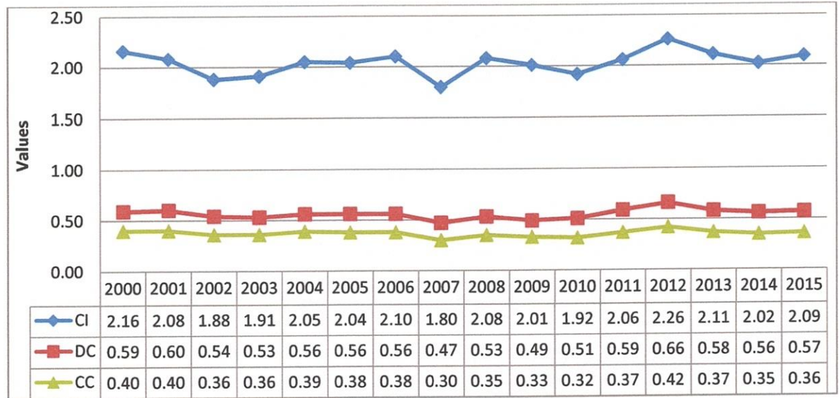
Figure 4.15: CI, DC and CC: comparative analysis
