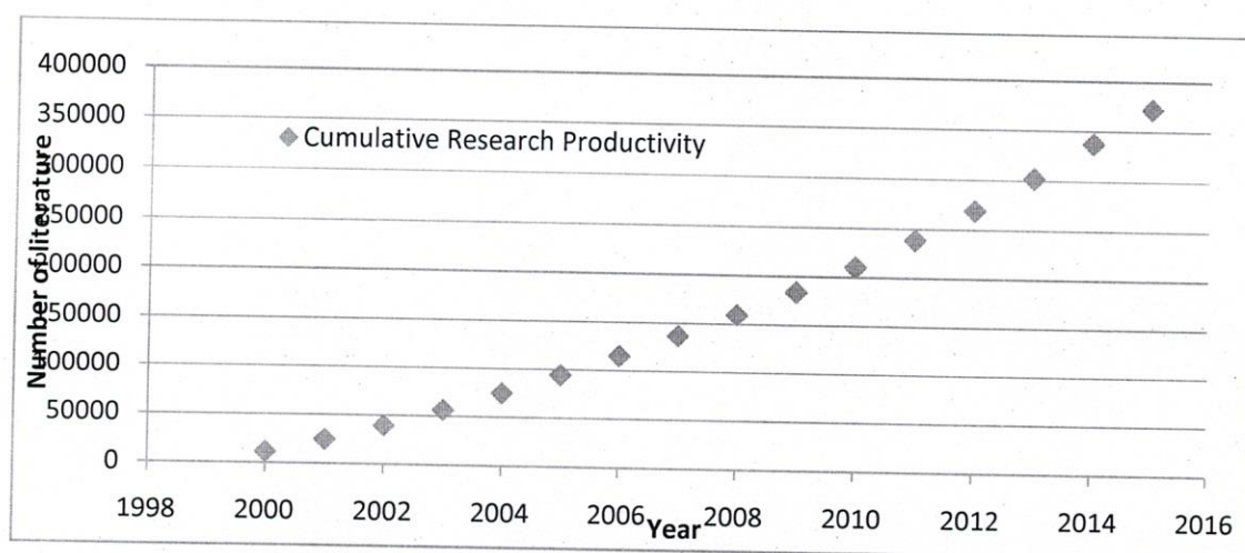
Figure 4.2: Cumulative growth of literature
