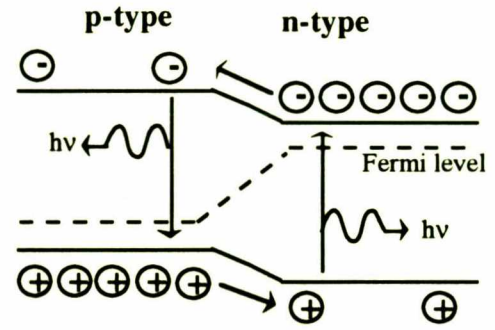
Figure 3.3 Radiative recombination in a p-n junction
