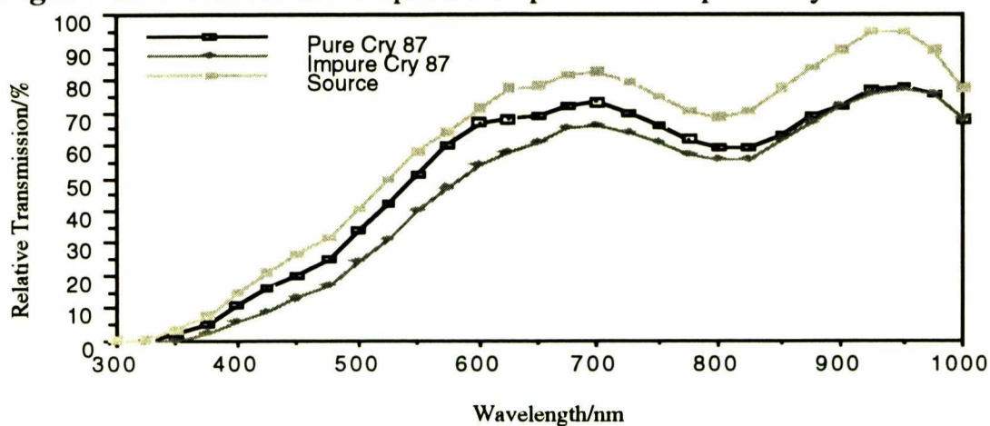
Figure 8.3c Transmission spectra of pure and impure Crylin 87.
