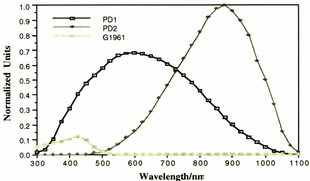
Figure 4.5 Spectral responses of PD1, PD2, G1961 photodiode triplet (Henderson 1990).
