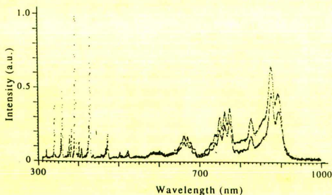
Figure 5. Emission spectra of pure nitrogen at 20 W (lower trace) and 40 W (upper trace).
