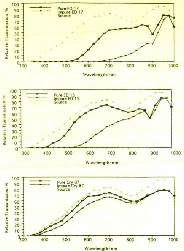
Figure 3. Transmission spectra for pure and impure oils.
