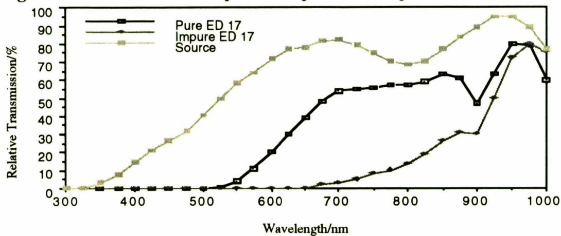
Figure 8.3a Transmission spectra of pure and impure Edwards 17.
