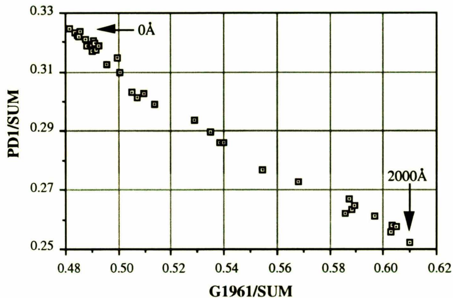
Figure 7.5 Film thickness plotted on a chromatic plane.
