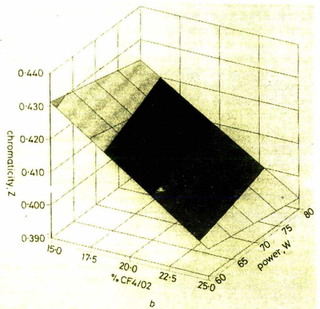
Fig. 6 Use of chromaticity in plasma control
