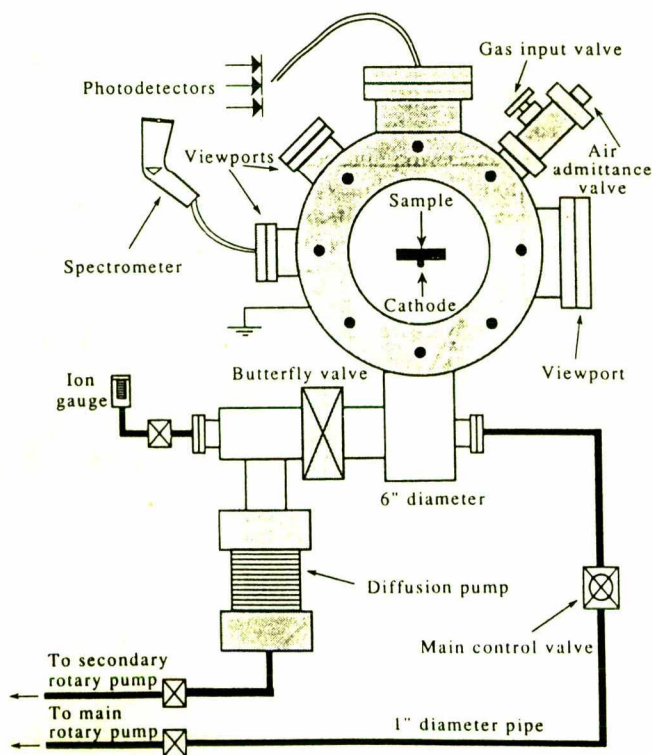
Figure 2. Schematic of dc plasma chamber.
