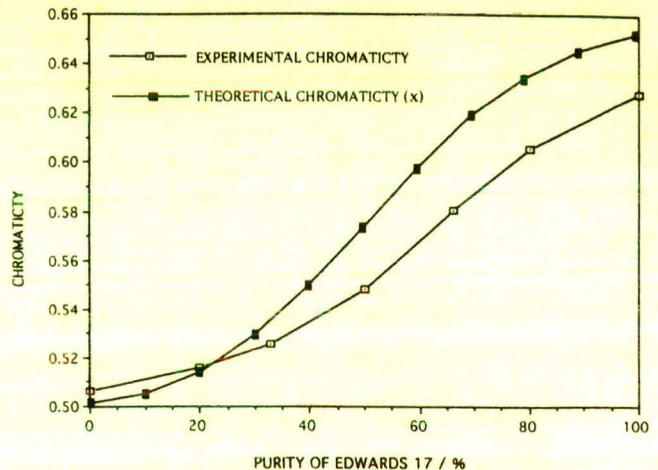
Figure 6. Chromaticity of Edwards 17 as a function of purity.
