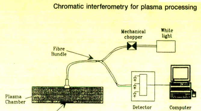
Figure 5. The experimental system used for monitoring film thickness online.
