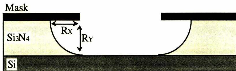
Figure 2.1b Mask undercut due to isotropic etching.
