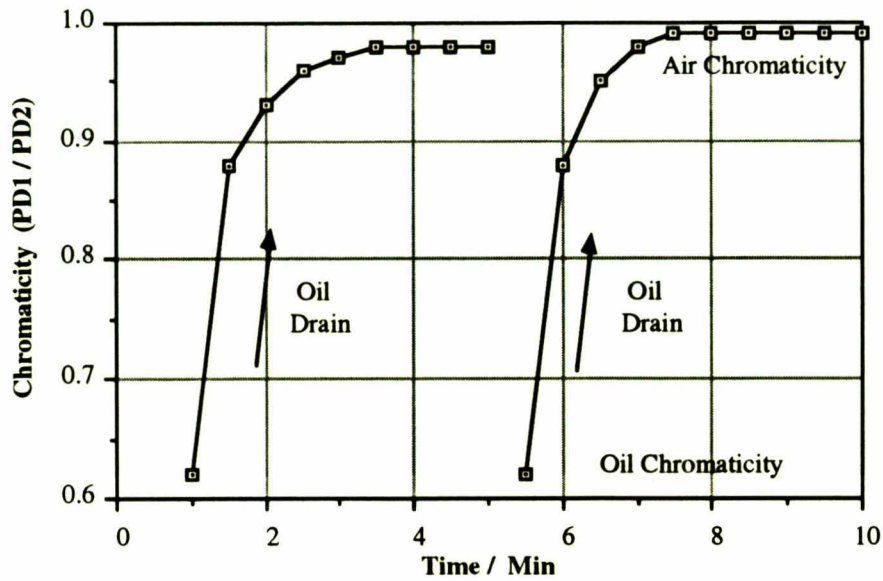
Figure 8.7 The repeatability of air and oil chromaticities.
