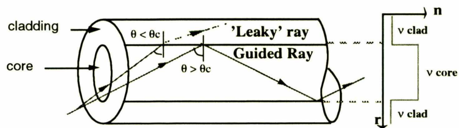
Figure 3.6: Confinement of light in a fibre according to ray theory.
