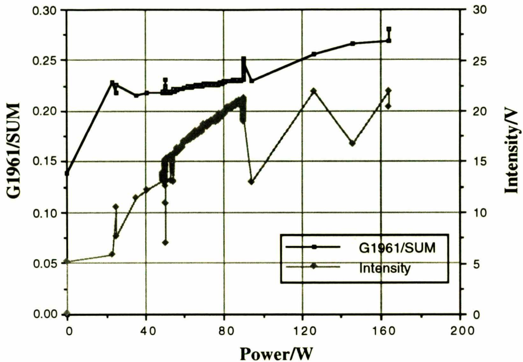
Figure 6.5 The change in chromaticity as a function of increasing power with the change in plasma intensity for comparison.
