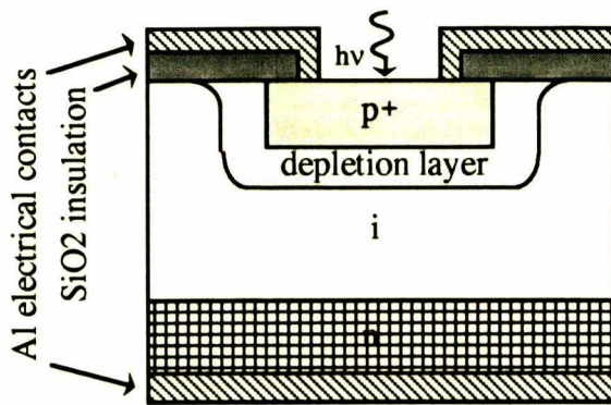
Figure 3.4 Construction of a p-i-n silicon photodiode
