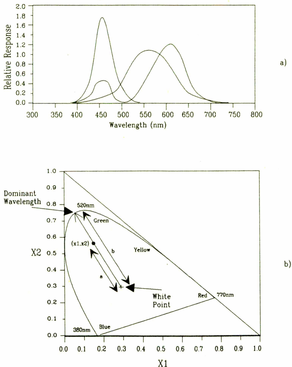
Figure 3. The three detector responses shown in (a) produce the chromaticity diagram shown in (b). Using these detectors, white light has coordinates (0.3,0.3) as indicated in (b). A coloured source may have coordinates ( x_1, x_2 ). The dominant wavelength of this source is shown in (b). The saturation of the source is calculated from the ratio of the lengths a/b .
