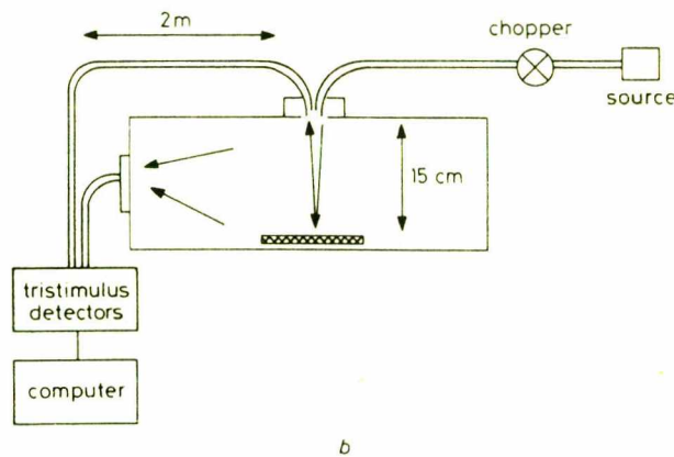
Fig. 1 Tristimulus systems
