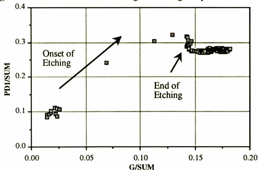
Figure 6.10 Chromatic changes during a plasma etch process
