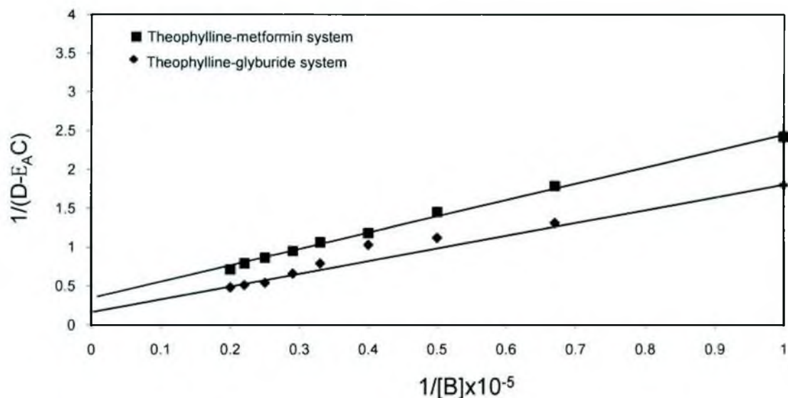
Fig. 7.1.6.18: Ardon's plot for complexation of theophylline with glyburide and metformin at pH 2.4
