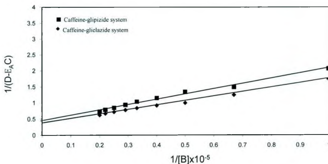
Fig.7.1.6.3: Ardon's plot for complexation of caffeine with gliclazide and glipizide at pH 2.4
