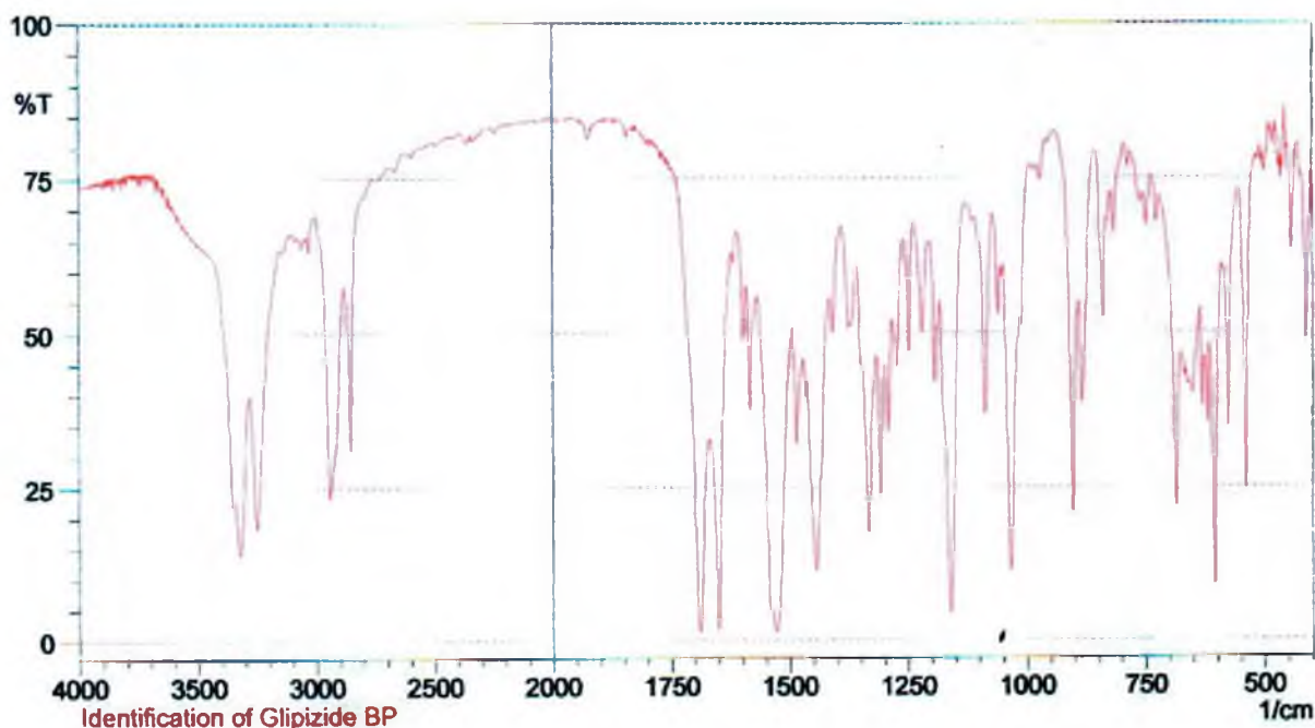
Fig. 4.2.1: IR spectrum for working standard of glipizide
