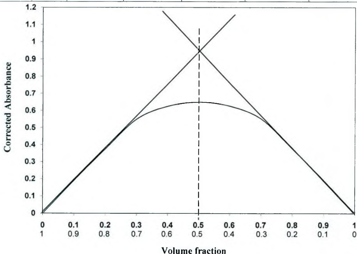
Fig. 7.1.3.1: Continuous-variation plot for Caffeine-Gliclazide system
