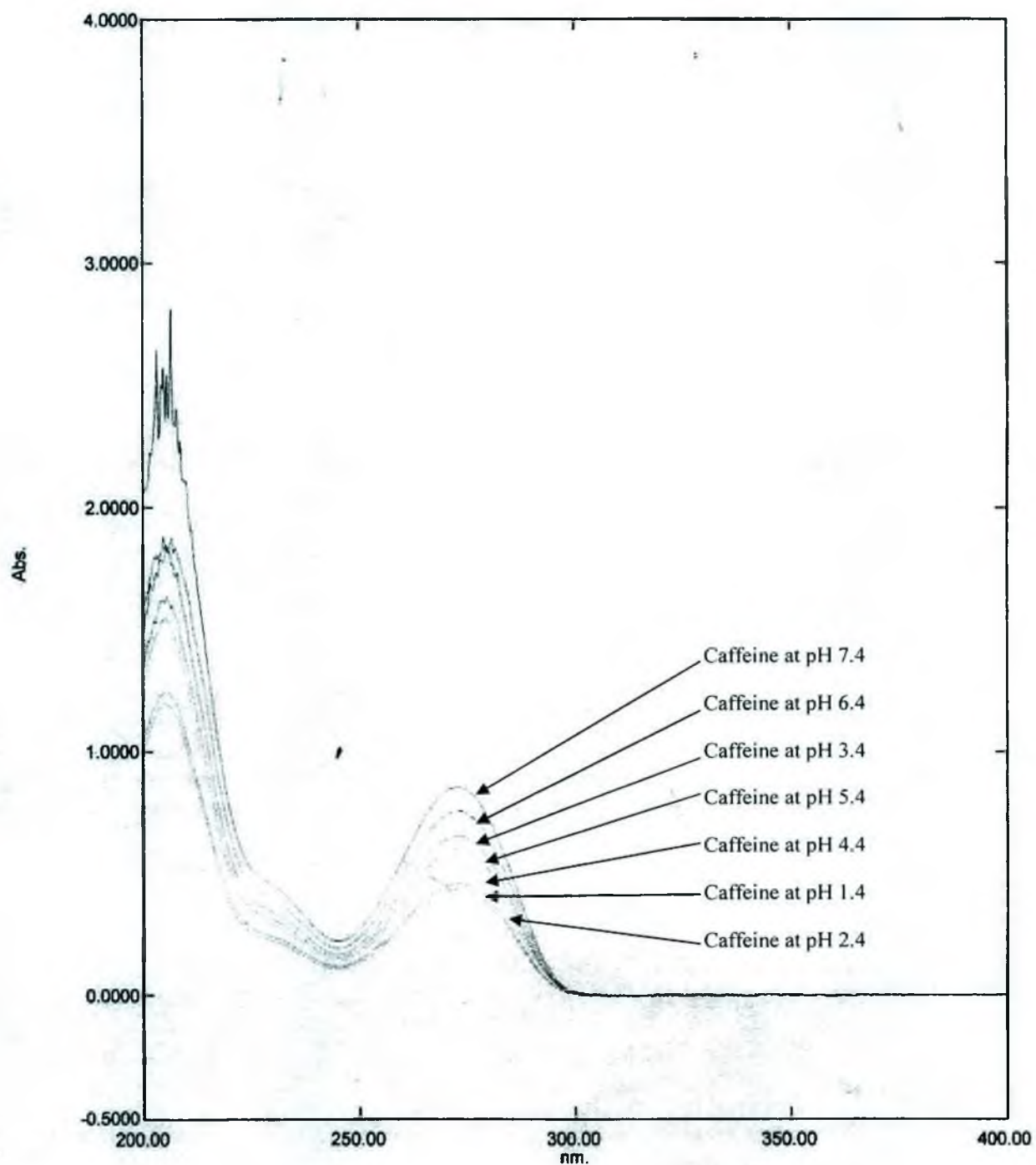
Fig. 7.1.2.1: UV spectra of Caffeine at different p^H (Conc. of Caffeine = 0.0001 M)
