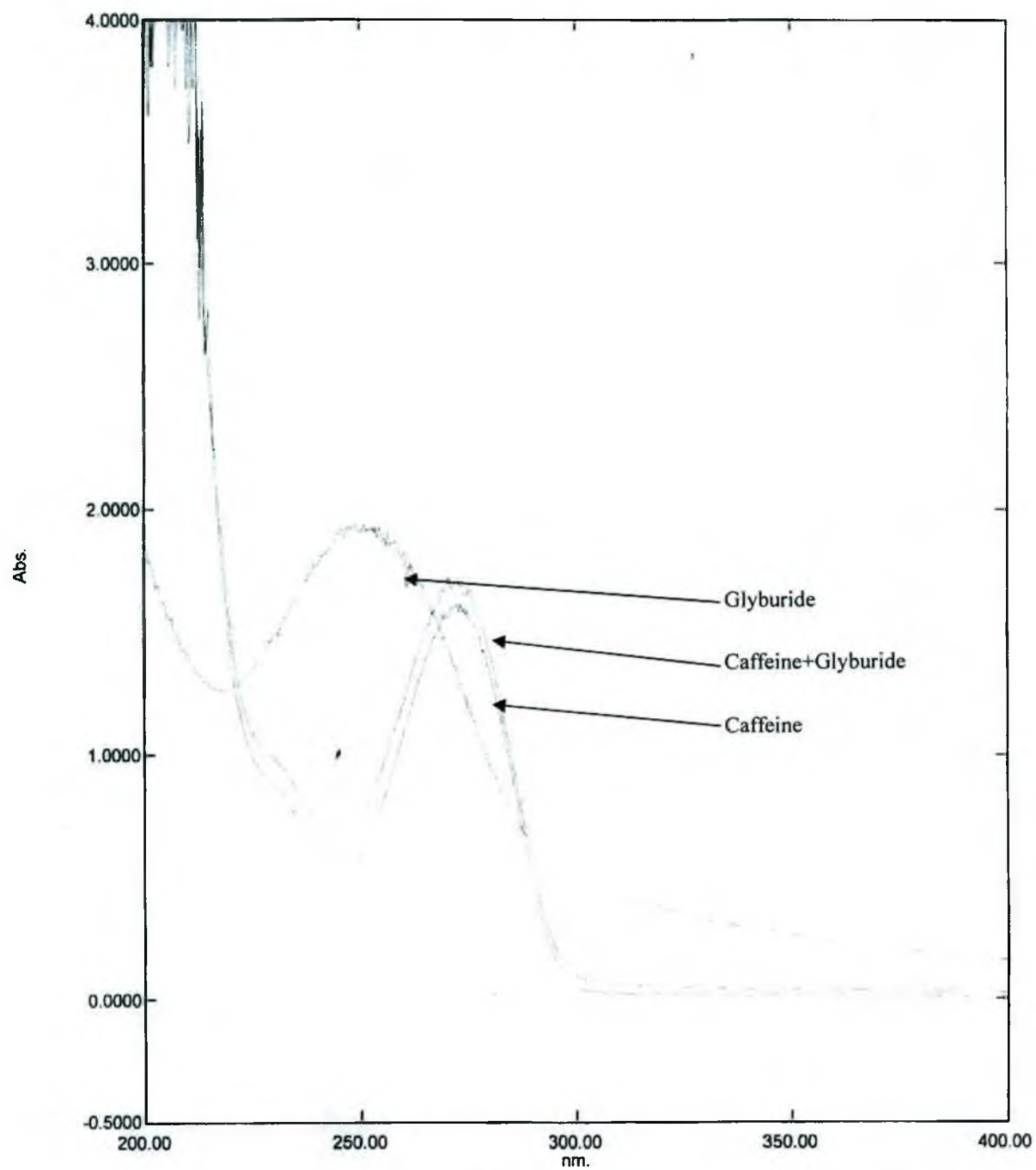
Fig.7.1.2.16: UV spectra of Caffeine – Glyburide systems at pH 4.4 (Conc. of Caffeine = Conc. of Glyburide = 0.0001 M)
