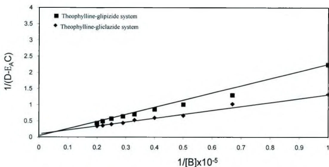
Fig. 7.1.6.21: Ardon's plot for complexation of theophylline with gliclazide and glipizide at pH 4.4
