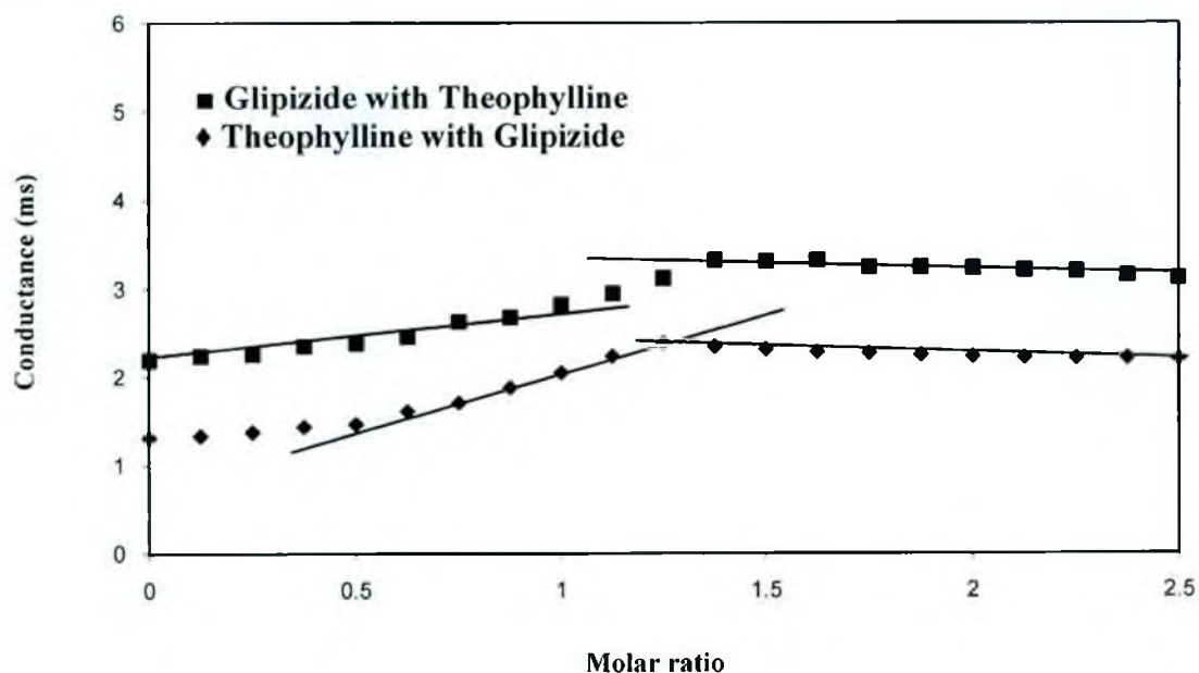
Fig. 7.1.5.34: Conductometric titration of theophylline with glipizide and glipizide with theophylline at pH 2.4
