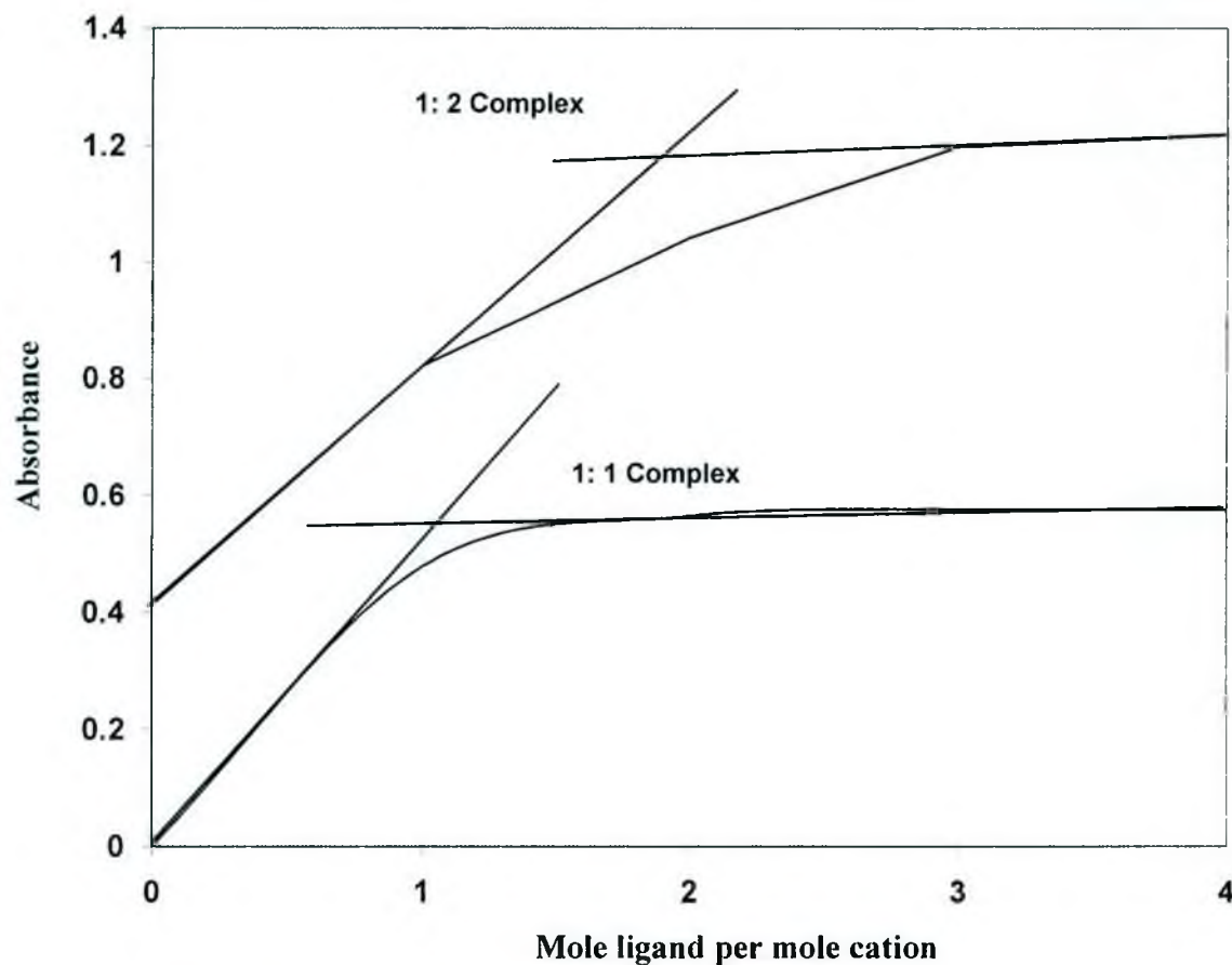
Fig. 7.1.4.8: Mole-ratio plot for theophylline-metformin system
