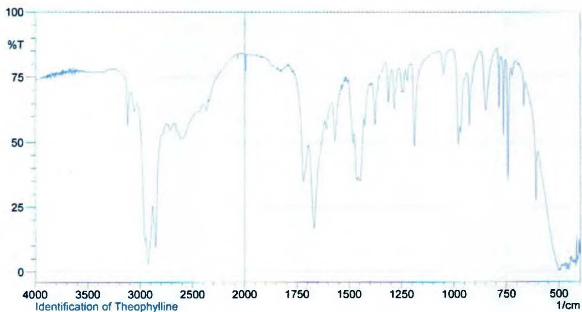
Fig. 4.6.2: IR spectrum for sample of theophylline
