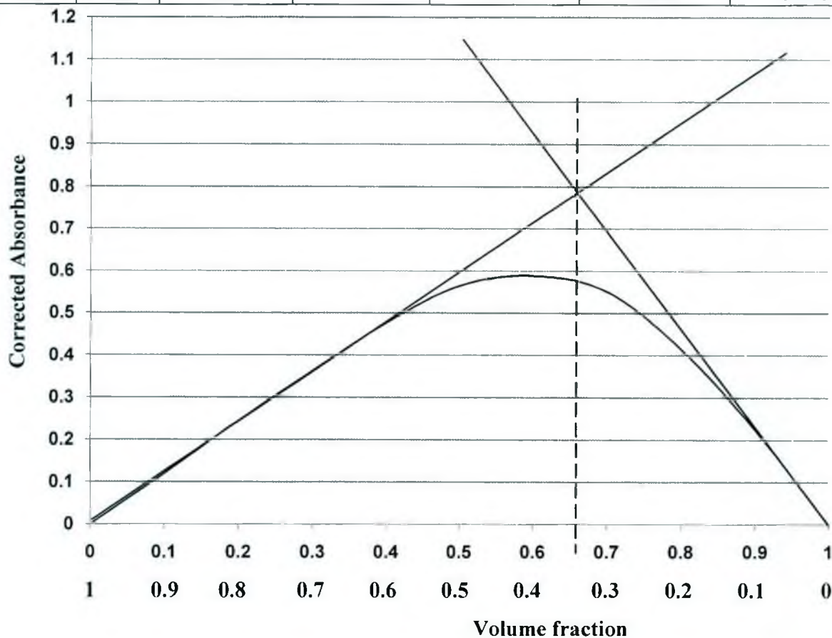
Fig. 7.1.3.6: Continuous-variation plot for Theophylline-Glipizide system
