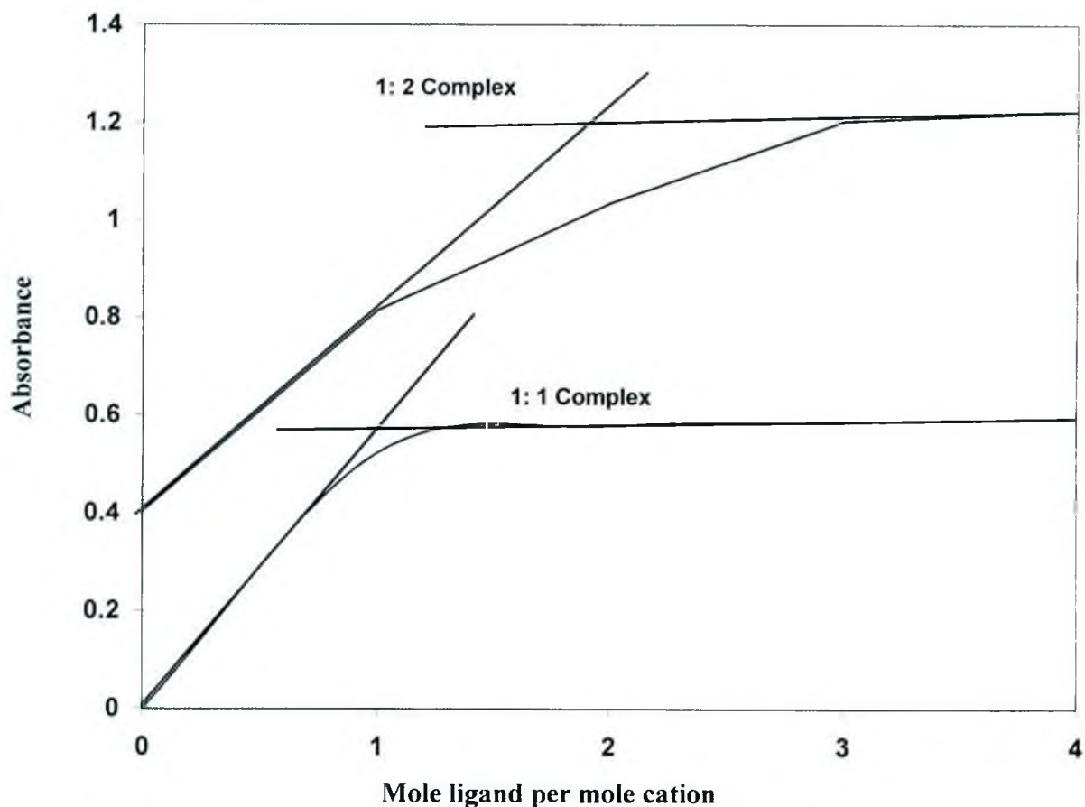
Fig. 7.1.4.4: Mole-ratio plot for caffeine-metformin system
