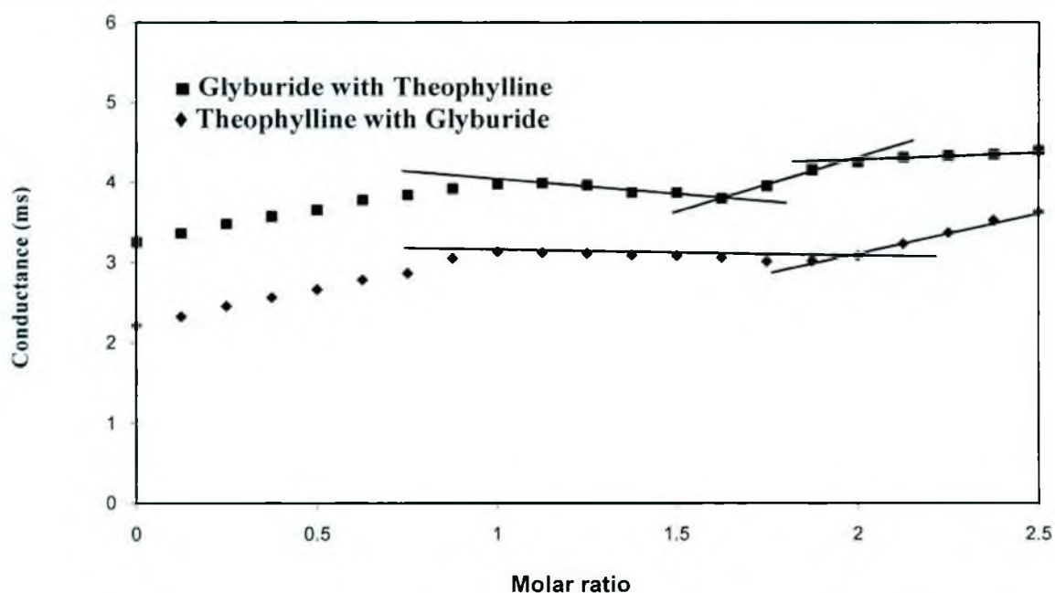
Fig. 7.1.5.47: Conductometric titration of theophylline with glyburide and glyburide with theophylline at pH 5.4
