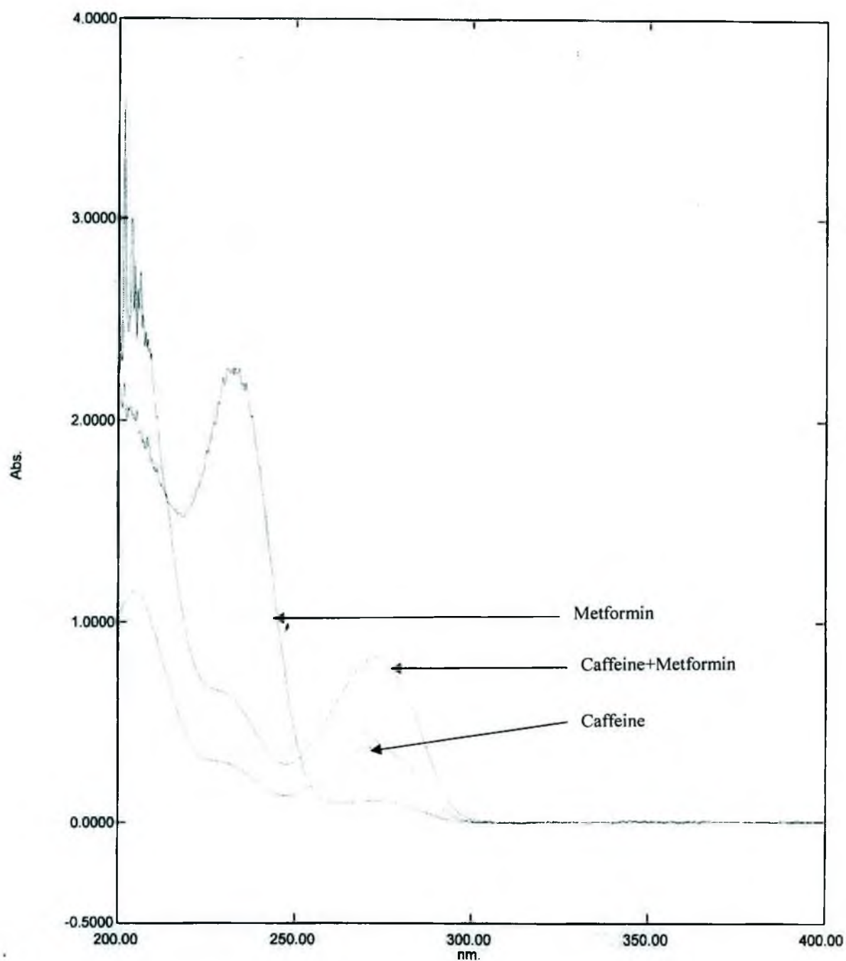
Fig.7.1.2.13: UV spectra of Caffeine – Metformin systems at pH 3.4 (Conc. of Caffeine = Conc. of Metformin = 0.0001 M)
