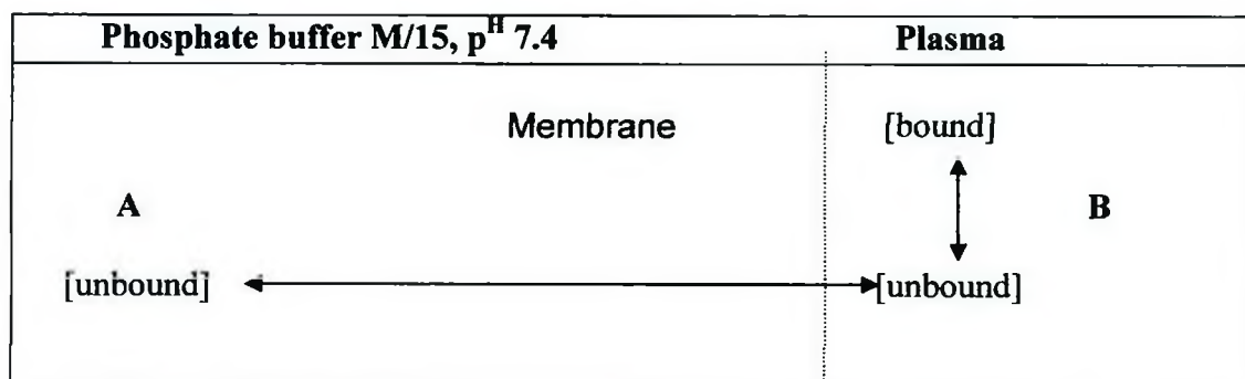
Fig 6.2.1: The equilibrium dialysis process
