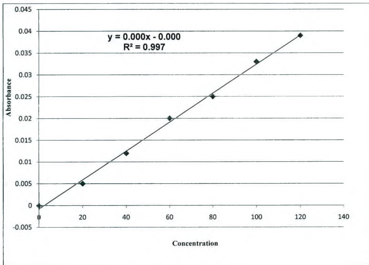
Fig. 6.3.3: Calibration curve for glyburide for determination of plasma concentration
