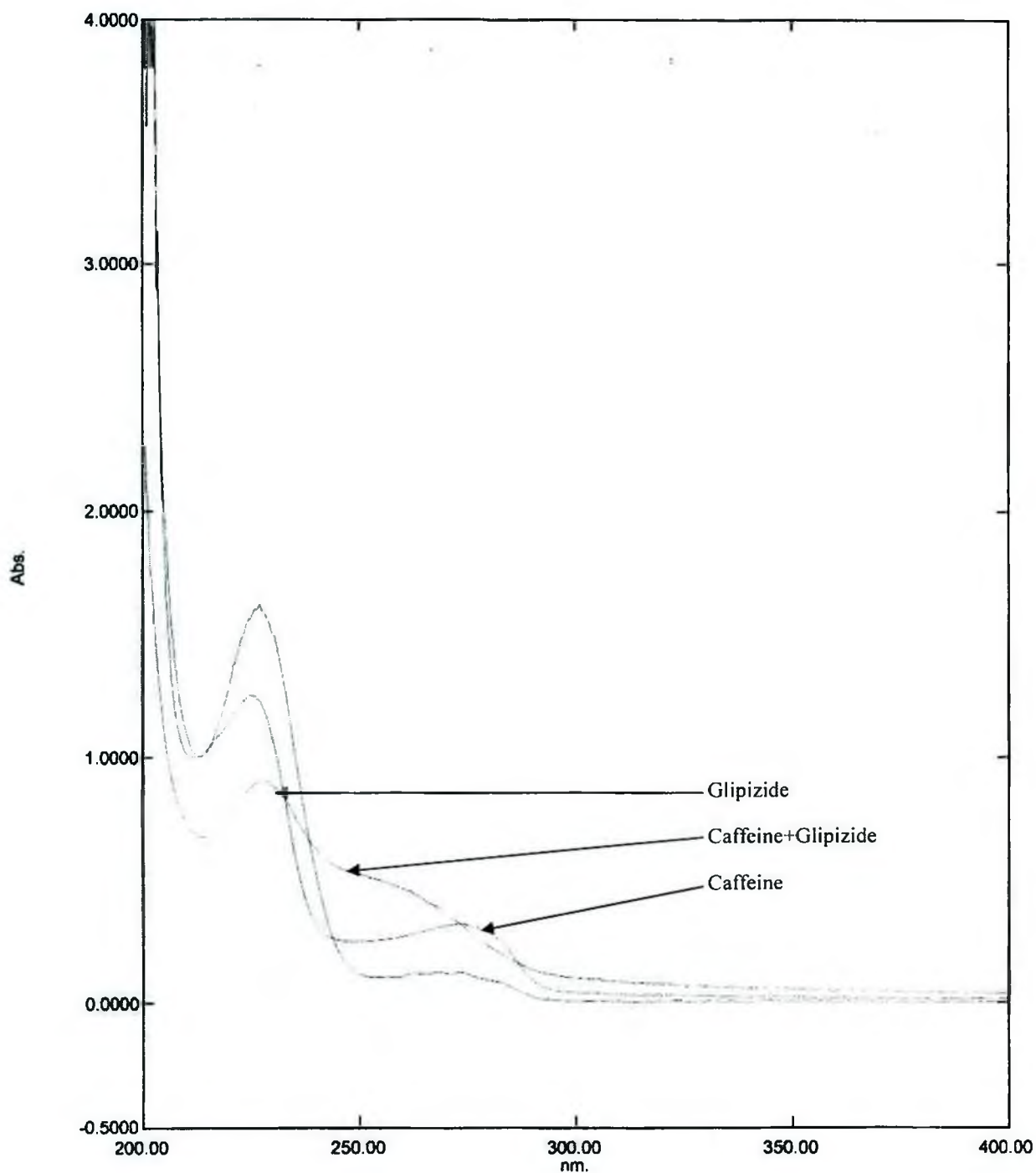
Fig.7.1.2.7: UV spectra of Caffeine – Glipizide systems at pH 2.4 (Conc. of Caffeine = Conc. of Glipizide = 0.0001 M)
