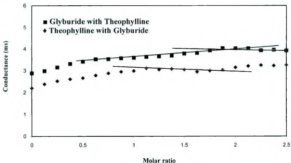
Fig. 7.1.5.31: Conductometric titration of theophylline with glyburide and glyburide with theophylline at pH 1.4
