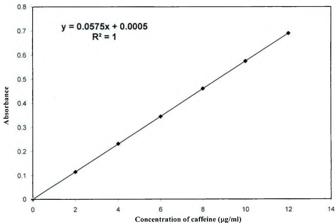
Fig. 4.5.5: Standard curve for caffeine
