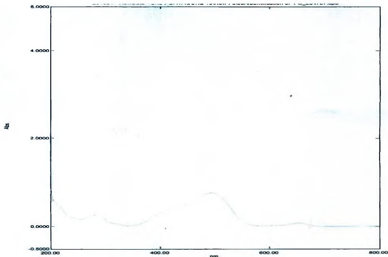
Fig. 4.7.1: UV – VIS spectrum for glucose solution
