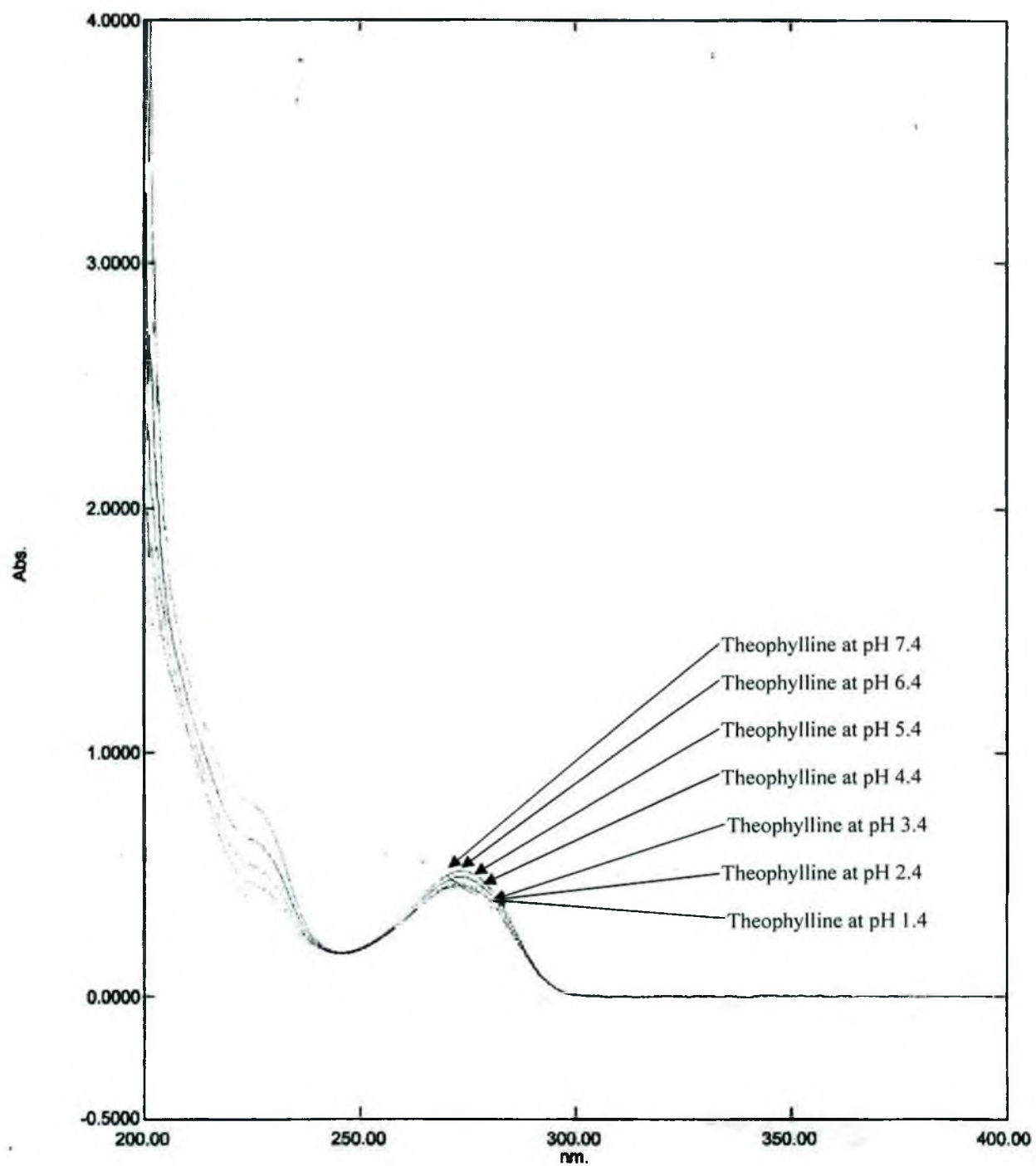
Fig.7.1.2.30: UV spectra of Theophylline at different p^H (Conc. of theophylline = 0.0001 M)
