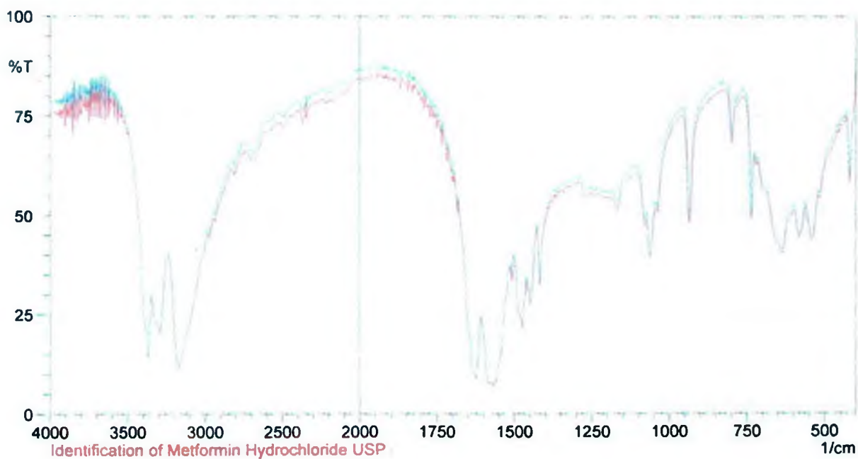
Fig.4.4.3: Joined visible IR spectrum for working standard & sample of metformin
