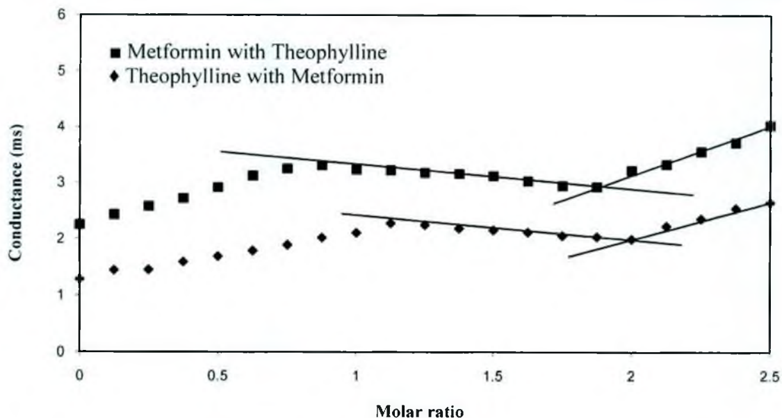
Fig. 7.1.5.56: Conductometric titration of theophylline with metformin and metformin with theophylline at pH 7.4
