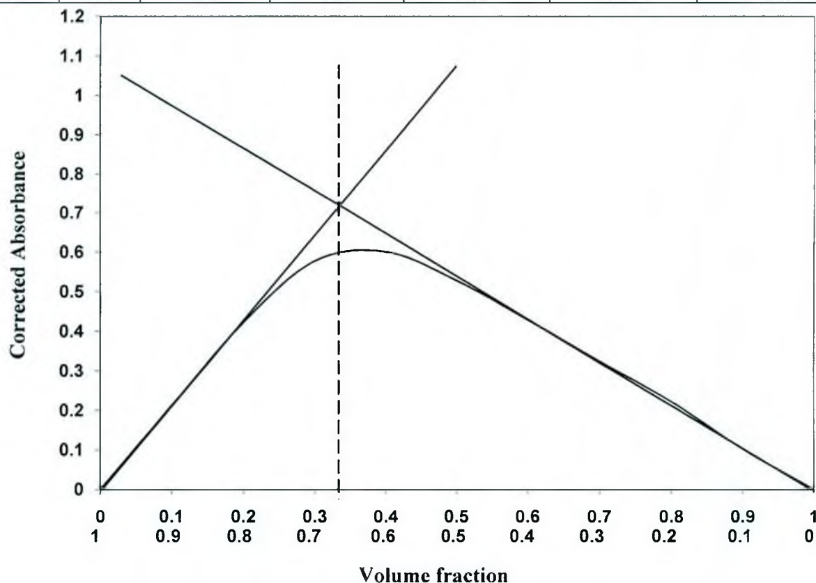
Fig. 7.1.3.3: Continuous-variation plot for Caffeine-Glyburide system
