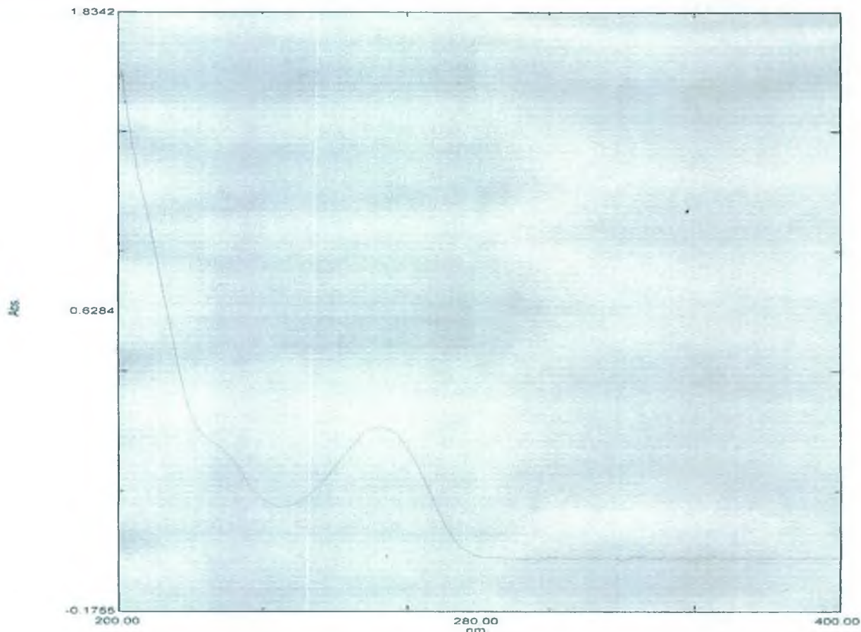
Fig.4.6.4: UV – VIS spectrum for working standard of theophylline
