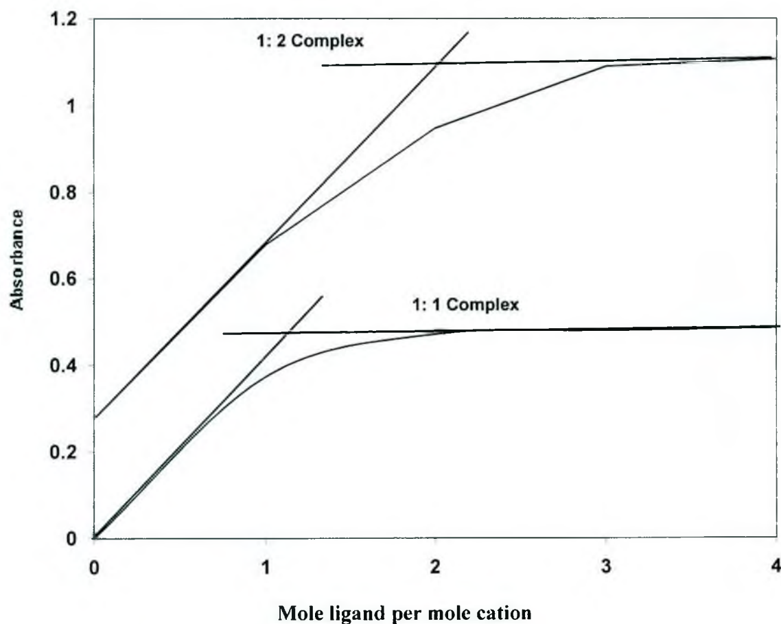
Fig. 7.1.4.7: Mole-ratio plot for theophylline-glyburide system
