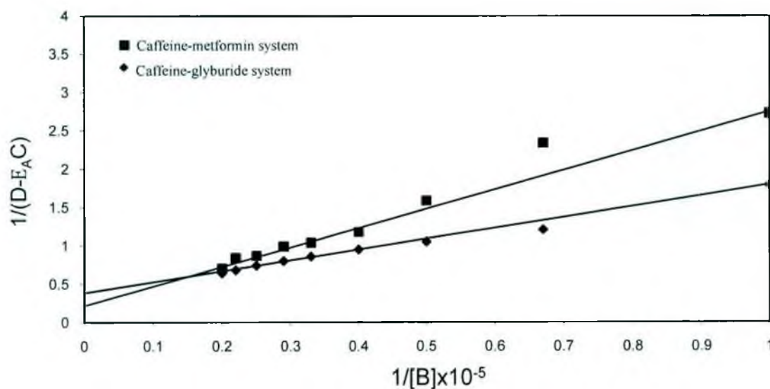
Fig.7.1.6.2: Ardon's plot for complexation of caffeine with glyburide and Metformin at pH 1.4
