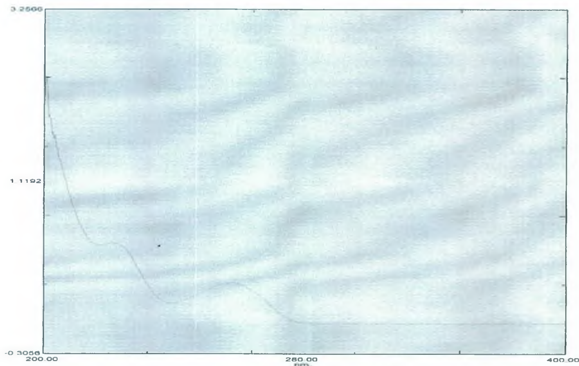
Fig.4.1.4: UV – VIS spectrum for working standard of gliclazide
