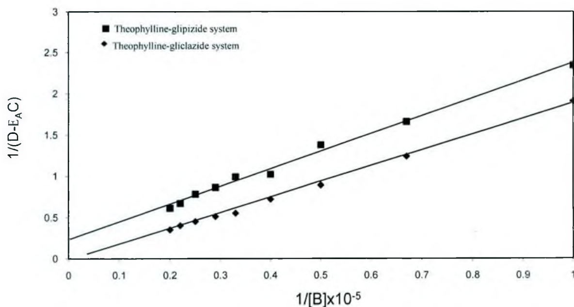
Fig. 7.1.6.27: Ardon's plot for complexation of theophylline with gliclazide and glipizide at pH 7.4
