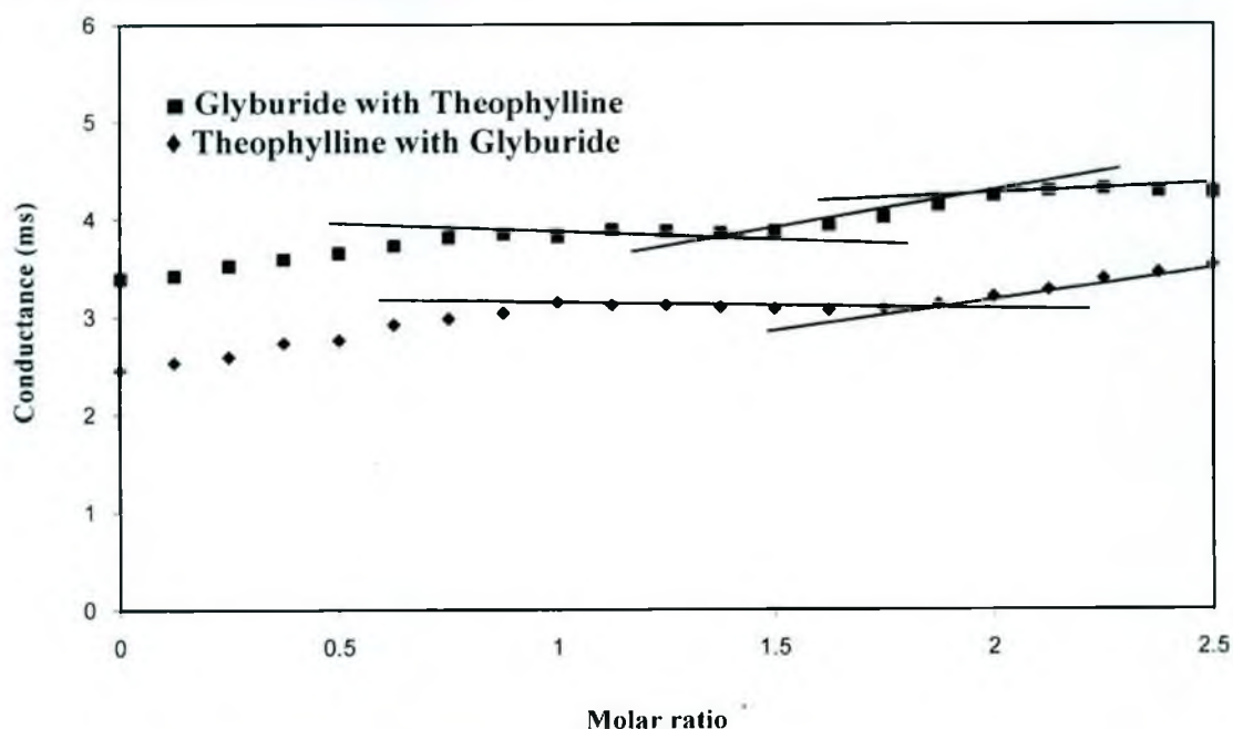
Fig. 7.1.5.51: Conductometric titration of theophylline with glyburide and glyburide with theophylline at pH 6.4
