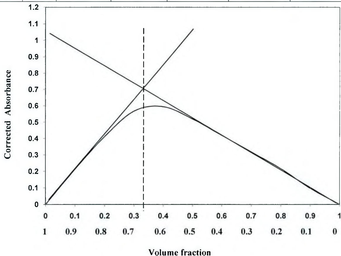
Fig. 7.1.3.7: Continuous-variation plot for Theophylline-Glyburide system
