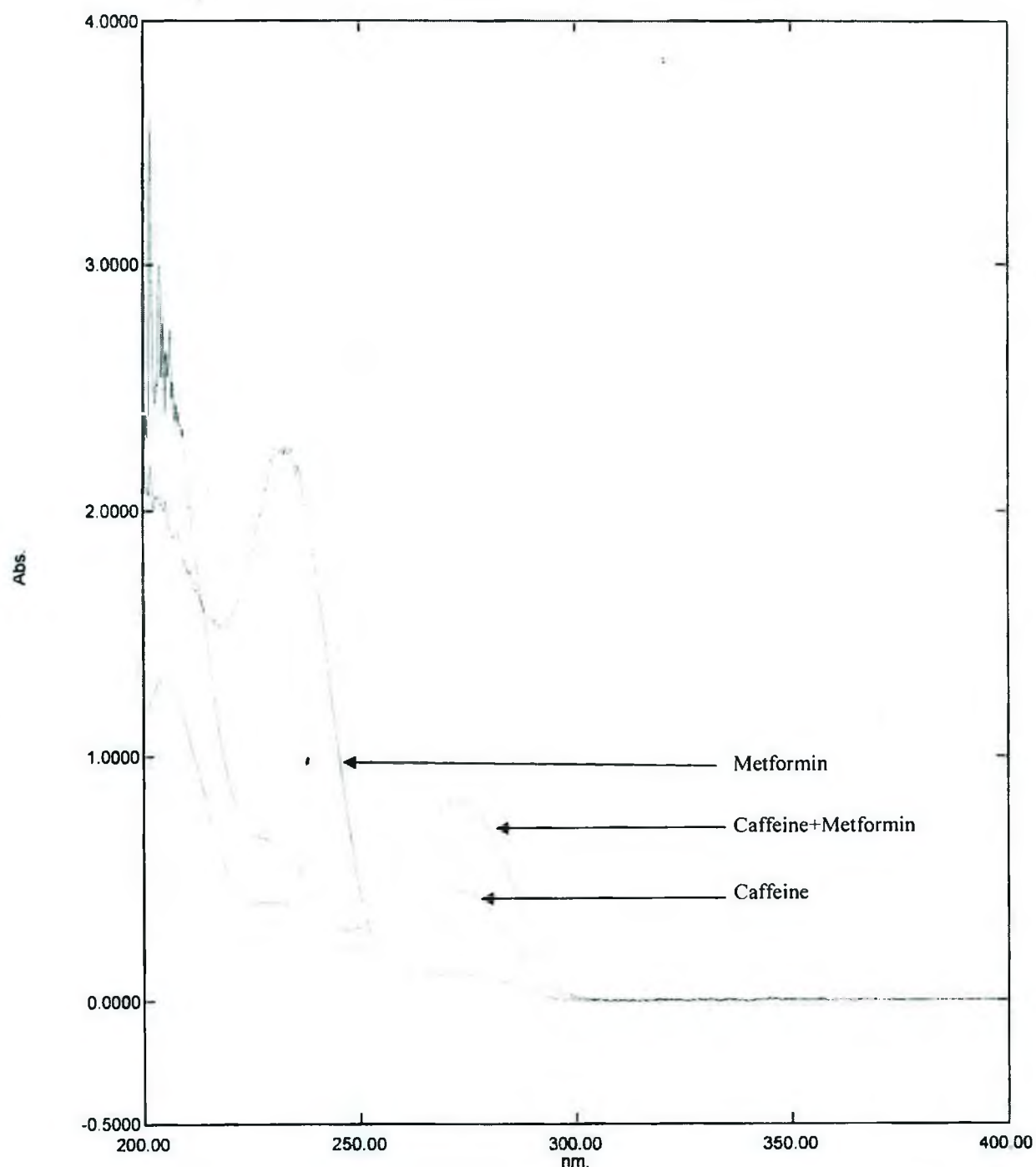
Fig.7.1.2.17: UV spectra of Caffeine – Metformin systems at pH 4.4 (Conc. of Caffeine = Conc. of Metformin = 0.0001 M)
