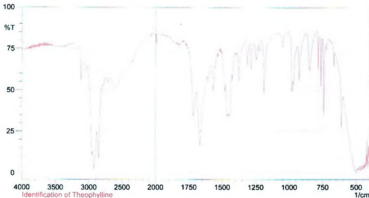
Fig. 4.6.1: IR spectrum for working standard of theophylline
