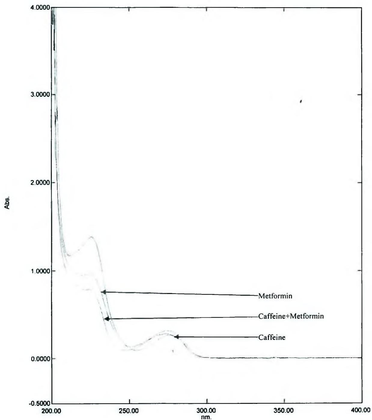
Fig.7.1.2.5: UV spectra of Caffeine – Metformin systems at pH 1.4 (Conc. of Caffeine = Conc. of Metformin = 0.0001 M)
