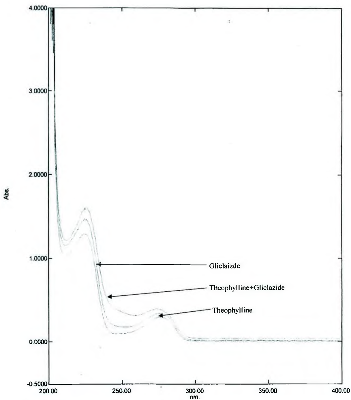
Fig.7.1.2.39: UV spectra of Theophylline – Gliclazide systems at pH 3.4 (Conc. of Theophylline = Conc. of Gliclazide = 0.0001 M)
