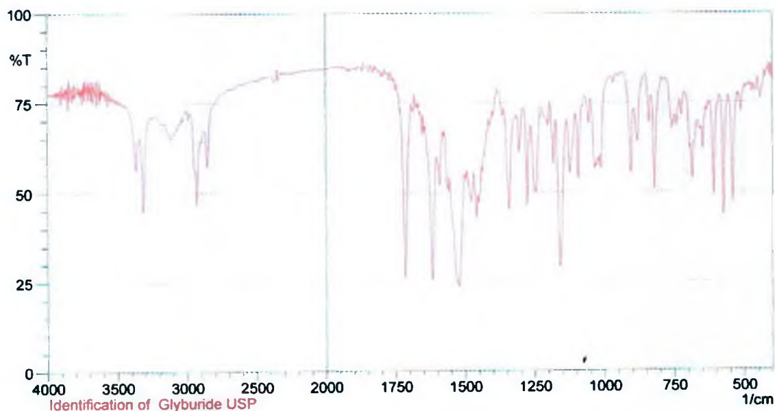
Fig. 4.3.1: IR spectrum for working standard of glyburide
