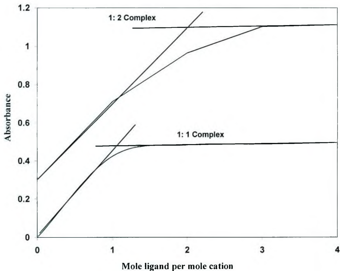
Fig. 7.1.4.1: Mole-ratio plot for caffeine-gliclazide system
