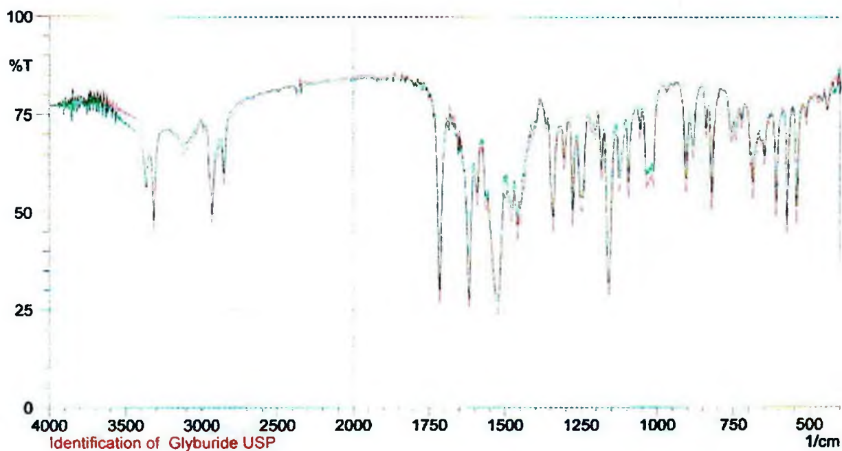
Fig. 4.3.2: IR spectrum for sample of glyburide
