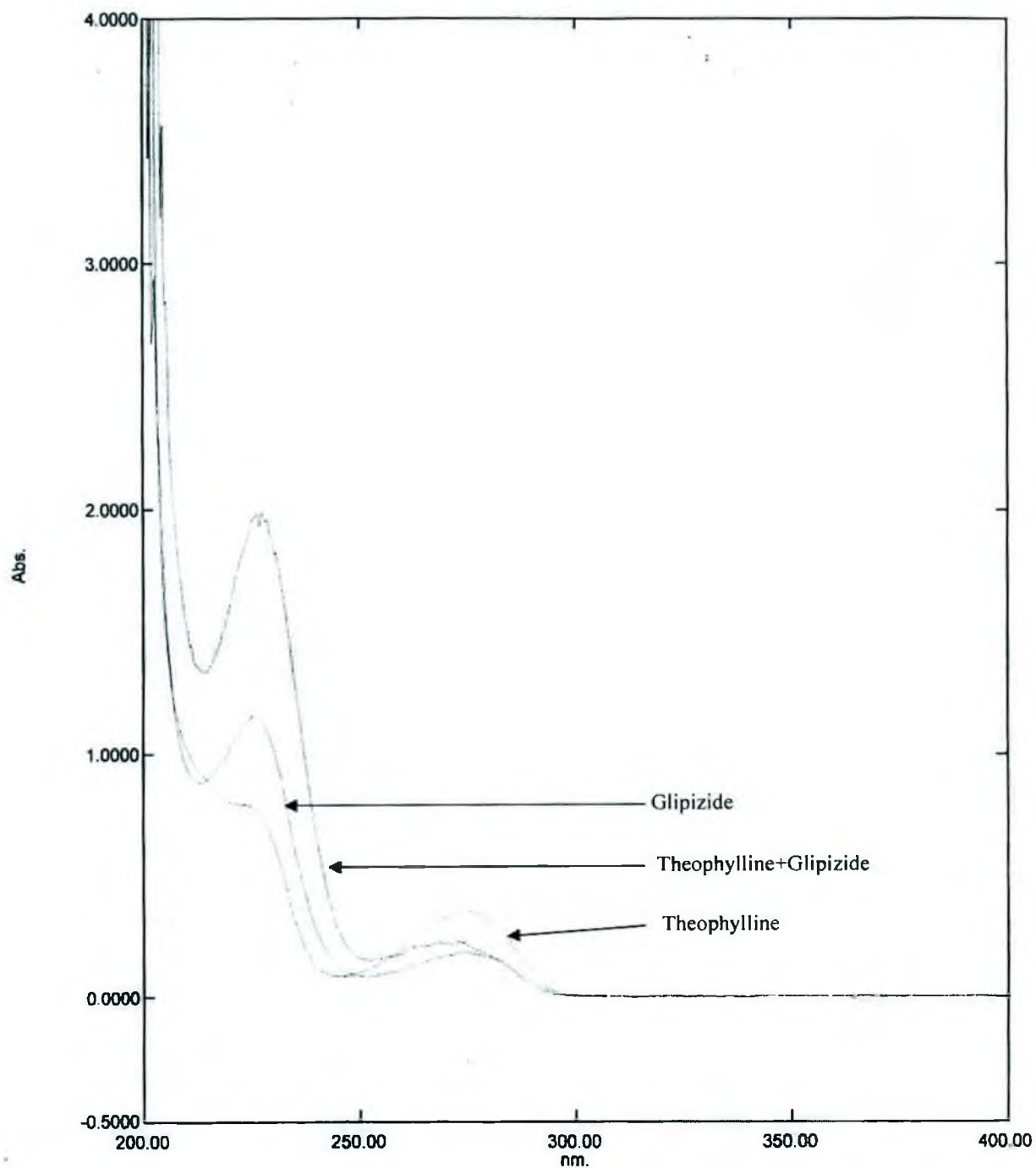
Fig.7.1.2.48: UV spectra of Theophylline – Glipizide systems at pH 5.4 (Conc. of Theophylline = Conc. of Glipizide = 0.0001 M)
