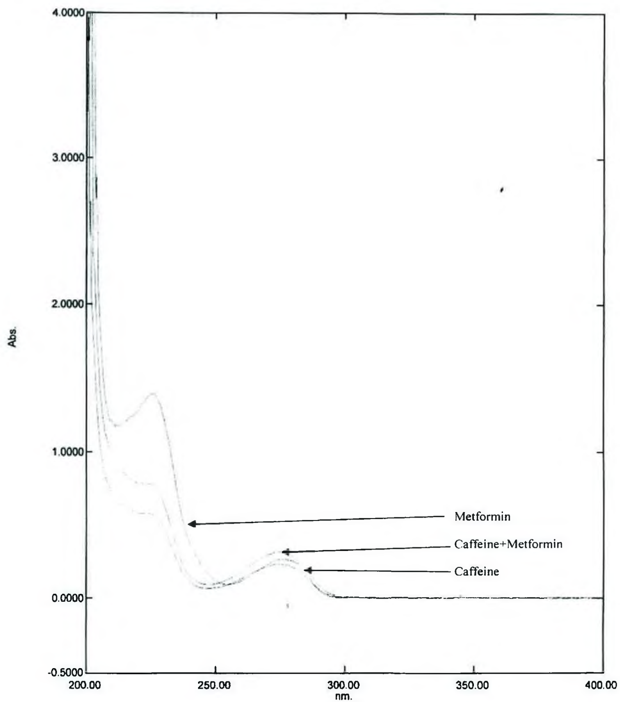
Fig.7.1.2.9: UV spectra of Caffeine – Metformin systems at pH 2.4 (Conc. of Caffeine = Conc. of Metformin = 0.0001 M)
