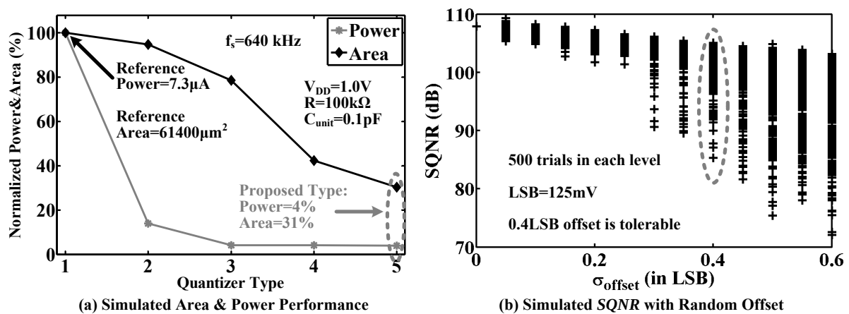
Figure 12. (a) Simulated area and power performance of the introduced five nine-level quantizers; (b) Simulated signal-to-quantization noise ratio ( SQNR ) with random comparator offset, where there are 500 trials at each level.
