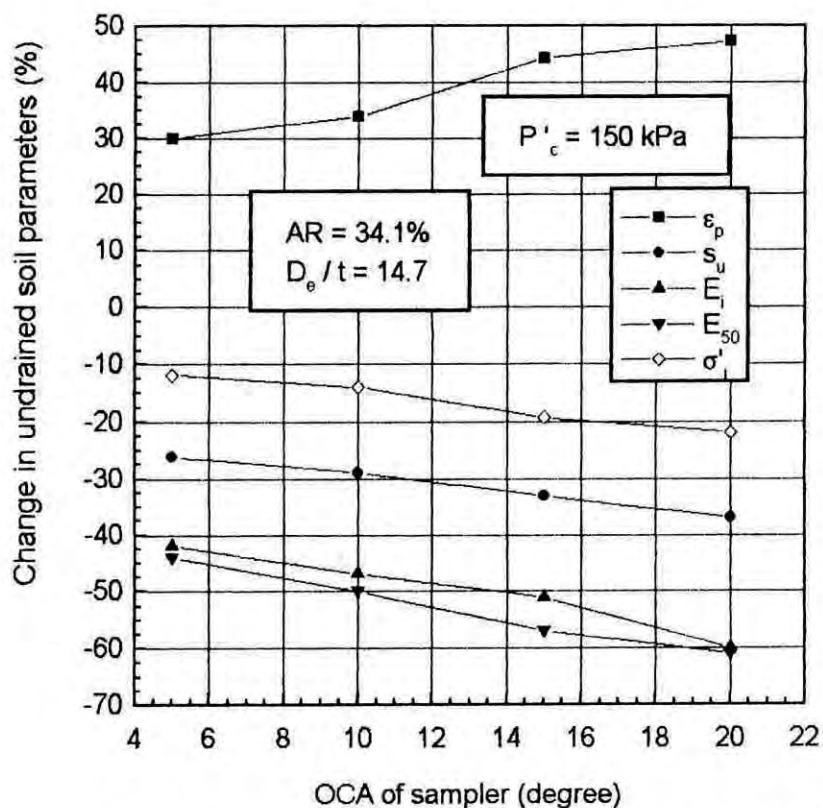
Fig.5.33 Influence of OCA of samplers (degree) on undrained soil parameters for samples of Dhaka Clay for OCR = 1.
