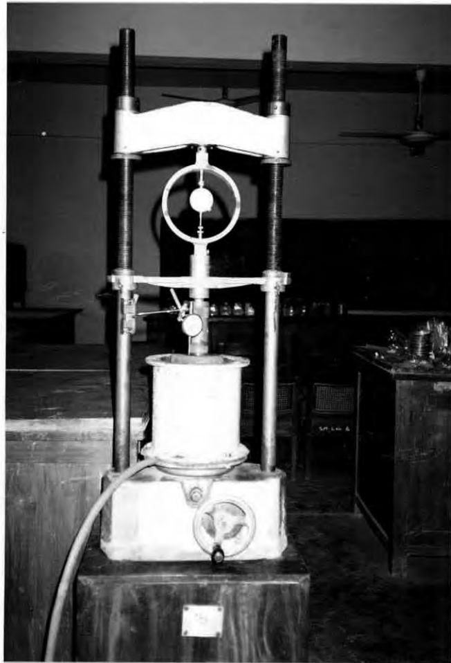
Fig. 3.2 Apparatus for K_0 consolidation of soil slurry
