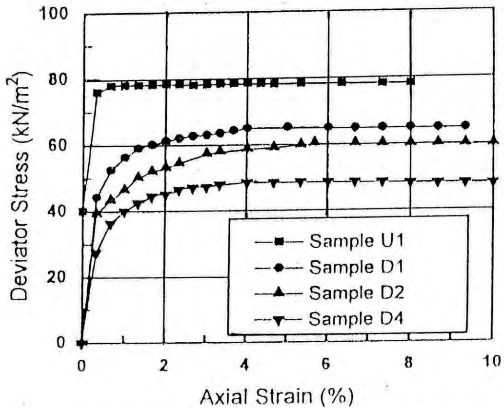
Fig.2.8 Deviator stress versus axial strain plots for “tube” samples for Dhaka clay ( after Siddique and Sarker, 1995).
