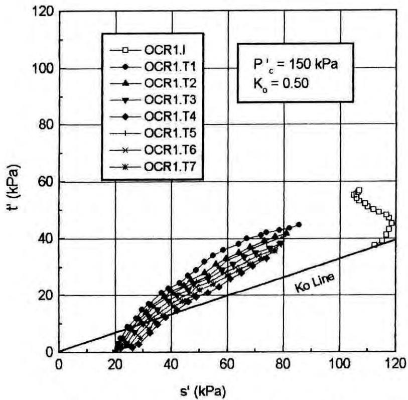
Fig. 5.8. Comparison of effective stress paths for "in situ" and "tube" samples of Dhaka clay for OCR = 1.
