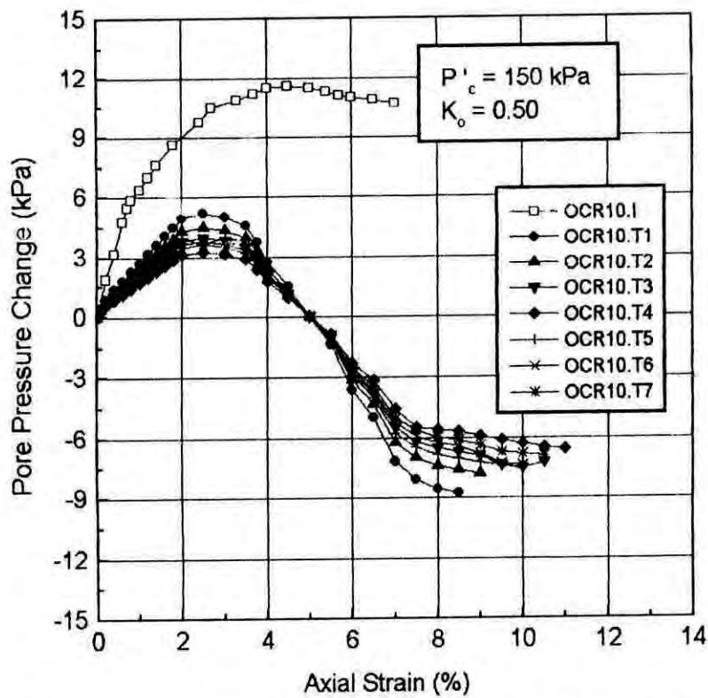
Fig.5.19. Comparison of pore pressure response between "in situ" and "tube" samples of Dhaka clay for OCR = 10.
