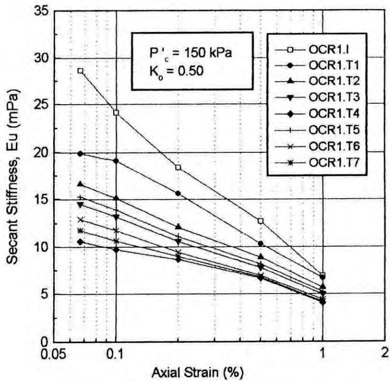
Fig.5.14 Secant stiffness vs. axial strain plots on "in situ" and "tube" samples of Dhaka clay for OCR = 1.
