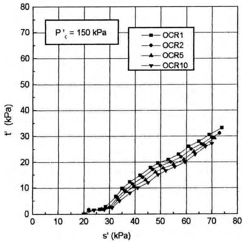
Fig. 5.22. Comparison of effective stress paths at different OCR of Dhaka clay by sampling tube no. T4.
