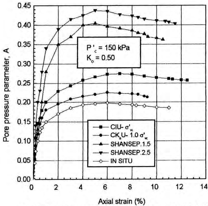
Fig. 5.53 Pore pressure parameter vs. axial strain plots for "n situ" and reconsolidated "perfect" samples of OCR = 2
