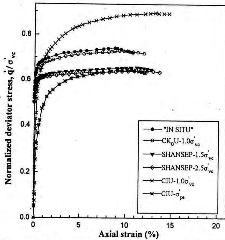
Fig.2.23 Normalized deviator stress versus axial strain plots for “in situ” and reconsolidated “perfect” samples for a normally consolidated coastal soil (after Bashar et al., 1997b).
