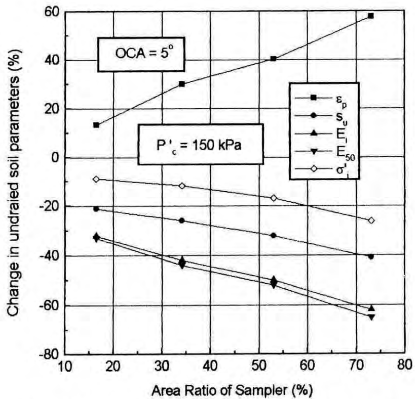
Fig. 5.23 Influence of area ratio of samples on undrained soil parameters for samples of Dhaka Clay for OCR = 1
