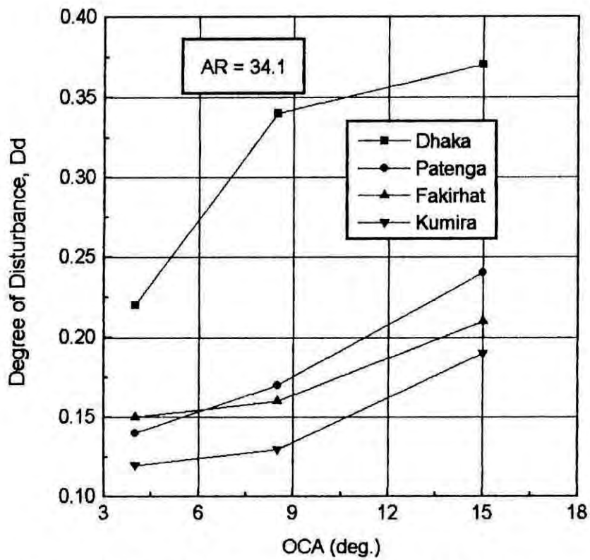
Fig. 2.19 Variation of degree of disturbance with OCA of sampler for samples (reproduced after Siddique and Sarker, 1996; Siddique et al., 2000).
