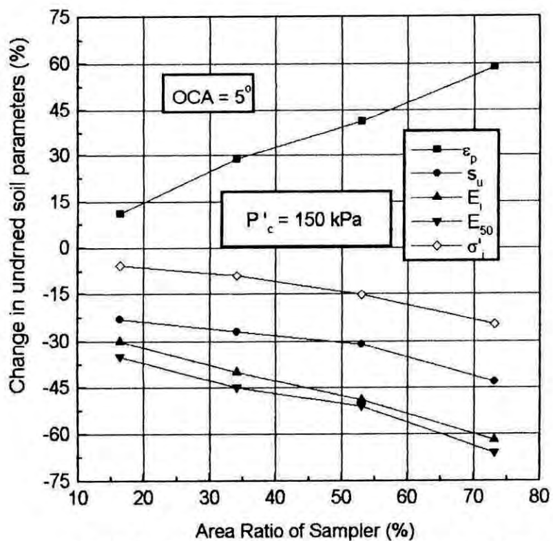
Fig. 5.24. Influence of area ratio of samplers on undrained soil parameters for samples of Dhaka Clay for OCR = 2.
