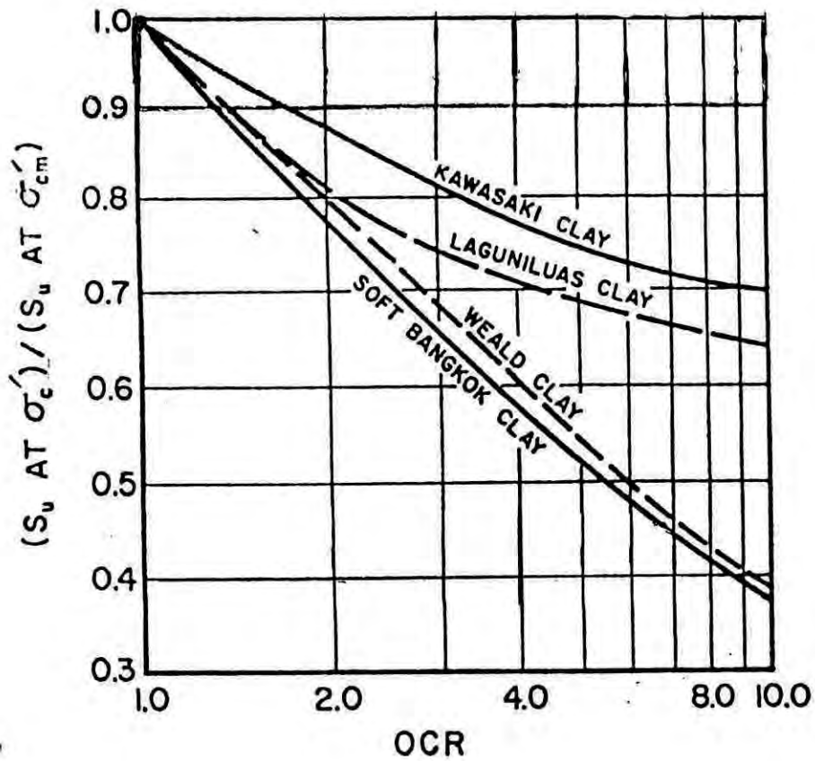
Fig.2.20 Effect of OCR on Undrained strength for various clays (after Nelson et al, 1971).
