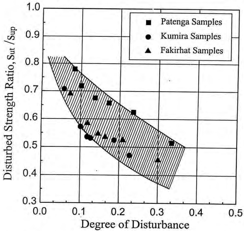
Fig.2.21 Disturbed strength ratio versus degree of disturbance plot for samples of three coastal soils (after Siddique et al, 2000).
