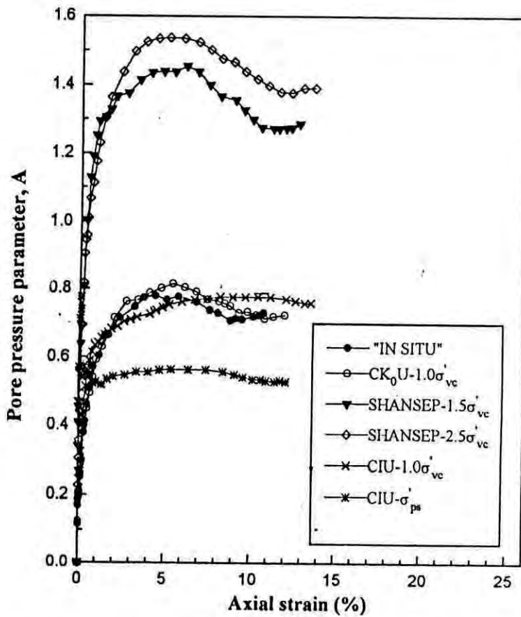
Fig.2.24 Pore pressure parameter, A versus axial strain plots for “in situ” and reconsolidated “perfect” samples for a normally consolidated coastal soil (after Bashar et al., 1997b)
