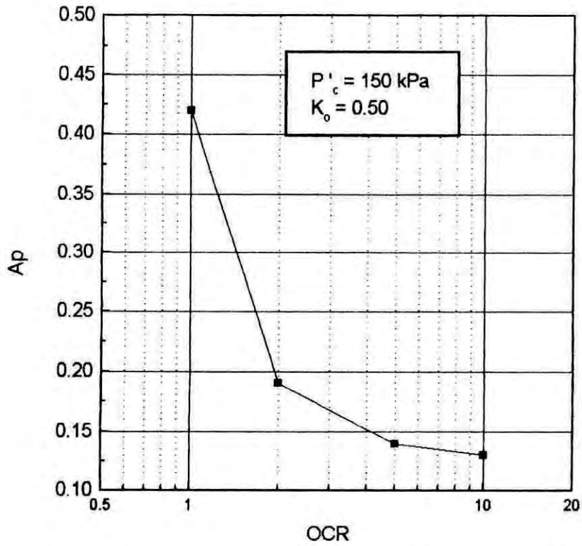
Fig.5.7 Variation of A_p with OCR for "In situ" samples of Dhaka Clay.
