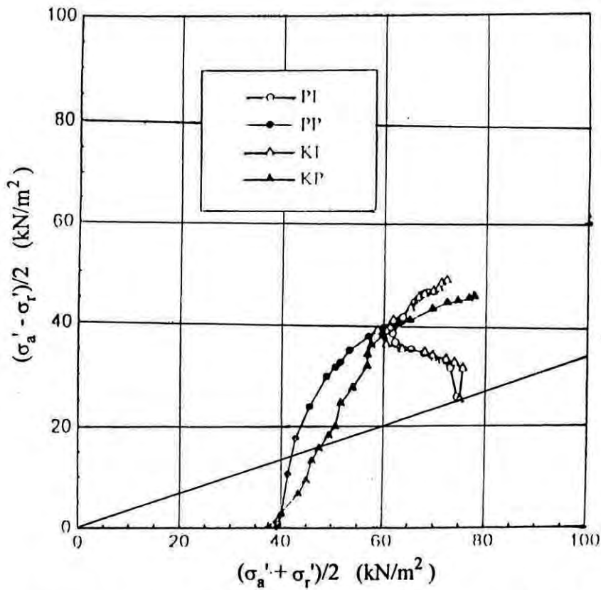
Fig.2.2 Effective stress paths of "perfect" and "in situ" samples from Patengha and Kumira (after Siddique and Farooq, 1996).
