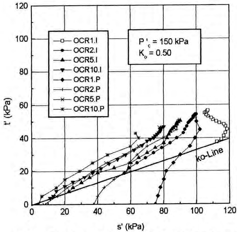
Fig. 5.43. Comparison of effective stress paths for "in situ" and "perfect" samples of Normally consolidated and Overconsolidated Dhaka Clay.
