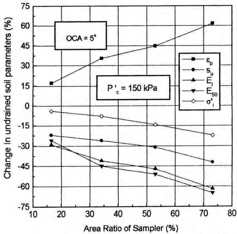
Fig.5.25. Influence of area ratio of samplers on undrained soil parameters for samples of Dhaka Clay for OCR = 5.
