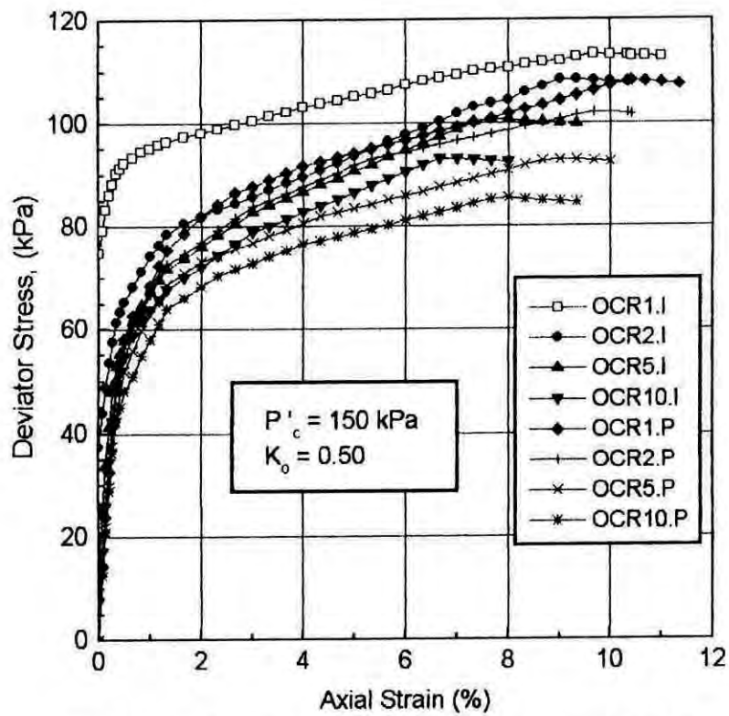
Fig.5.44 Deviator Stress vs. Axial strain (%) plots for "in situ" and "perfect" samples of Normally consolidated and Overconsolidated Dhaka Clay.
