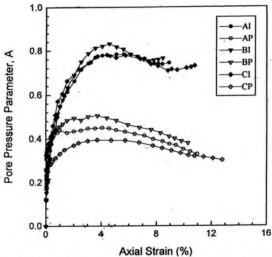
Fig.2.4 Comparison of pore pressure parameter, A vs. Axial strain plots of “perfect” and “in situ” samples from three coastal soils ( after Bashar et al, 1997a).
