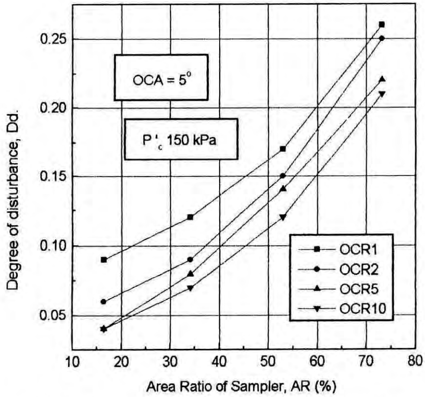
Fig. 5.38. Variation of degree of disturbance with area ratio (%) of sampler for samples of Dhaka clay for different OCR.
