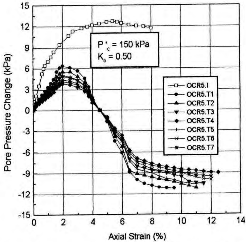
Fig.5.18. Comparison of pore pressures response between "in situ" and "tube" samples of Dhaka Clay for OCR = 5.
