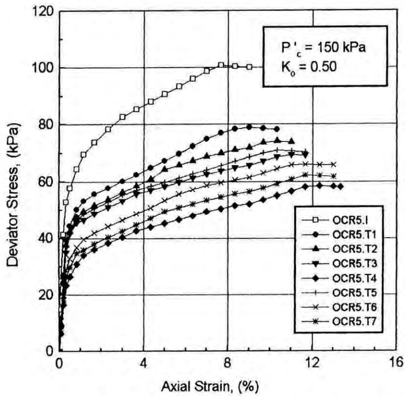
Fig. 5. 12. Comparison of deviator stress vs. axial strain for "in situ" and "tube" samples of Dhaka clay for OCR = 5.
