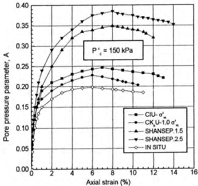
Fig.5.49 Pore pressure parameter vs. axial strain plots for "in situ" and reconsolidated "tube" samples of OCR=2.
