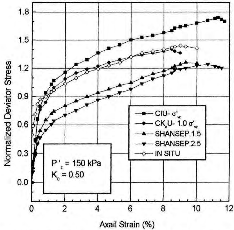
Fig.5.51 Normalized Deviator Stress vs. Axial Strain (%) plots for "In situ" and Reconsolidated "Perfect" samples of Dhaka Clay for OCR = 2.
