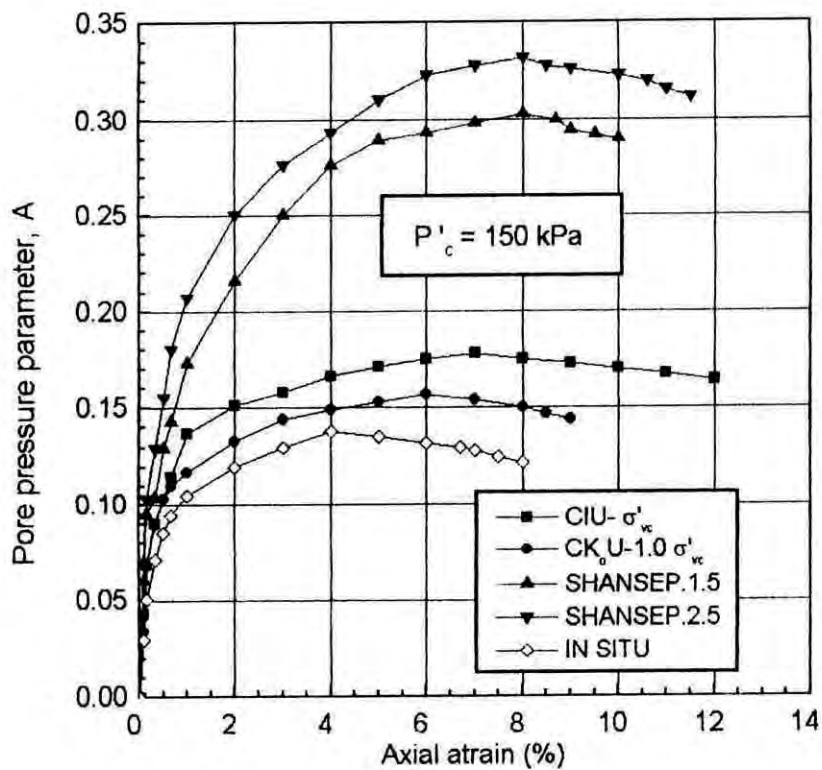
Fig.5.50 Pore pressure parameter, vs. axial strain plot for "in situ" and reconsolidated "tube" samples of OCR = 10.
