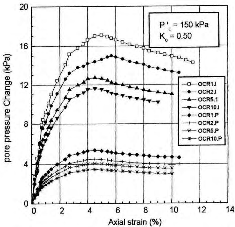
Fig.5.46 Pore pressure change versus Axial strain(%) plots for "in situ" and "perfect" samples of Normally consolidated and Overconsolidated Dhaka Caly.
