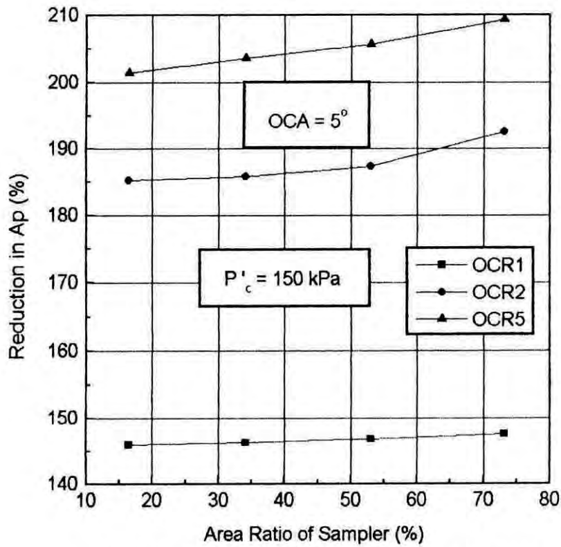
Fig.5.27 Influence of area ratio of samplers on A_p for samples of different OCR.
