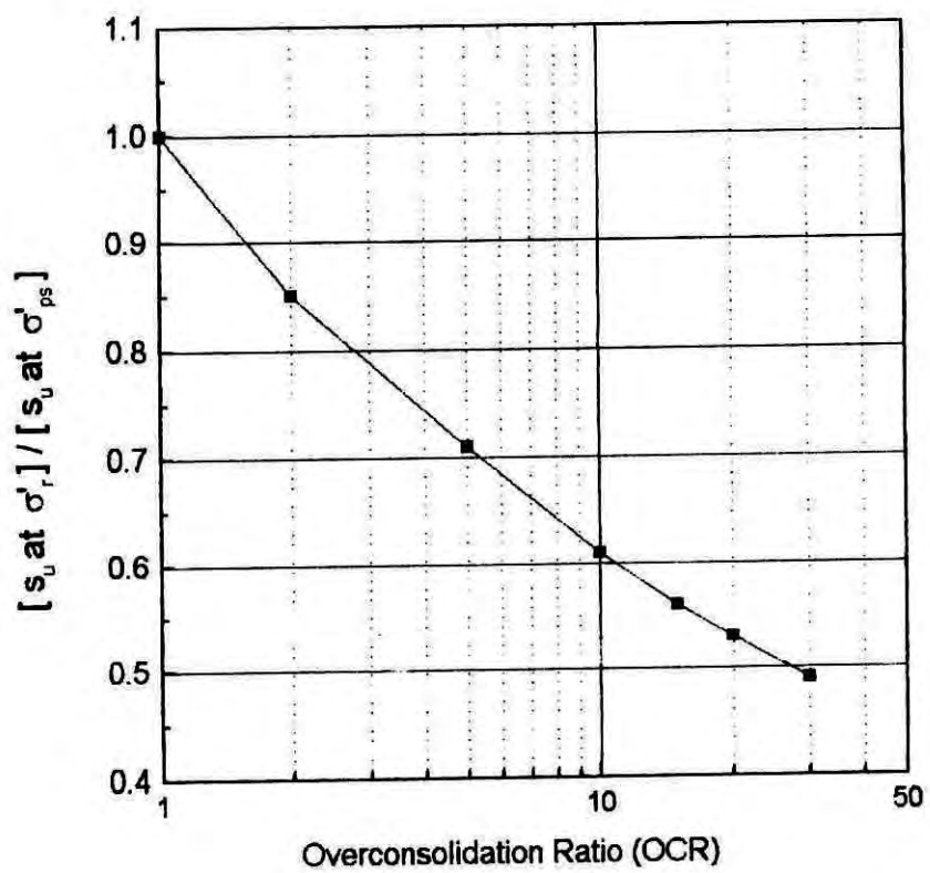
Fig.5.42 Undrained Shear Strength correction curve of Dhaka clay.
