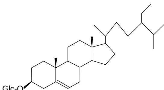
\beta -Sitosterol-3-O-D-glucoside ( 19 )
