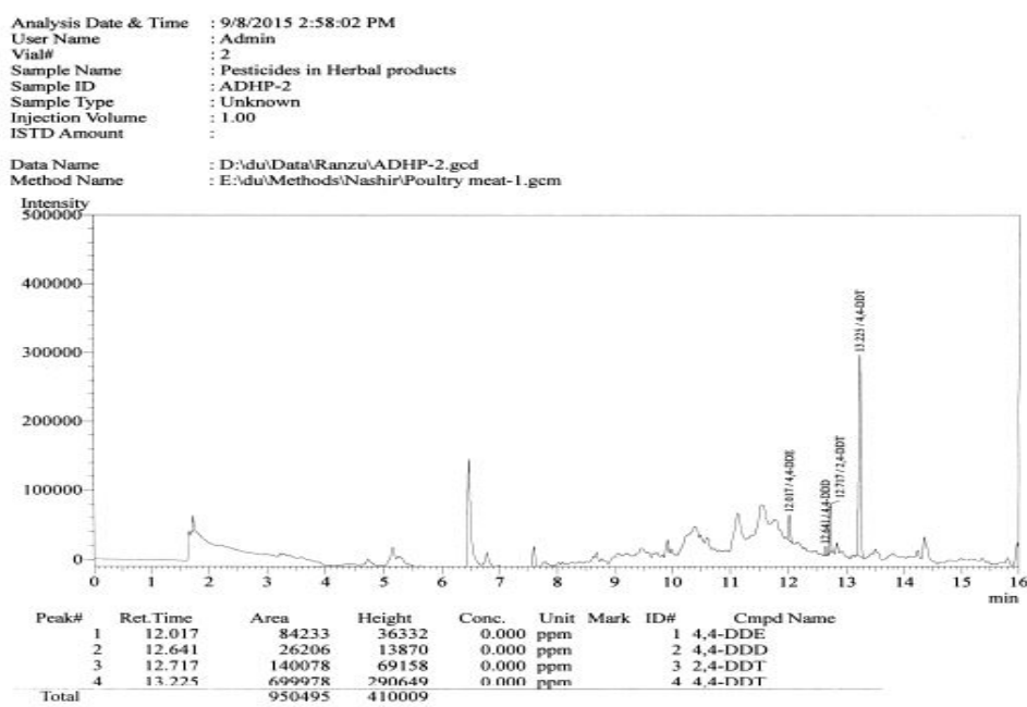
Figure-3.9.3: GC chromatogram for analysis of pesticide residues in ADHP-2
