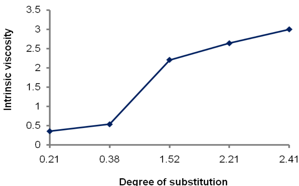
Figure 2.10 Relationship between degree of substitution and intrinsic viscosity of prepared CMC.
