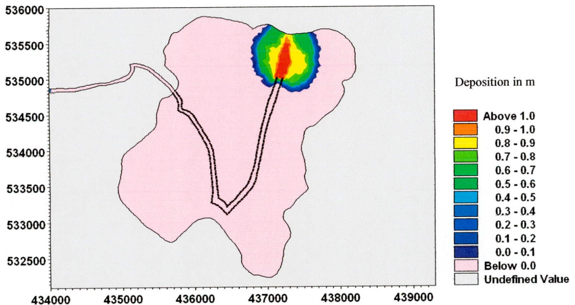
Figure 5.6.8: Simulated deposition pattern inside the tidal basin after first year with embankment length of 3800 m for Option-3
