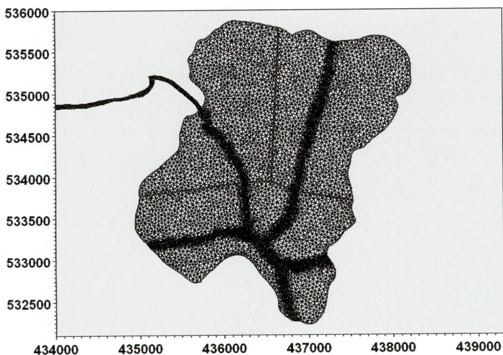
Figure 5.2.1: Schematization of sediment transport model of Beel Baruna
