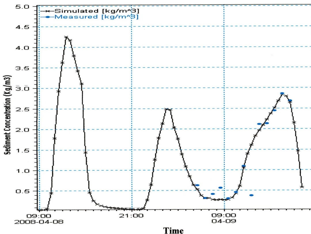
Figure 5.3.2: Observed and simulated suspended sediment concentration in the Hari River near Dierkatakhali link canal of East Beel Khukshia
