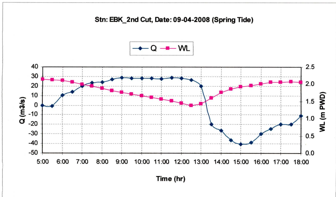
Figure B-5: Water Level and Discharge Hydrograph of EBK 2nd Cut
