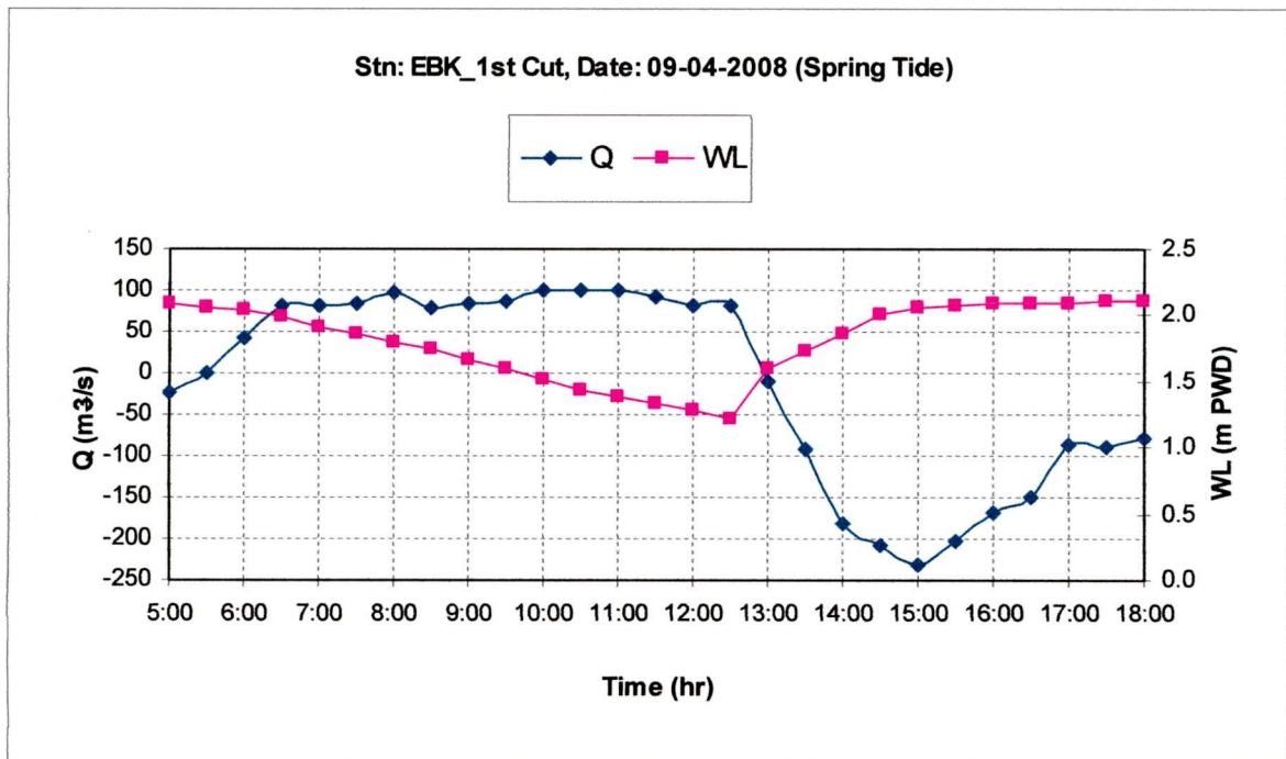
Figure B-4: Water Level and Discharge Hydrograph of EBK 1st Cut
