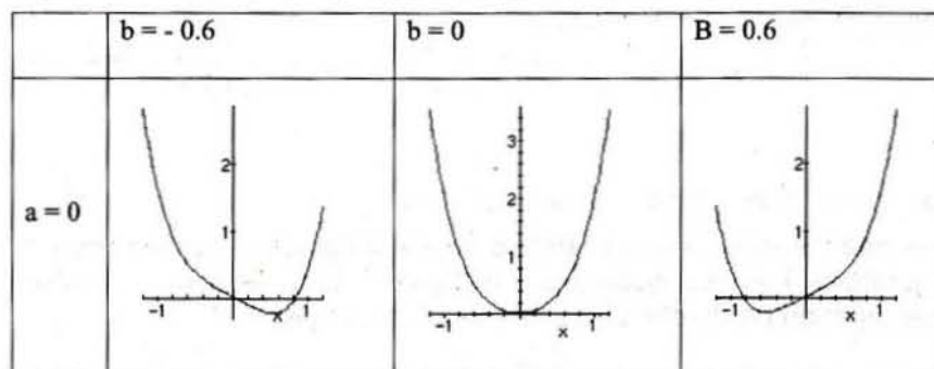
Figure 3.2: Graph of y = x^4 + ax^2 + bx at a=0
