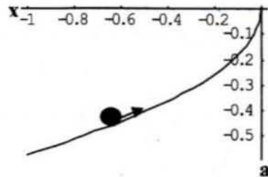
Figure 4.6: x = -\frac{\sqrt{-a}}{\sqrt{3}}
