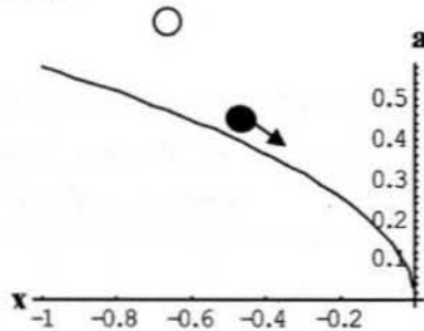
Figure 4.5: x = \frac{\sqrt{-a}}{\sqrt{3}}
