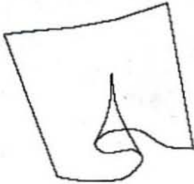
Figure 4.8: A fold catastrophe
