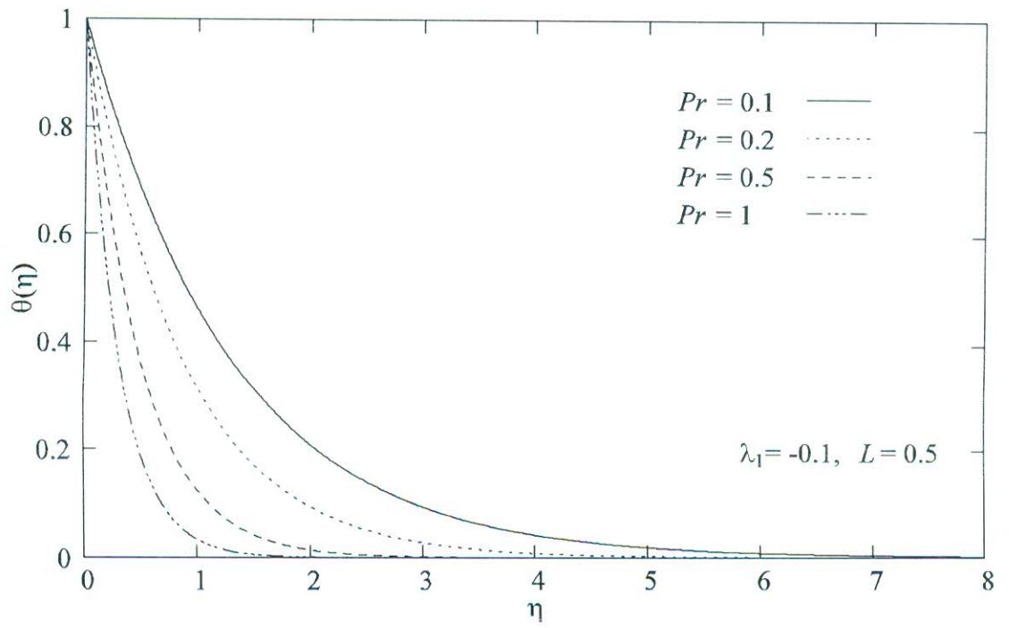
Fig3(b) Temperature profiles for several values of Pr for Walter's liquid B (i.e. \lambda_1 < 0 ).
