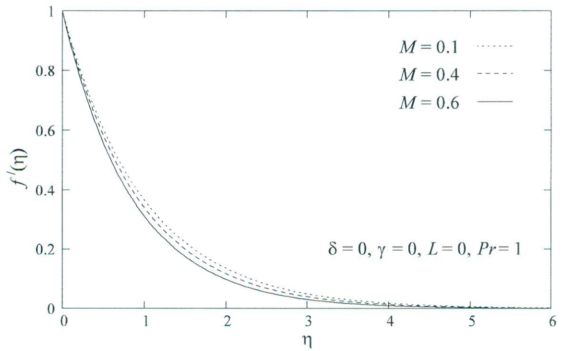
Fig1 Variation of horizontal velocity f'(\eta) with \eta for several values of magnetic parameter M .
