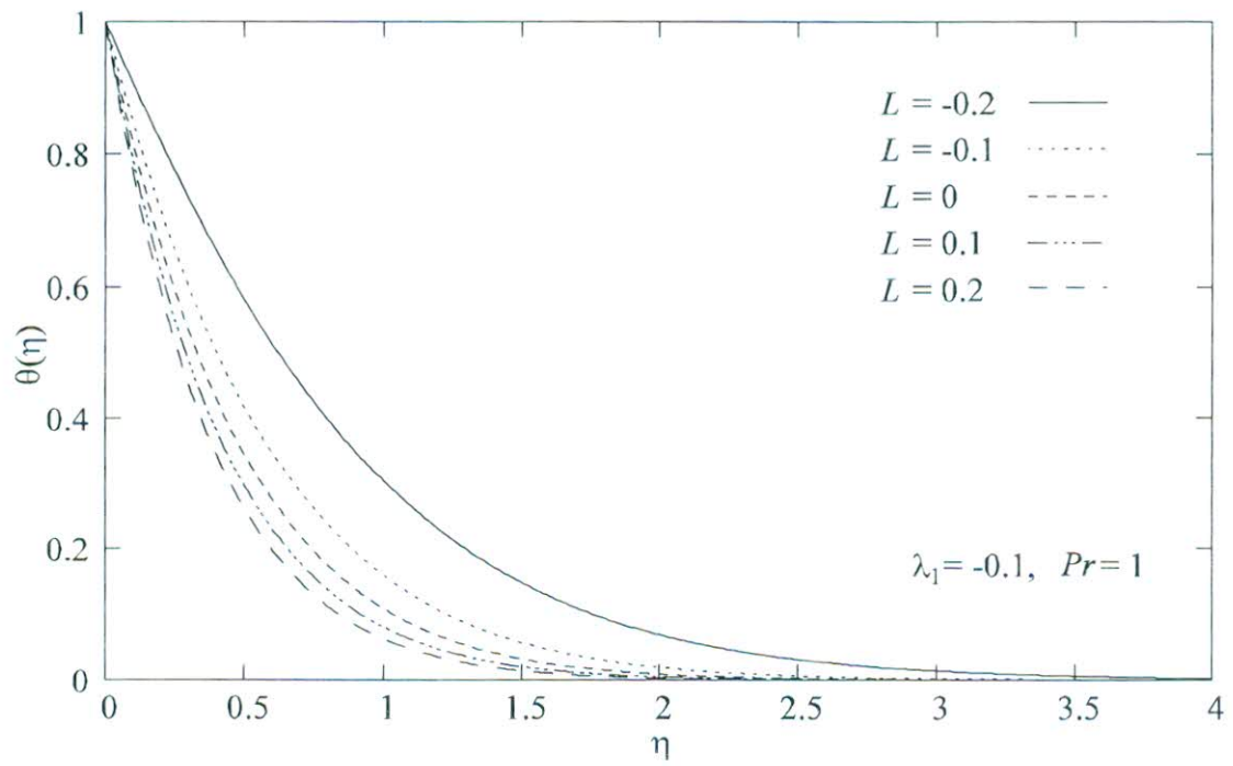
Fig4(b) Temperature profiles for several values of L for Walter's liquid B (i.e. \lambda_1 < 0 ).
