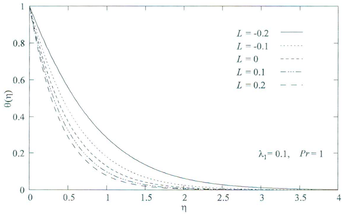
Fig4(a) Temperature profiles for several values of L for second-grade fluid (i.e. \lambda_1 > 0 ).
