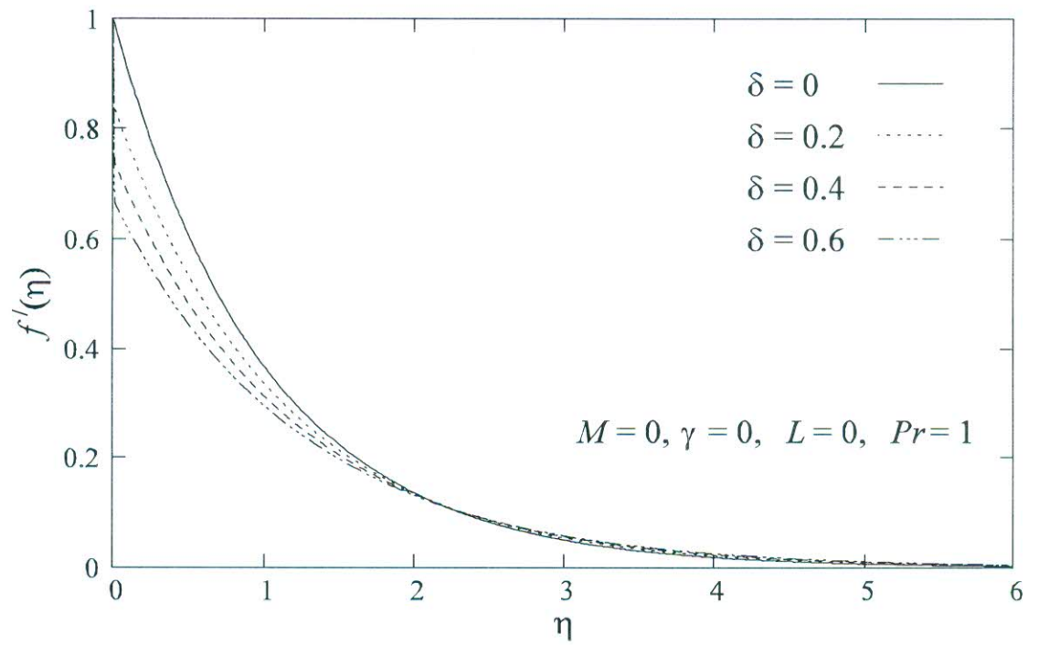
Fig3(a) Variation of horizontal velocity f'(\eta) with \eta for several values of velocity slip parameter \delta in the absence of magnetic field.
