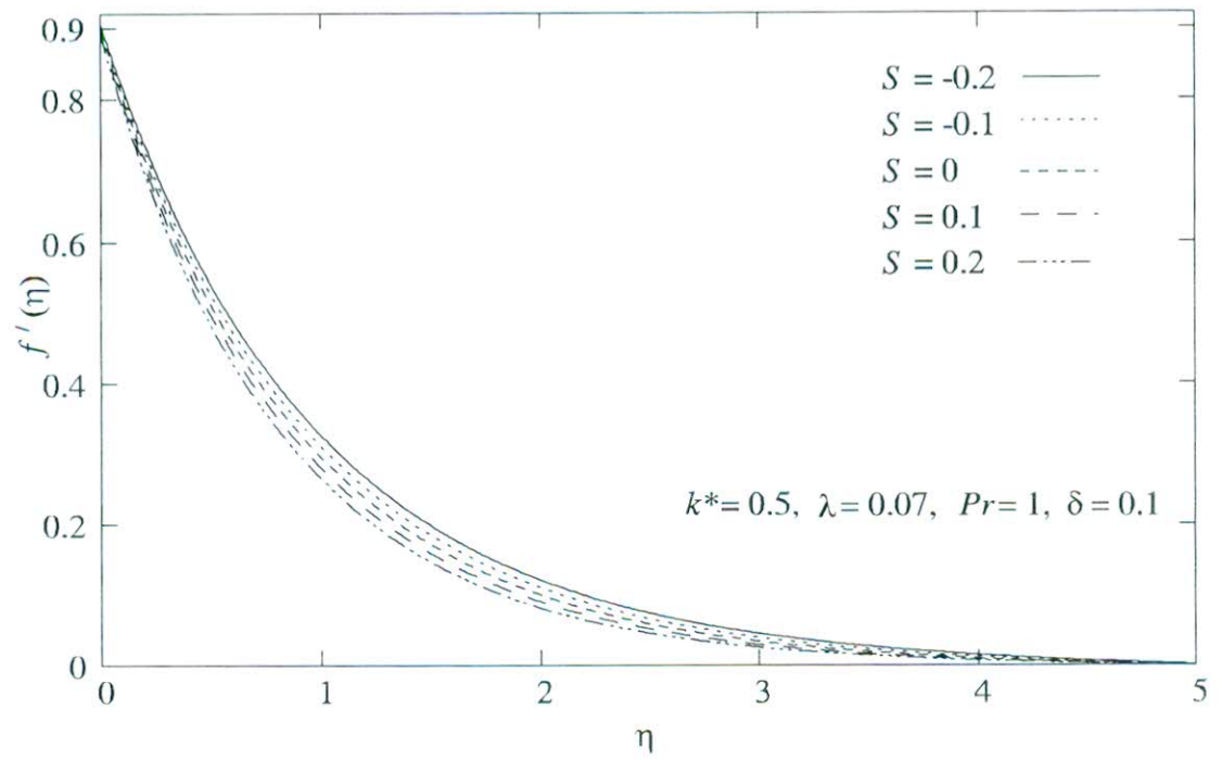
Fig10 Velocity profiles f'(\eta) for various values of suction/blowing parameter S .
