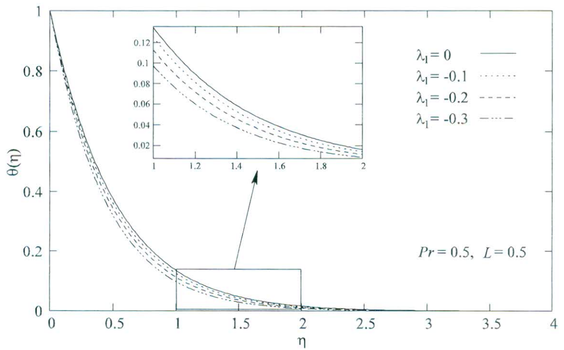
Fig2(b) Temperature profiles for several values of \lambda_1 Walter's liquid B (i.e. \lambda_1 < 0 ).
