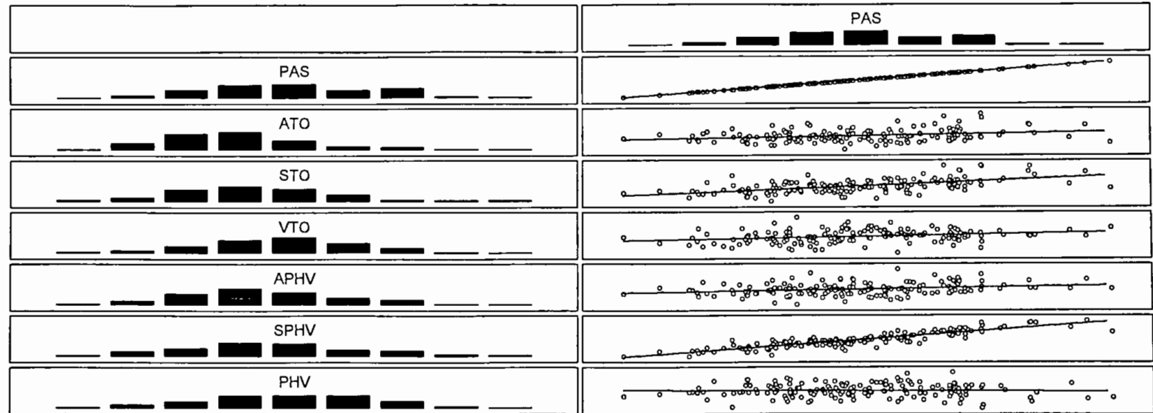
Fig. 4.2b Correlation matrix plot between adult stature and growth parameters for Japanese girls. The Parameters are drawn from the estimated distance and velocity curves of the JPA-2 model. The growth parameters are; age at takeoff (ATO), stature at takeoff (STO), velocity at takeoff (VTO), age at peak height velocity (APHV), stature at peak height velocity (SPHV), peak height velocity (PHV), and predicted adult stature (PAS). Bar diagram of the graph indicates the distribution of the parameter-variables. In every element in the matrix, the X-axis is for PAS. Only the pattern, either linear or nonlinear, is of concern. No scales are shown here.
