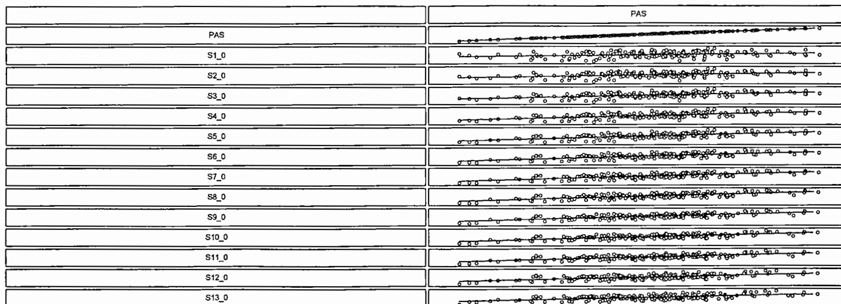
Fig. 4.3b Correlation matrix plot between adult stature and stature at different ages for Japanese boys. The statures are drawn from the estimated distance curves of the JPA-2 model. The predicted statures considered in this study are: stature at age 2 (S2), stature at age 3 (S3), stature at age 4 (S4), stature at age 5 (S5), stature at age 6 (S6), stature at age 7 (S7), stature at age 8 (S8), stature at age 9 (S9), stature at age 10 (S10), stature at age 11 (S11), stature at age 12 (S12), stature at age 13 (S13) and predicted adult stature (PAS). In every element in the matrix, the X-axis is for PAS. Only the pattern, either linear or nonlinear, is of concern. No scales are shown here.
