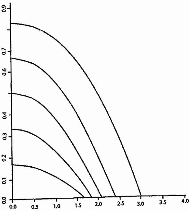
Fig.-3.2 : Depicts the solution processes of h(\mu)
