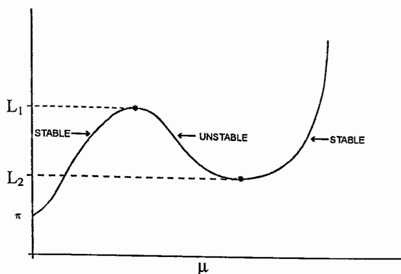
Fig.-3.9 : Depicts schematic representation of the stability of the model depends upon roots of the cubic equation.
