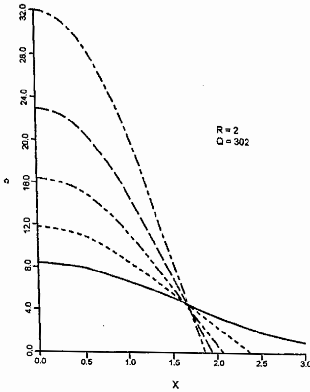
Fig.-3.12: Graphical representation of \eta(x) and \mu for
