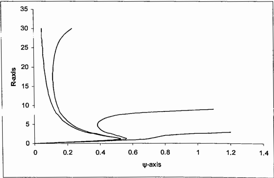
Fig-2.14 : Depicts the relationship between the control parameter R and population size \psi for different values of Q .
