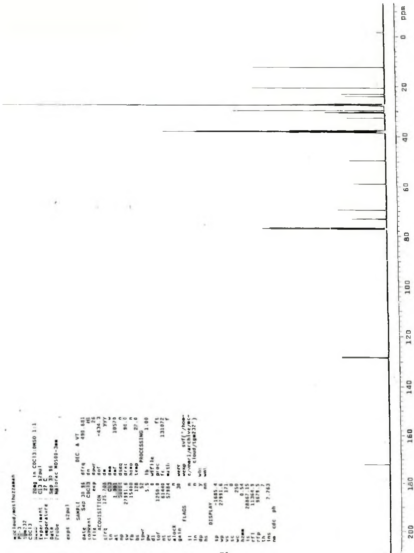
Fig.9: ^{13}\text{C} -NMR spectrum of compound PC 3
