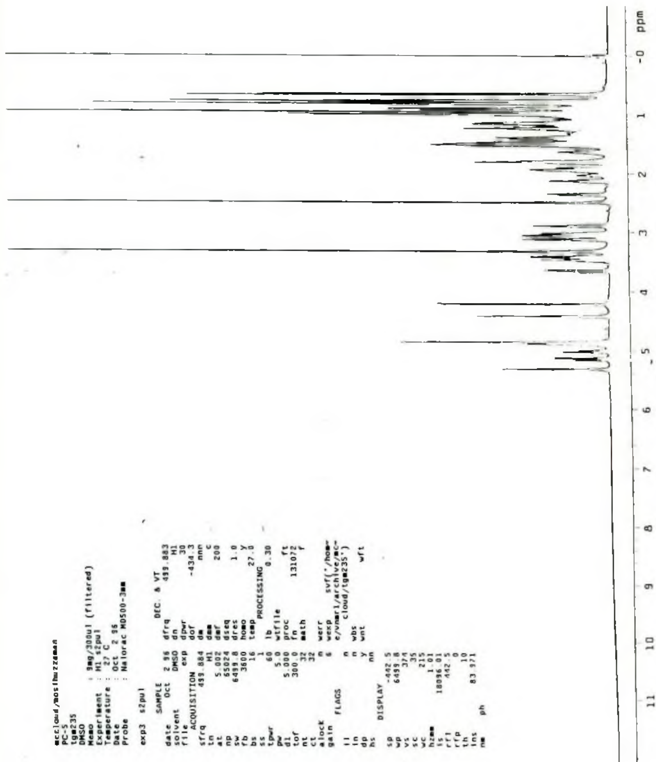
Fig.23: 1 H-NMR spectrum of compound PC 5
