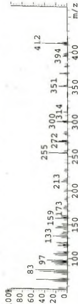
Fig. 5: Mass spectrum of compound C1
