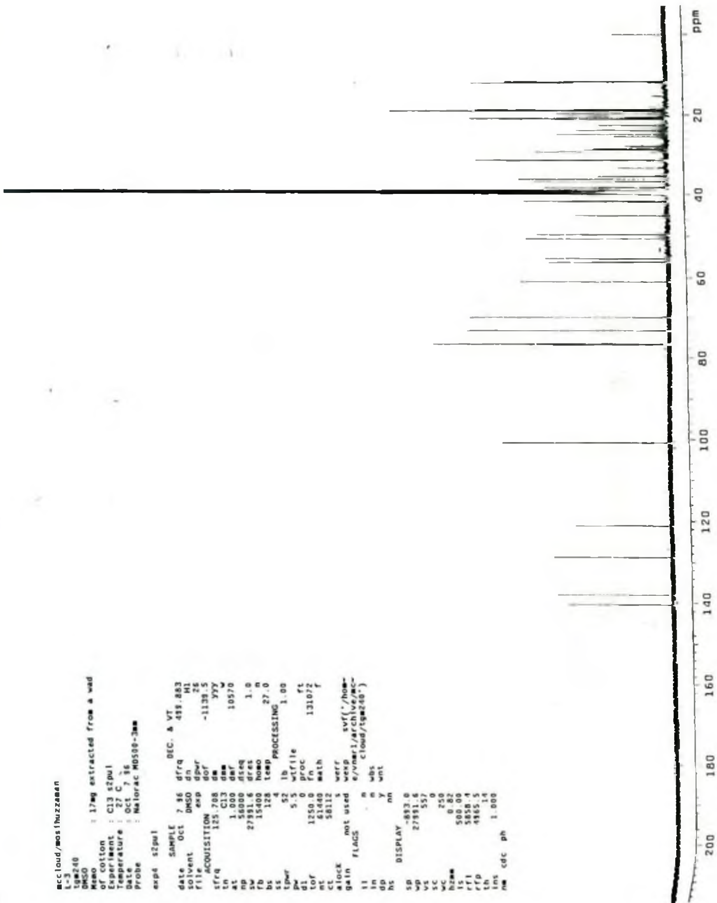
Fig.24: ^{13}\text{C} -NMR spectrum of compound PC 5
