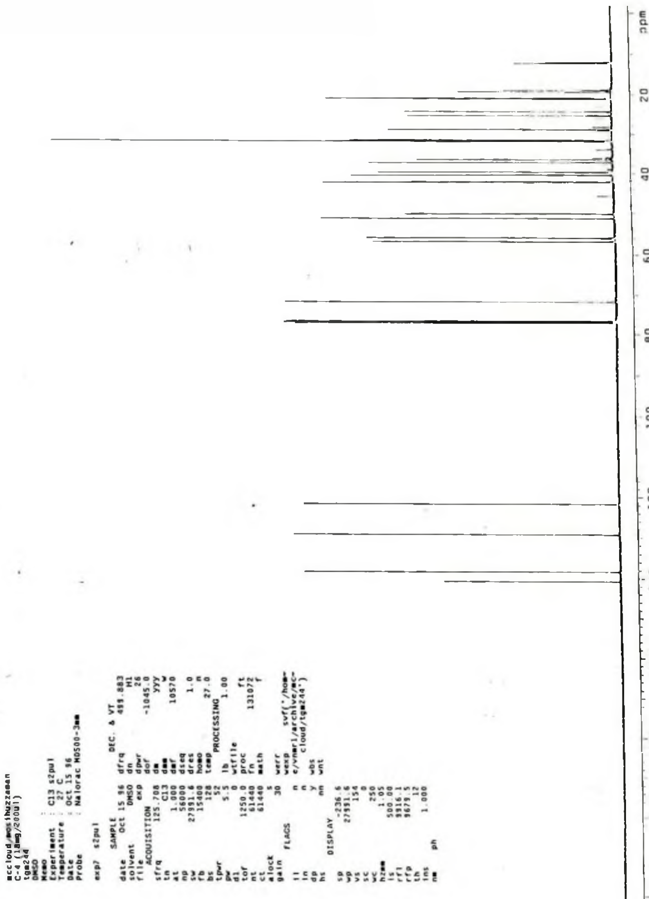
Fig.4: 13 C-NMR spectrum of compound C 4
