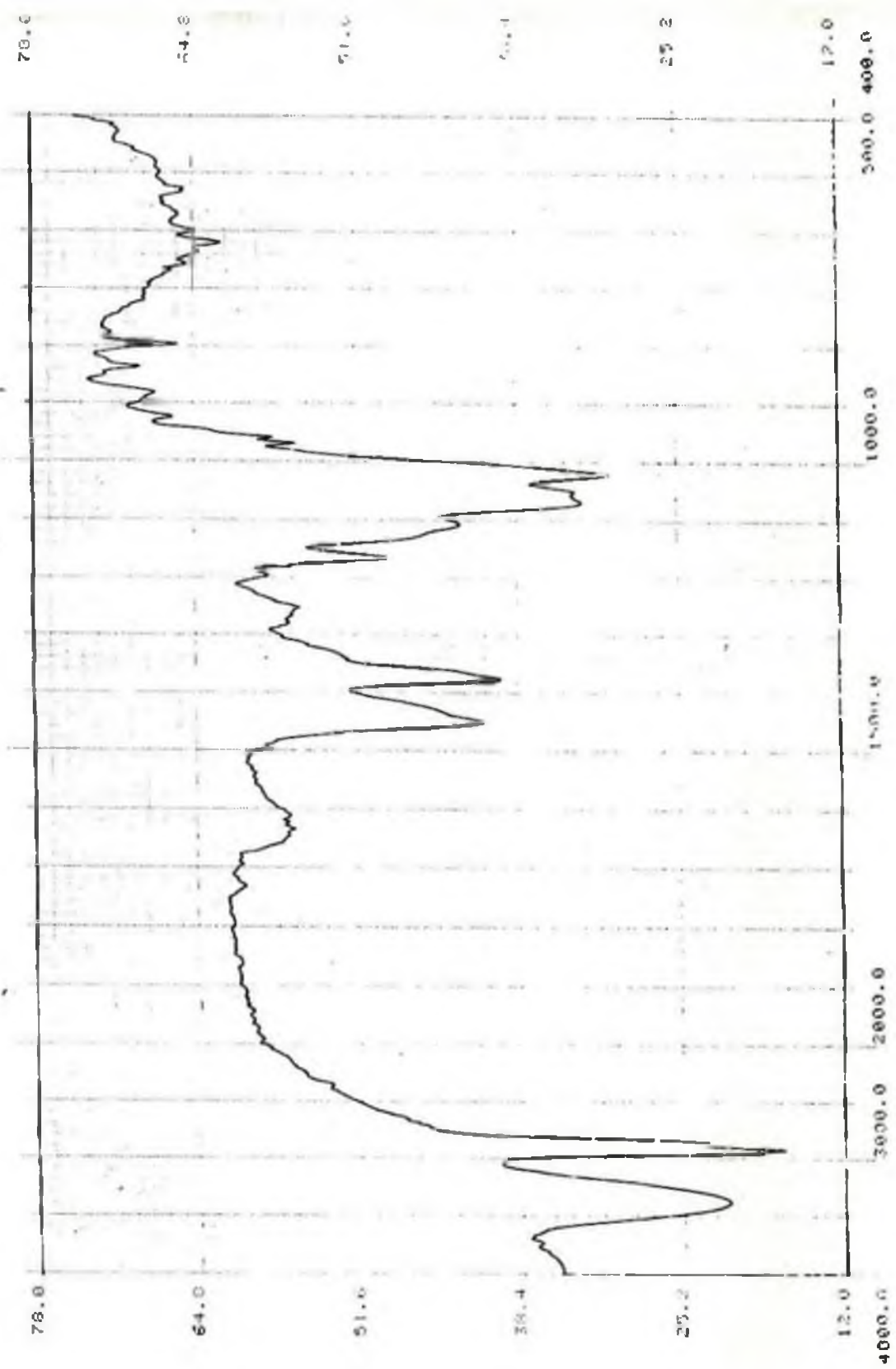
Fig 22: IR spectrum of compound PC 4
