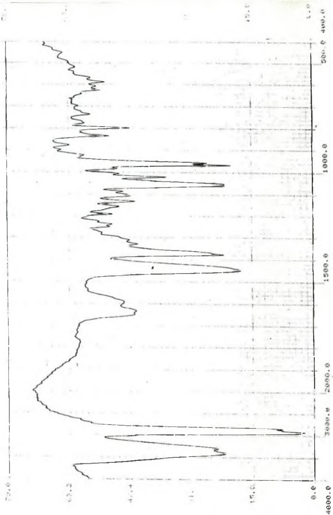
Fig 2 : IR spectrum of compound C4
