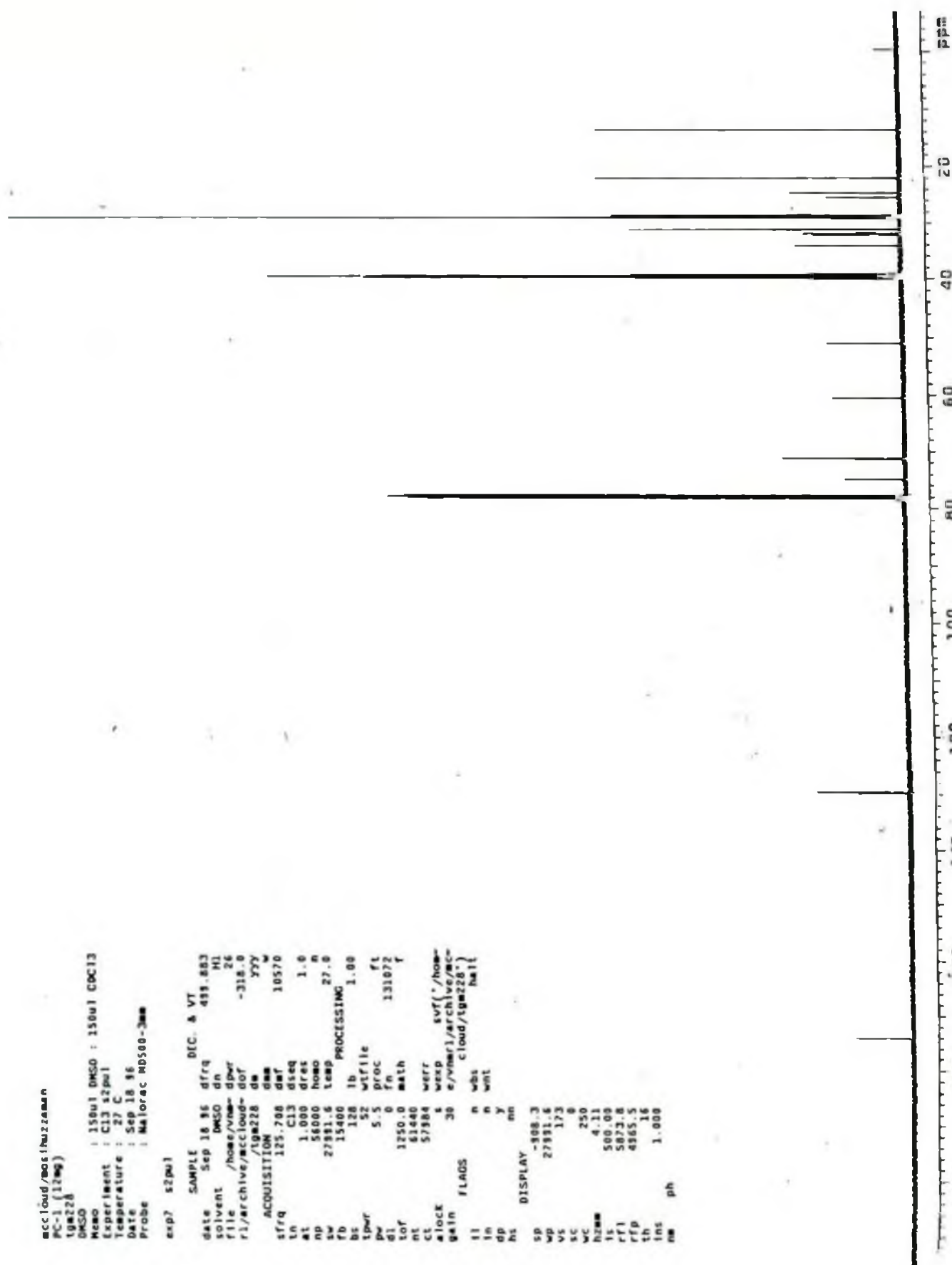
Fig.14: 13 C-NMR spectrum of compound PC 1
