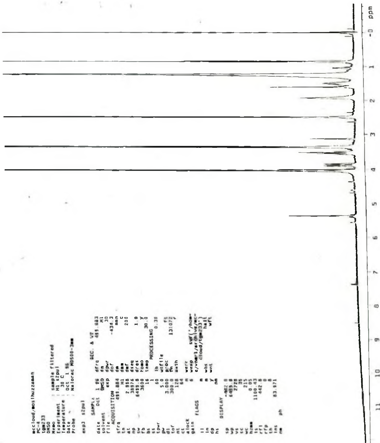
Fig.28: 1 H-NMR spectrum of compound L1
