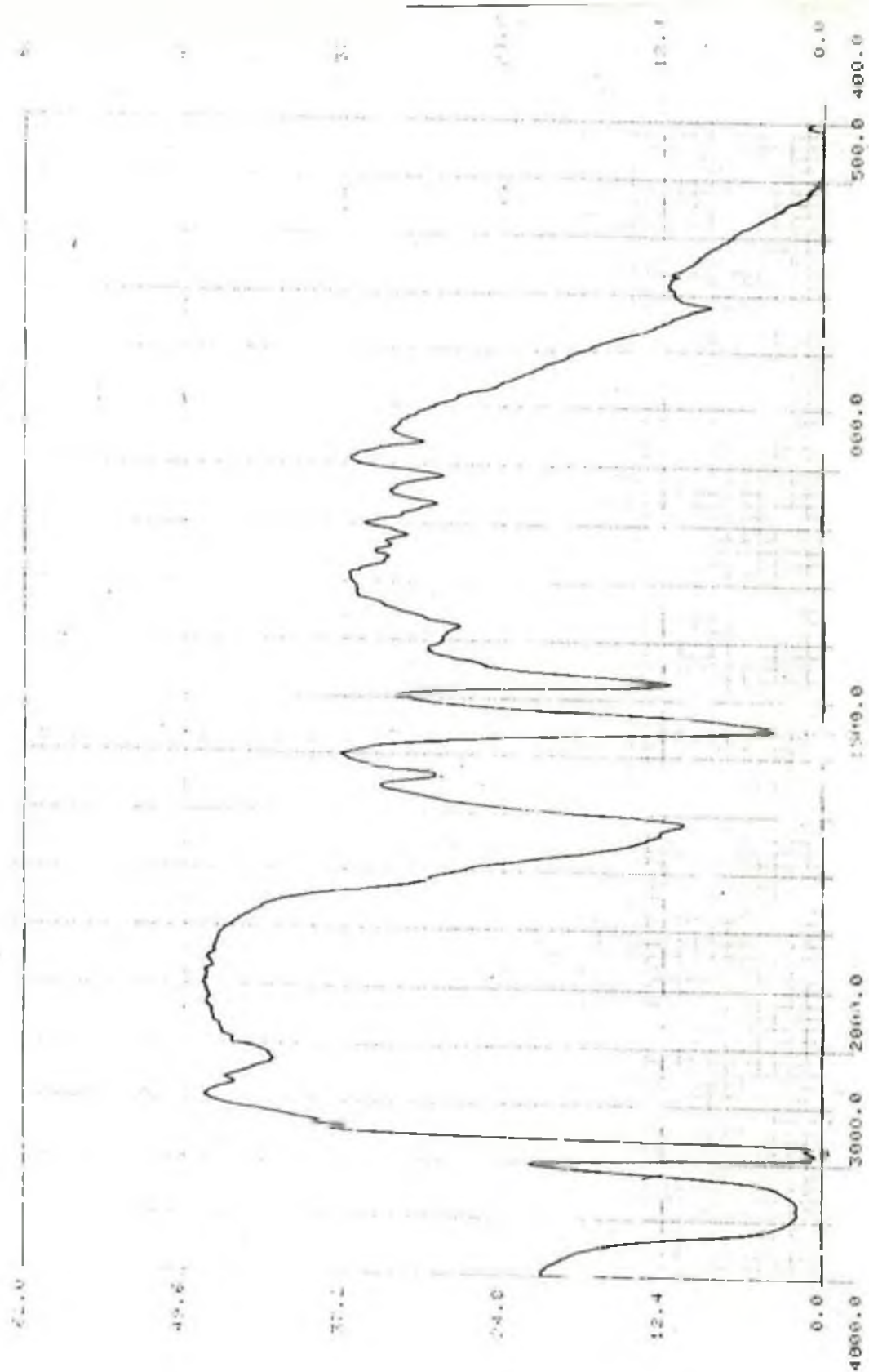
Fig.7: IR spectrum of compound PC 3
