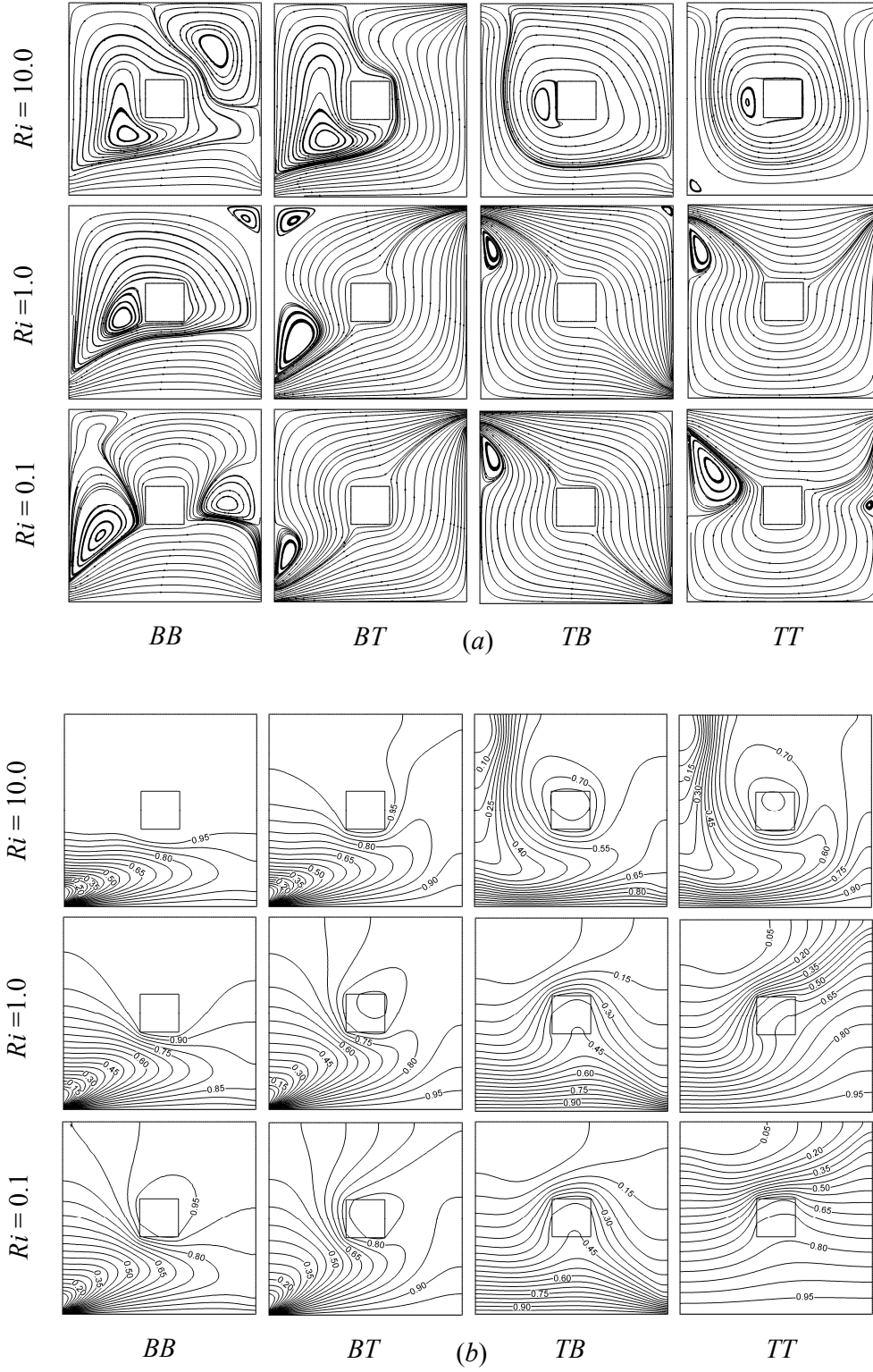
Figure 3.3: (a) Streamlines and (b) Isotherms at different inlet and outlet locations and various values of Richardson number Ri , while Re = 100 , Ha = 10 , K = 5 , Pr = 0.71 , Q = 1 and D = 0.2 .
