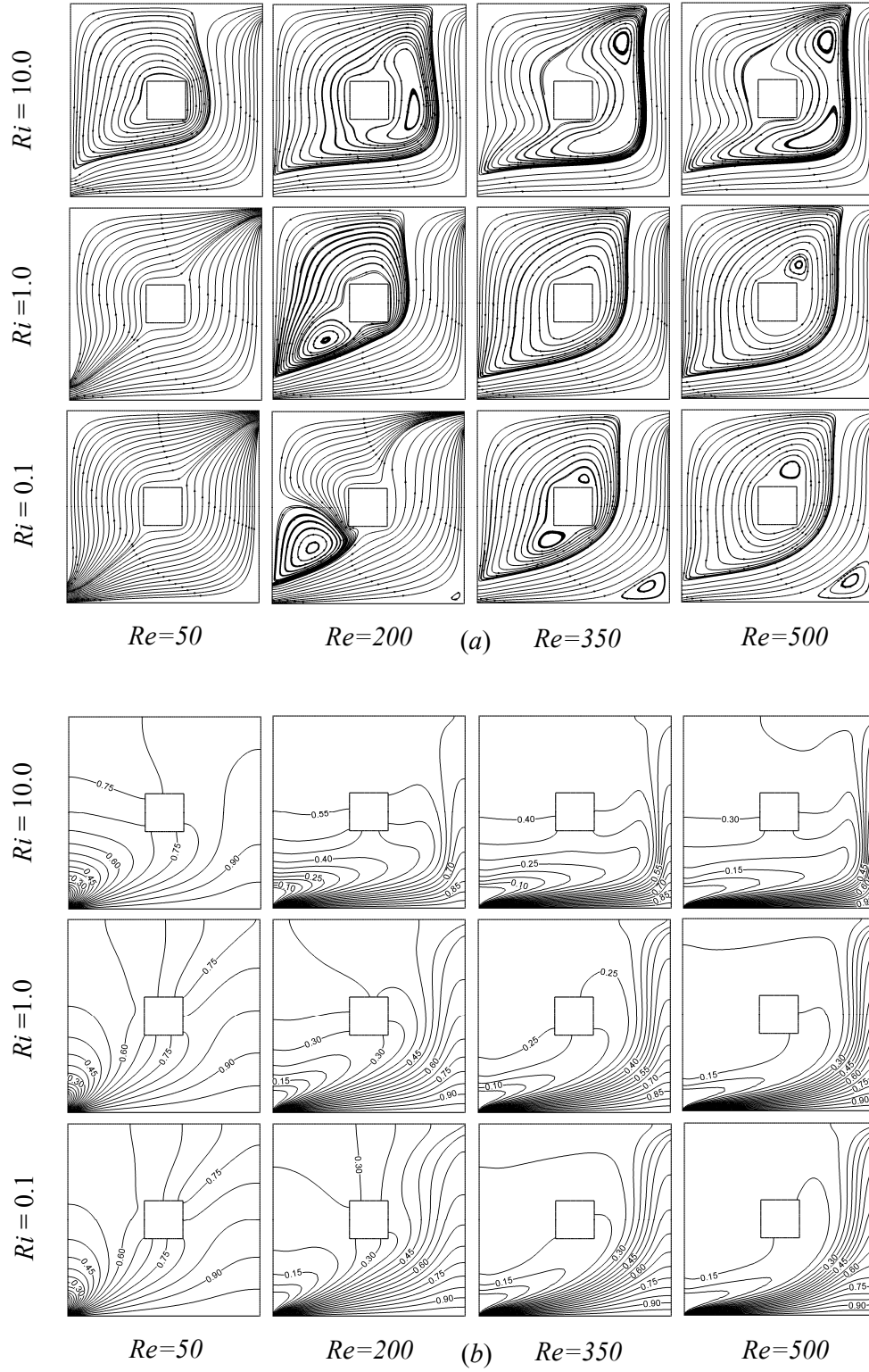
Figure 6.4: (a) Streamlines and (b) Isotherms at different Reynolds number and various values of Richardson number Ri , while Ha = 10 , K = 5 , Pr = 0.71 , Q = 1 and D = 0.2
