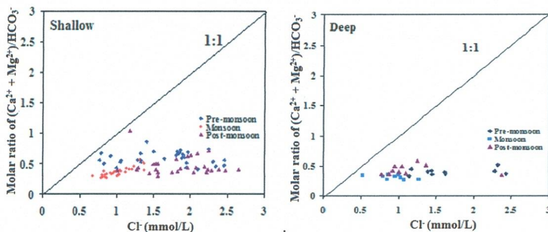
Figure 10. Scatter diagram of m(\text{Ca}^{2+} + \text{Mg}^{2+})/m\text{HCO}_3^- versus \text{Cl}^- of shallow and deep tubewells water samples of the study area.
