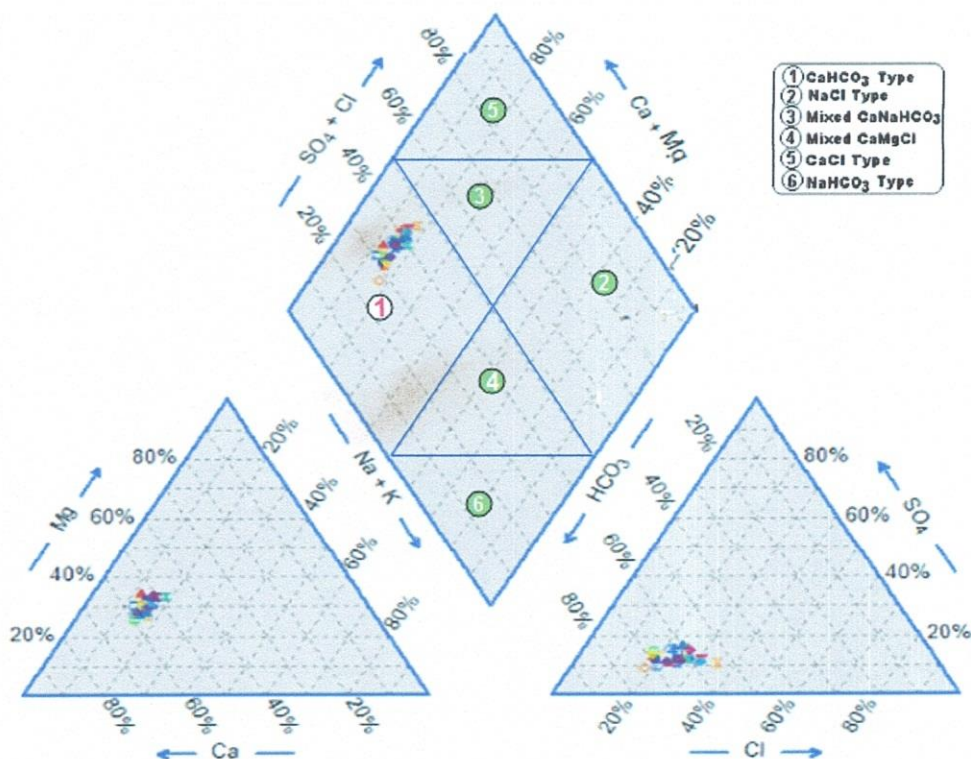
Figure 4. Hydro-chemical facies of groundwater in Rajshahi City in Piper diagram constructed using AUCHEM software Version 5.1 (water type: \text{Ca}^{2+} - \text{HCO}_3^- ).
