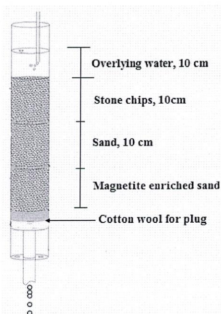
Figure 2. Schematic diagram of experimental packed column.
