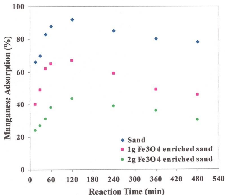
Figure 18. Adsorption of \text{Mn}^{2+} as a function of time for the 3.0 mg/L initial \text{Mn}^{2+} concentration spiked groundwater.
