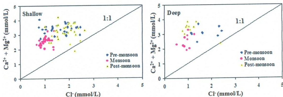
Figure 15. Relation between (\text{Ca}^{2+} + \text{Mg}^{2+}) and \text{Cl}^- .
