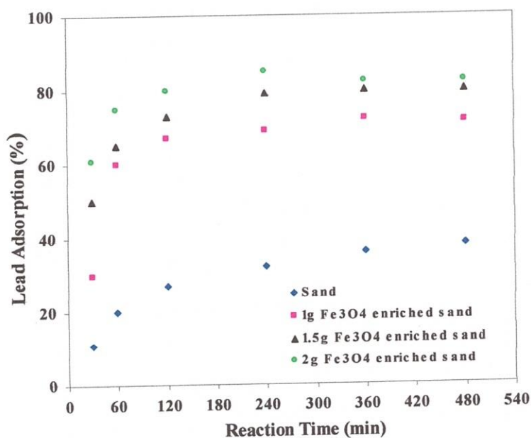
Figure 21. Adsorption of \text{Pb}^{2+} as a function of time for the 3.0 mg/L initial \text{Pb}^{2+} concentration spiked groundwater.
