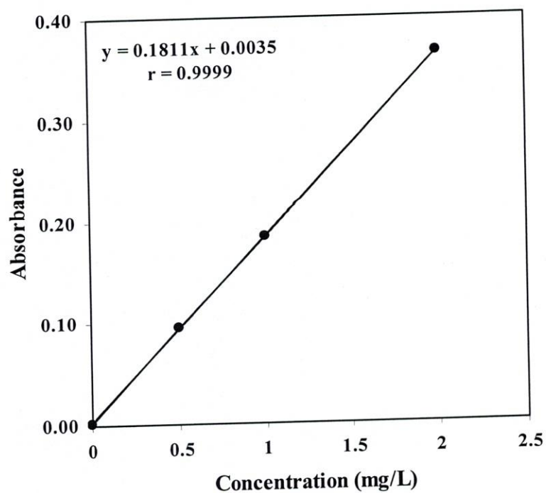
Figure 2.12. Standard curve of nitrate (NO 3 - ).
