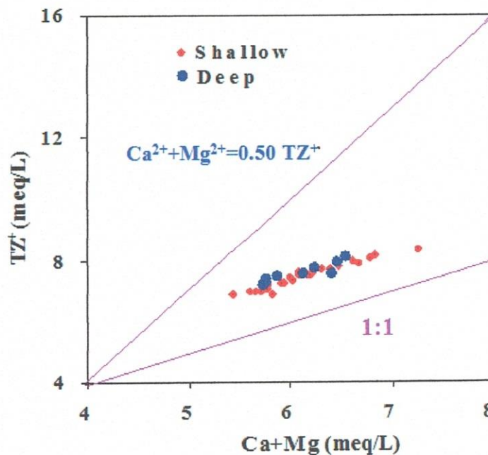
Figure 7. Scatter diagram of (\text{Ca}^{2+} + \text{Mg}^{2+}) versus total cations ( \text{TZ}^+ ).
