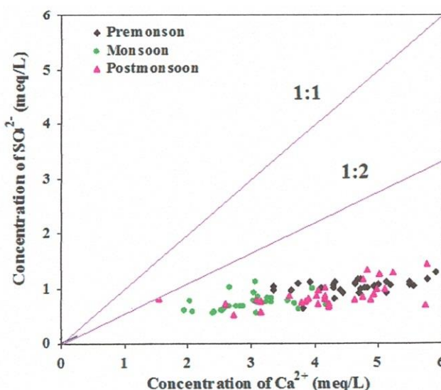
Figure 11. Scatter diagram of \text{Ca}^{2+} versus \text{SO}_4^{2-} of the groundwater samples of the study area.
