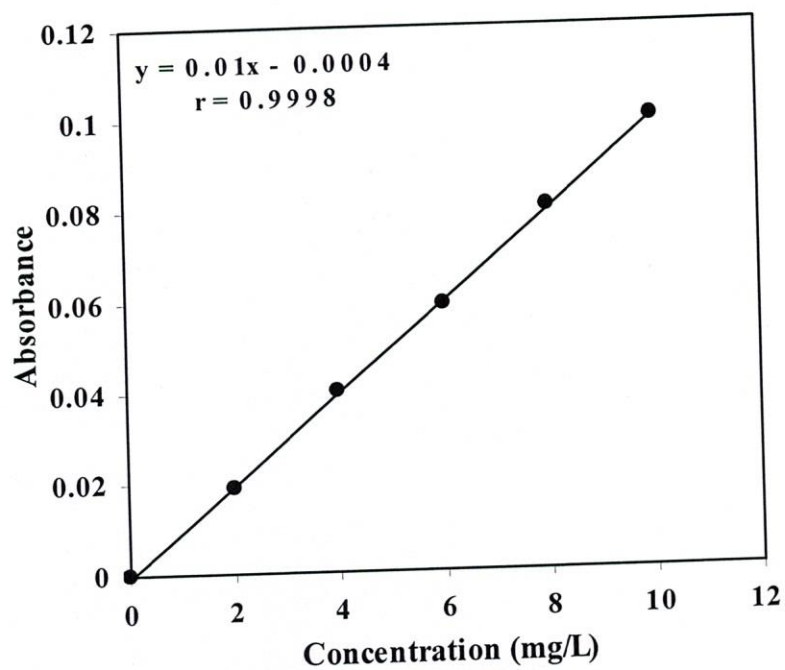
Figure 2.13. Standard curve of sulphate ( \text{SO}_4^{2-} ).
