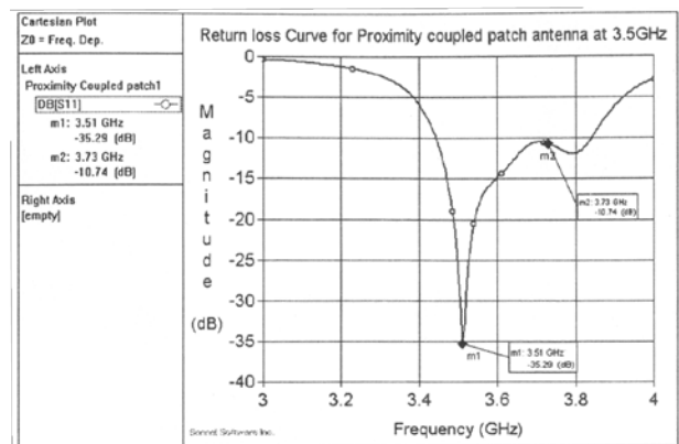
Figure 9. Simulated Return Loss of Proximity Coupled Patch Antenna.
