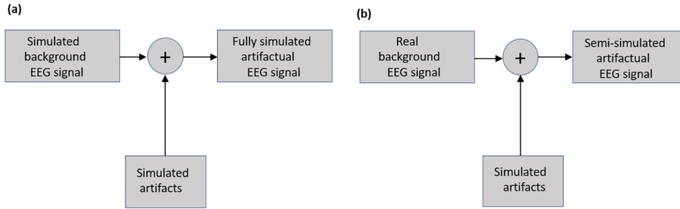
Fig. 3. Process to simulate the artifactual EEG signals: fully simulated artifactual EEG signal (a) and semi-simulated artifactual EEG signal (b).
