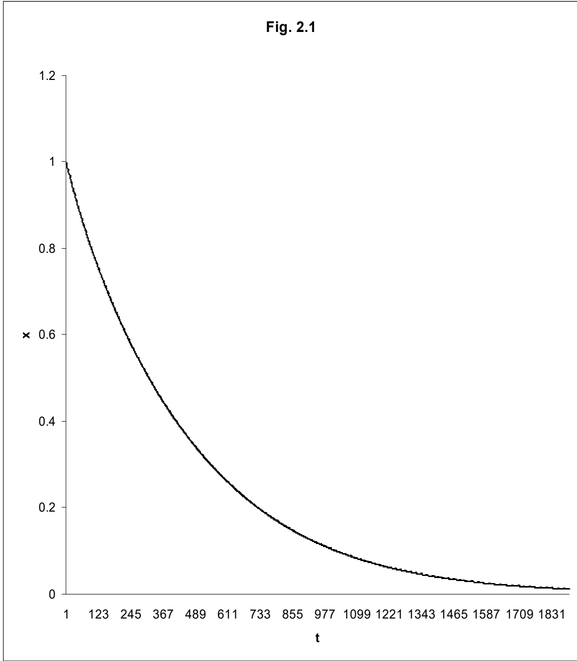
Fig 2.1: Perturbation solution with corresponding numerical solution is plotted with initial conditions x(0) = 1.0 , \dot{x} = -0.050421 for \lambda_1 = -0.05 , \lambda_2 = -5 , a_1 = 1 , a_2 = 0 , \varepsilon = 0.2 , E = 1 .
