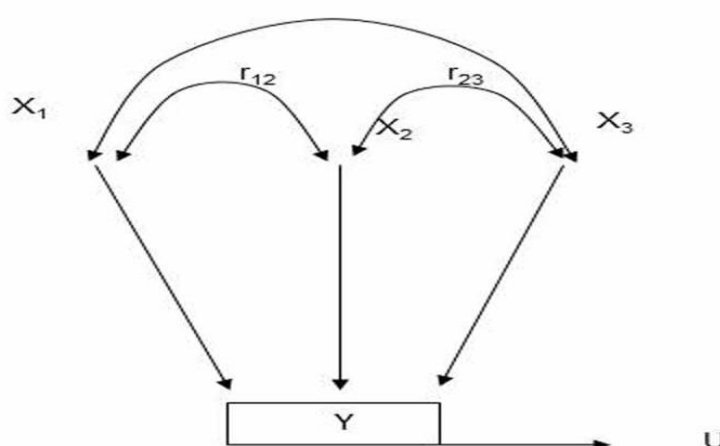
Figure 1: Path Diagram
