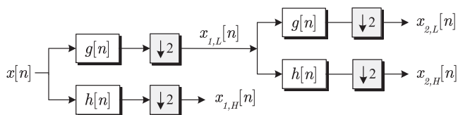
Figure 4 An example structure of 2-level decomposition by discrete wavelet transform.
