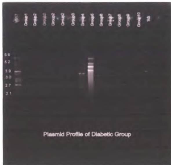
Figure3.17. Agarose gel electrophoresis (0.8% gel) of plasmid DNA showing the plasmid patterns among the representative isolates from 10 ARDRA groups. E. coli V517 was used as reference plasmid marker. The gel was run along with molecular marker of 1 Kb DNA ladder (Bioneer, USA).
