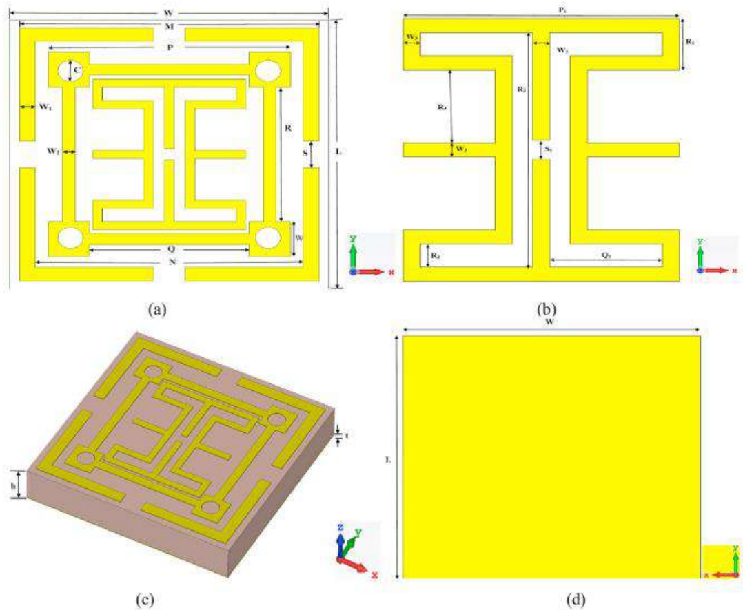
Figure 3 Absorber design
