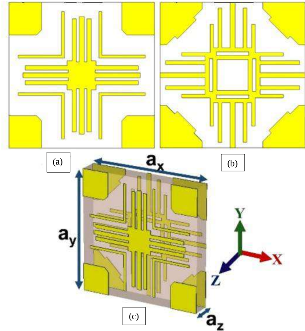
Figure 6 Absorber design
