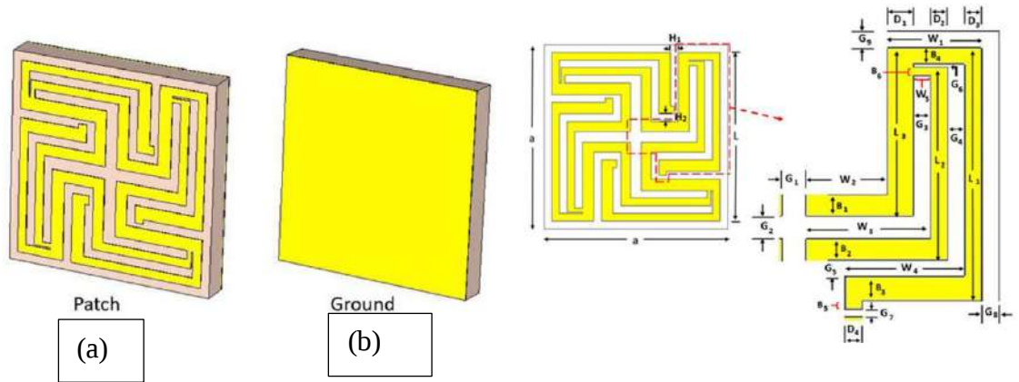
Figure 4 Absorber design
