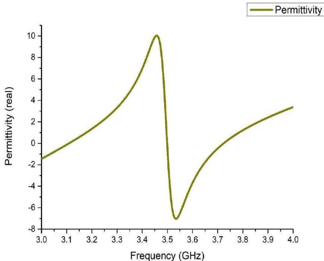
Figure 15: Permittivity
