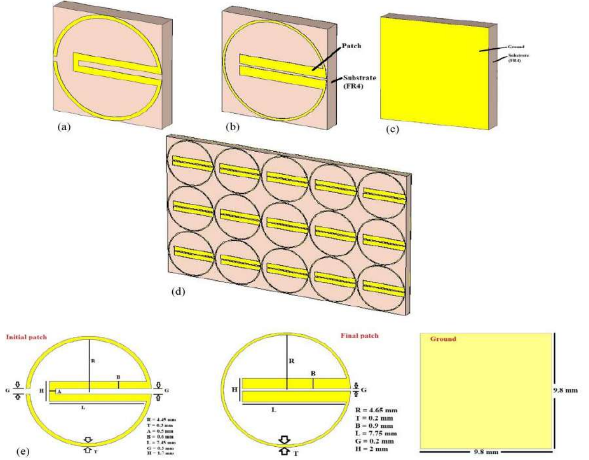
Figure 2 Absorber design
