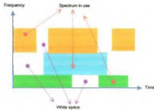
Figure 1.2: Example of spectrum availability [1]
