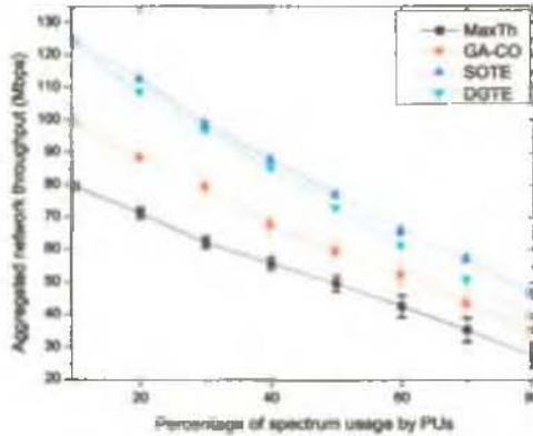
(a) Aggregated network throughput
