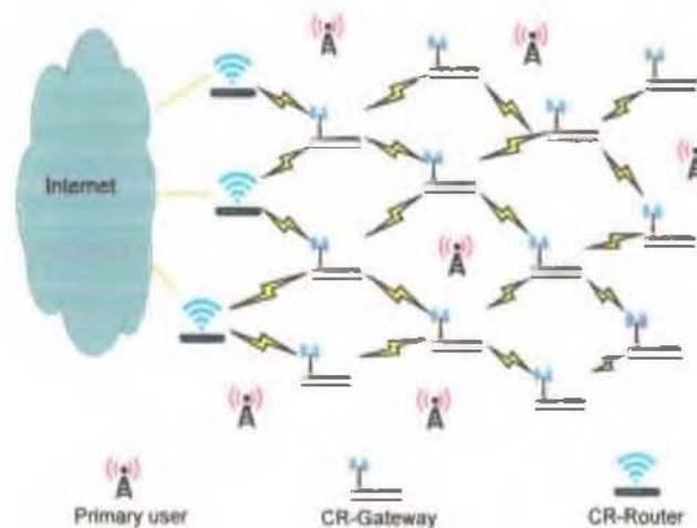
Figure 1.3: CR-WMN architecture
