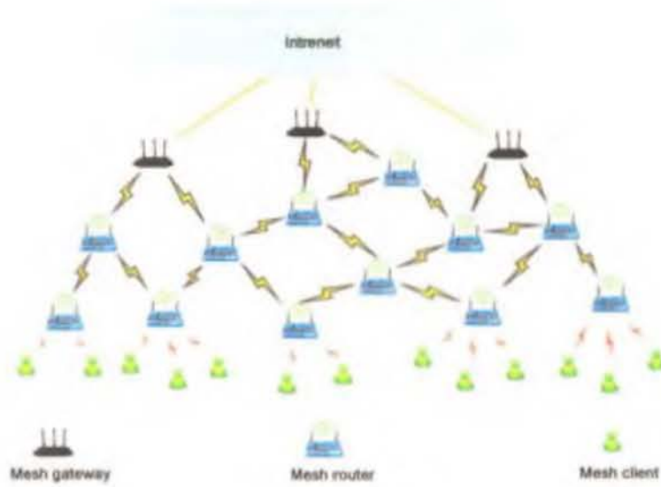
Figure 1.1: WMN architecture
