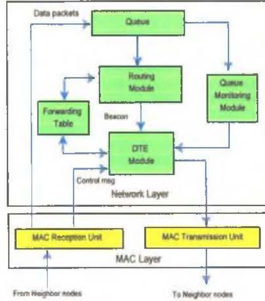
Figure 3.2: DTE component at each router v \in \mathcal{V} in WMNs
