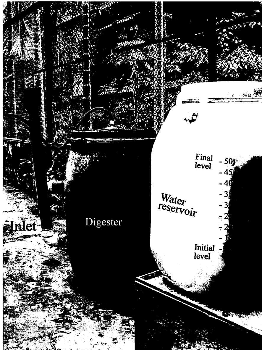
Fig. 2.5. Front view (partially) of the “Mini-Biogas Plant”. The raise of the water level in the translucent plastic reservoir from 16 L up to 52 L mark indicates 36 L of biogas stored in the digester. The 16 L level corresponds to the upper level of substrates in the digester without any gas.
