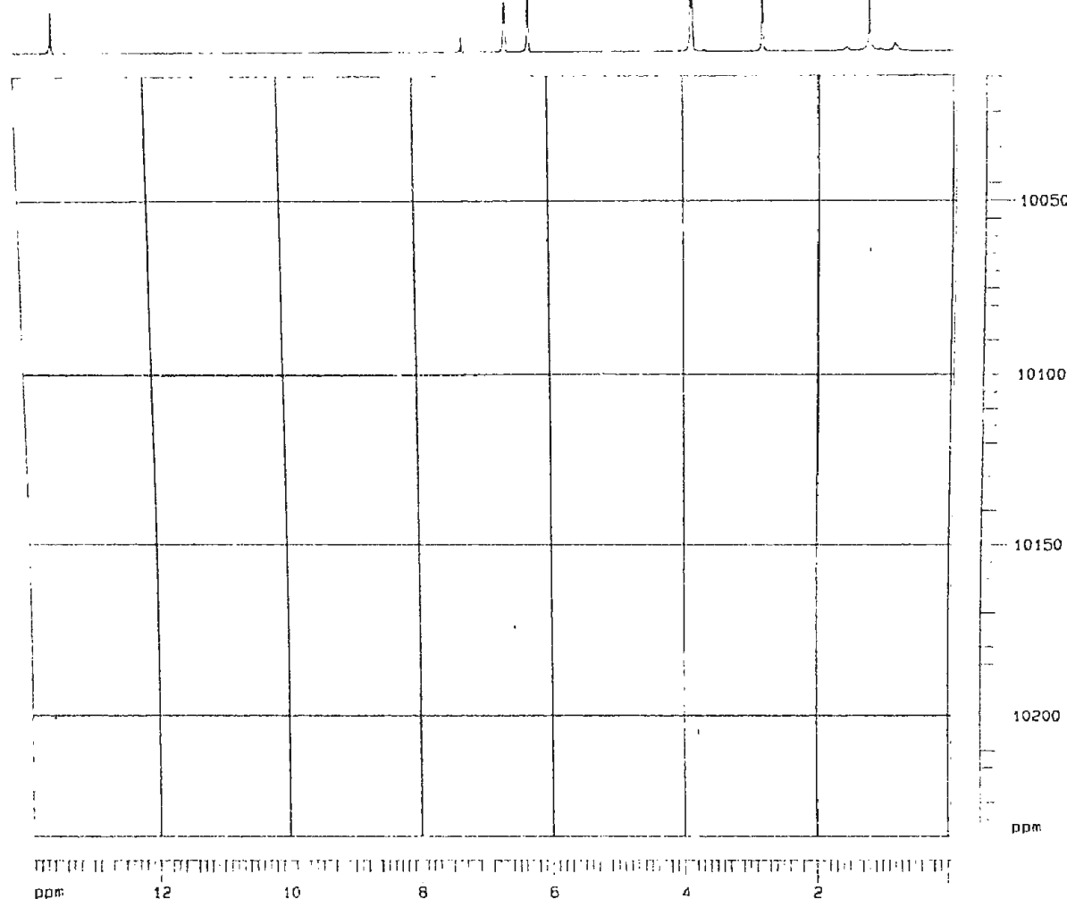
Fig. 18. HSQC spectrum of the compound LMI-1
