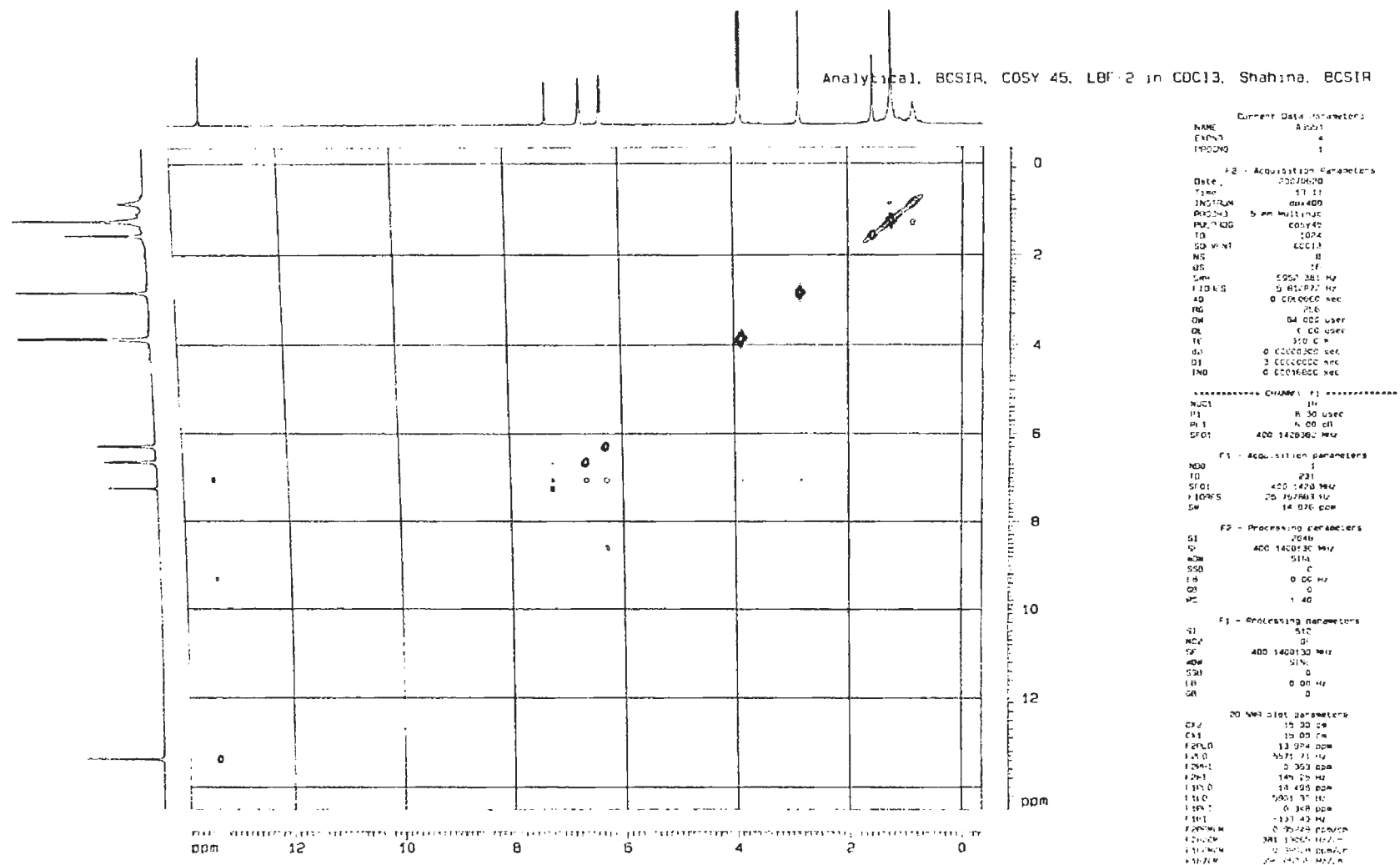
Fig. 24. ^{13}\text{C} -NMR spectrum for COSY of the compound LBF-2
