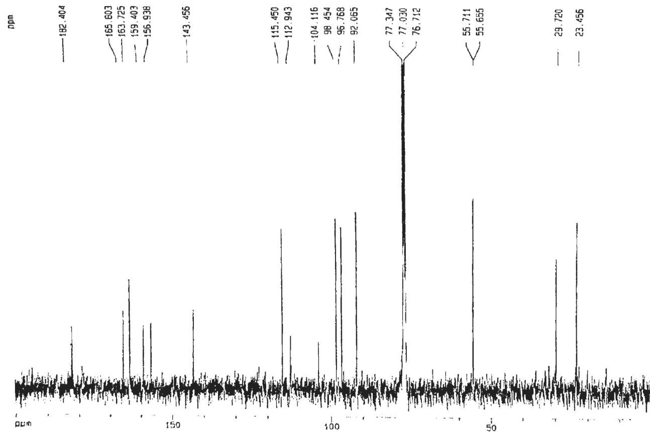
Fig. 21. ^{13}\text{C} -NMR spectrum of the compound LBF-2
