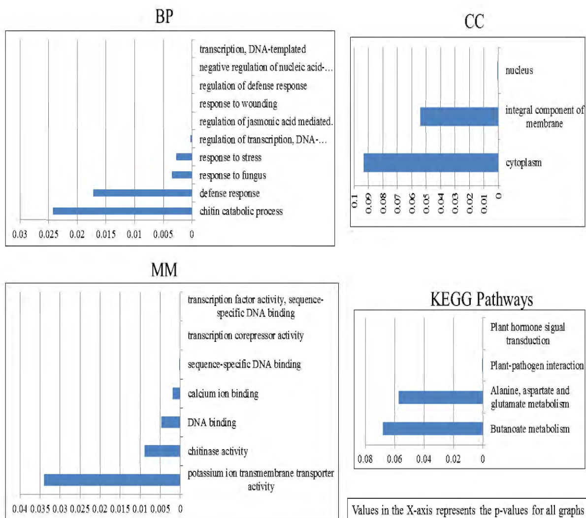
Fig. 3.13. GO analysis and KEGG pathways for classical method genes
