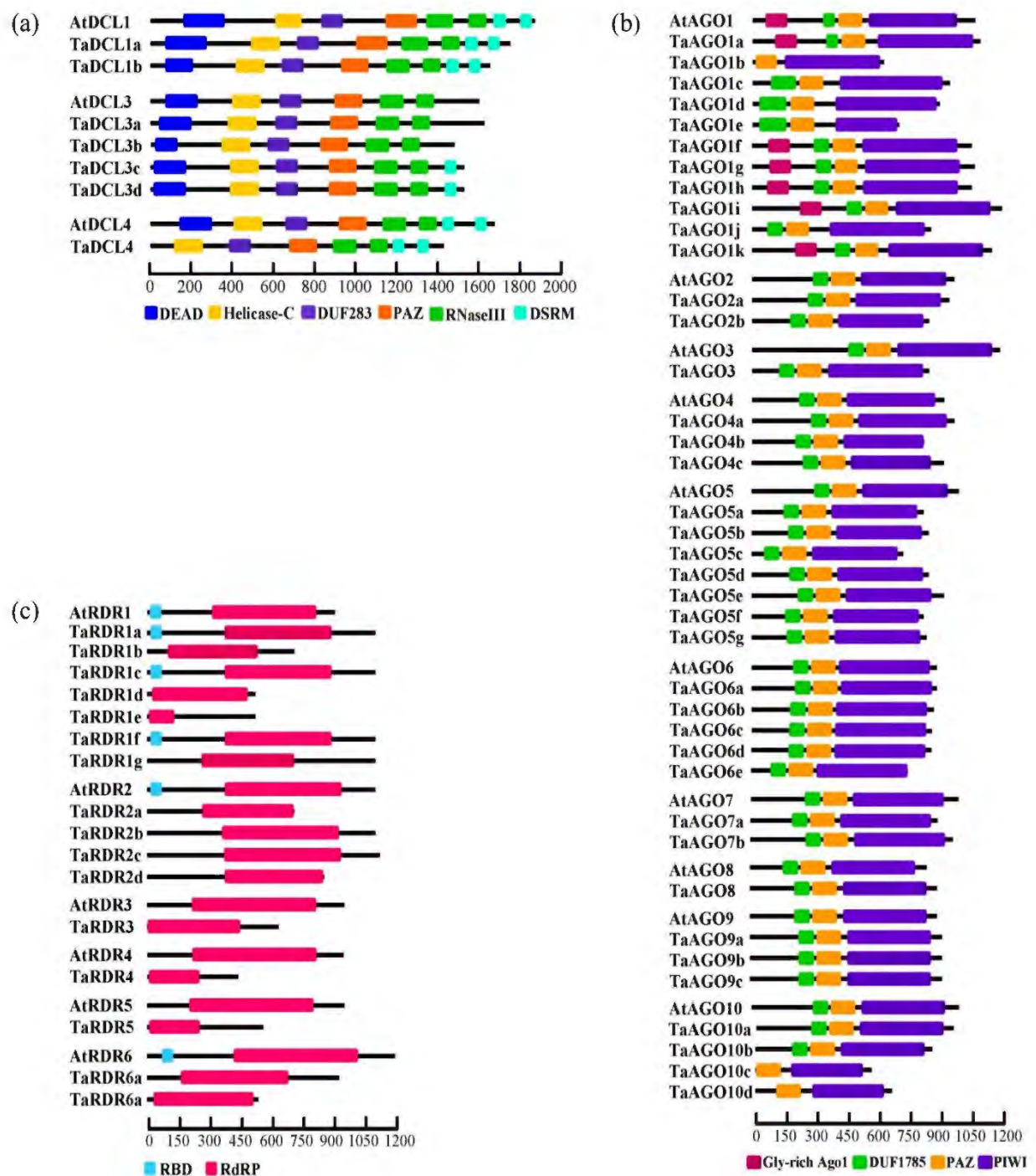
Fig.4.3. Protein structure and functional domain/motifs analysis of (a) DCL (b) AGO (c) RDR in wheat. Domains are indicated as boxes in different colors. The diagrams were drawn to scale.
