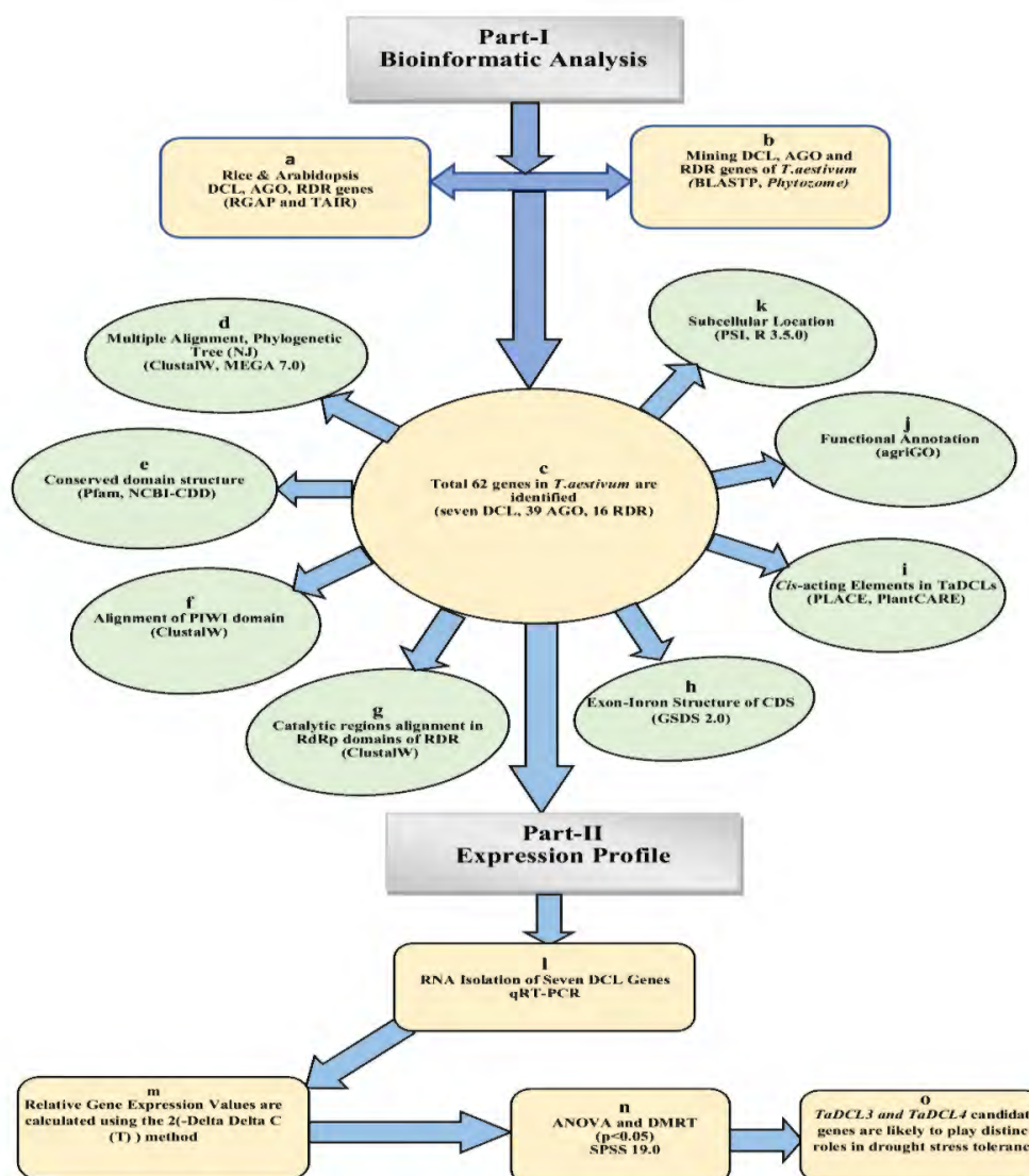
Fig. 4.1 Schematic diagram of the whole work. (a) Rice and Arabidopsis protein sequences were obtained from RGAP and TAIR databases. (b) Arabidopsis protein sequences were used query to find corresponding protein sequences of T.aestivum from Phytozome using BLASTP technique. (c) Total 62 DCL, AGO and RDR genes were identified. (d) Multiple alignment and phylogenetic analysis were carried out using ClustalW and MEGA 7.0 software. (e) Conserved domain structure of each 62 genes were obtained using Pfam and NCBI-CDD database. (f) Obtained alignment profile of PIWI domain of amino acids wheat AGO proteins using ClustalW. (g) Alignment of catalytic regions in RdRp domains of RDR proteins of wheat, rice, and A. thaliana using ClustalW. (h) Exon-intron structure of wheat and A. thaliana DCL, AGO and RDR of full-length coding sequence (CDS) using GSDS 2.0. (i) Estimate of cis-Acting Elements of the promoter regions of the TaDCL Genes were calculated using PLACE and PlantCARE database. (j) Functional annotation/enrichment analysis of wheat DCL, AGO and RDR genes were performed to identify significantly enriched gene ontology and pathway terms. (k) Subcellular locations of each 62 genes were obtained to identify their involvement in metabolism process using PSI. (l) Gene expression analysis of TaDCL genes in leaves, roots and under drought stress following quantitative real time PCR (qRT-PCR) technique. (m) Gene expressions were obtained using 2^{-\Delta\Delta Ct} method. (n) Significant genes were calculated following ANOVA and DMRT ( P < 0.05 ). (o) TaDCL3 and TaDCL4 were significantly induced upon drought treatment and showed higher expression level.
