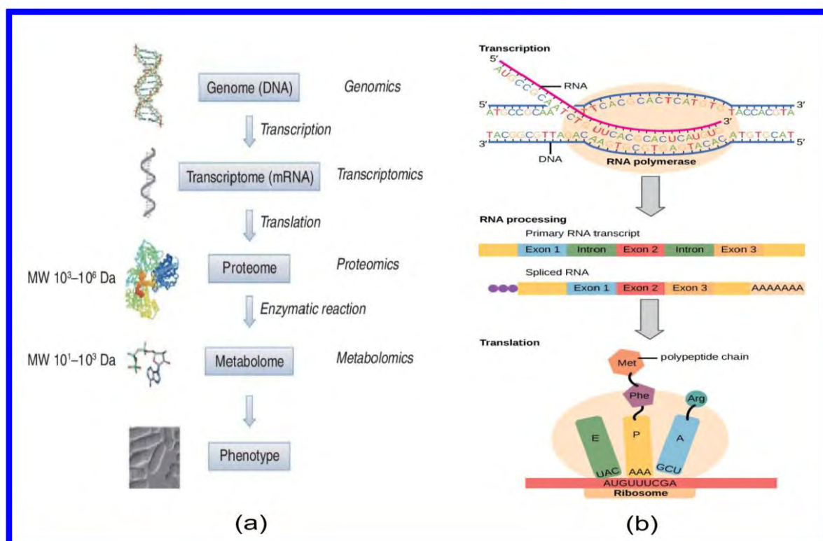
Fig.1.4. (a) The Central dogma of molecule biology and (b) Process of gene expression
