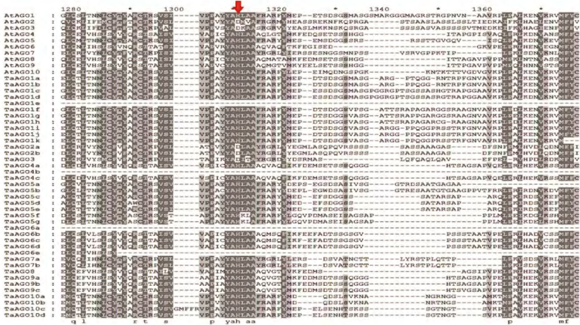
Fig.4.4. Alignment profile of PIWI domain amino acids of wheat AGO proteins. The protein sequences were aligned using MEGA 7.0. The conserved Asp, Asp and His (DDH) trait residues, as well as His (H) are shaded in colors. Amino acid positions corresponding to each protein are indicated at the end of each line.
