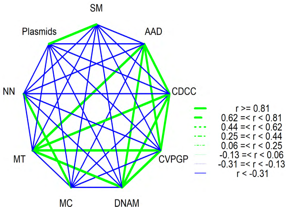
Fig.6.2. Pearson correlation network for nine key functional metagenomes
