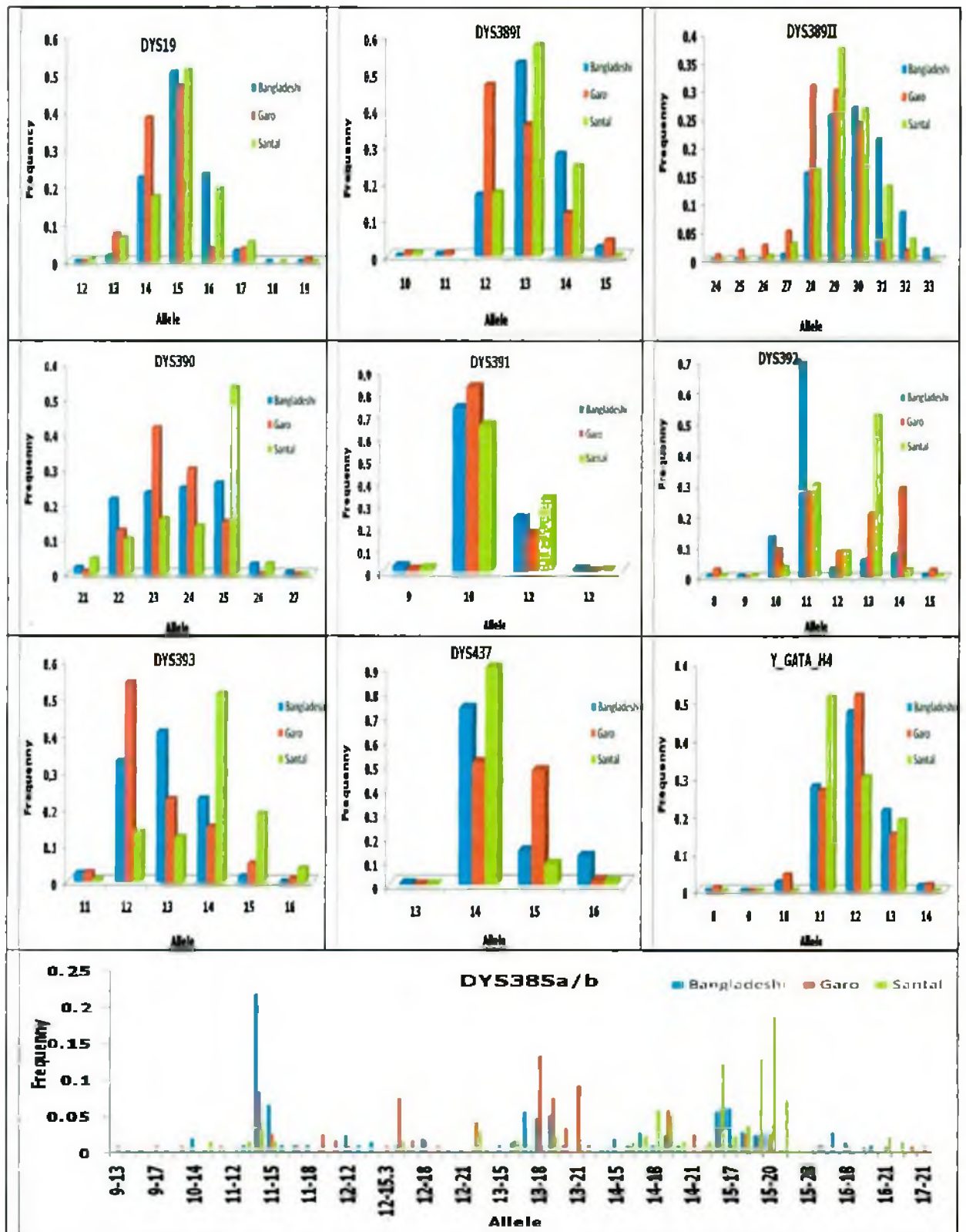
Figure 1.2: Allele frequency distribution of ten Y-STR loci. The figures compared Bangladeshi Bengali, Garo and Santal genetic data.
