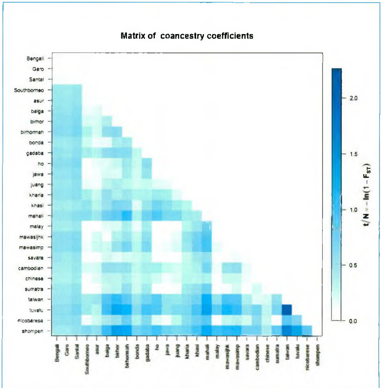
Figure 1.10: Matrix of co-ancestry coefficients indicates the relationship between different populations: Lower the co-ancestry coefficient means closer the two populations. Results showed that co-ancestry coefficients among Garo, Chinese and Cambodian populations ranges from about 0.2 to 0.5, which means that Garo, Chinese and Cambodian populations are closely related to each other. On the other hand, Santal, Malay and Khasi population ranges from about 0.5 to 0.6 means these three populations are closely related to each other.
