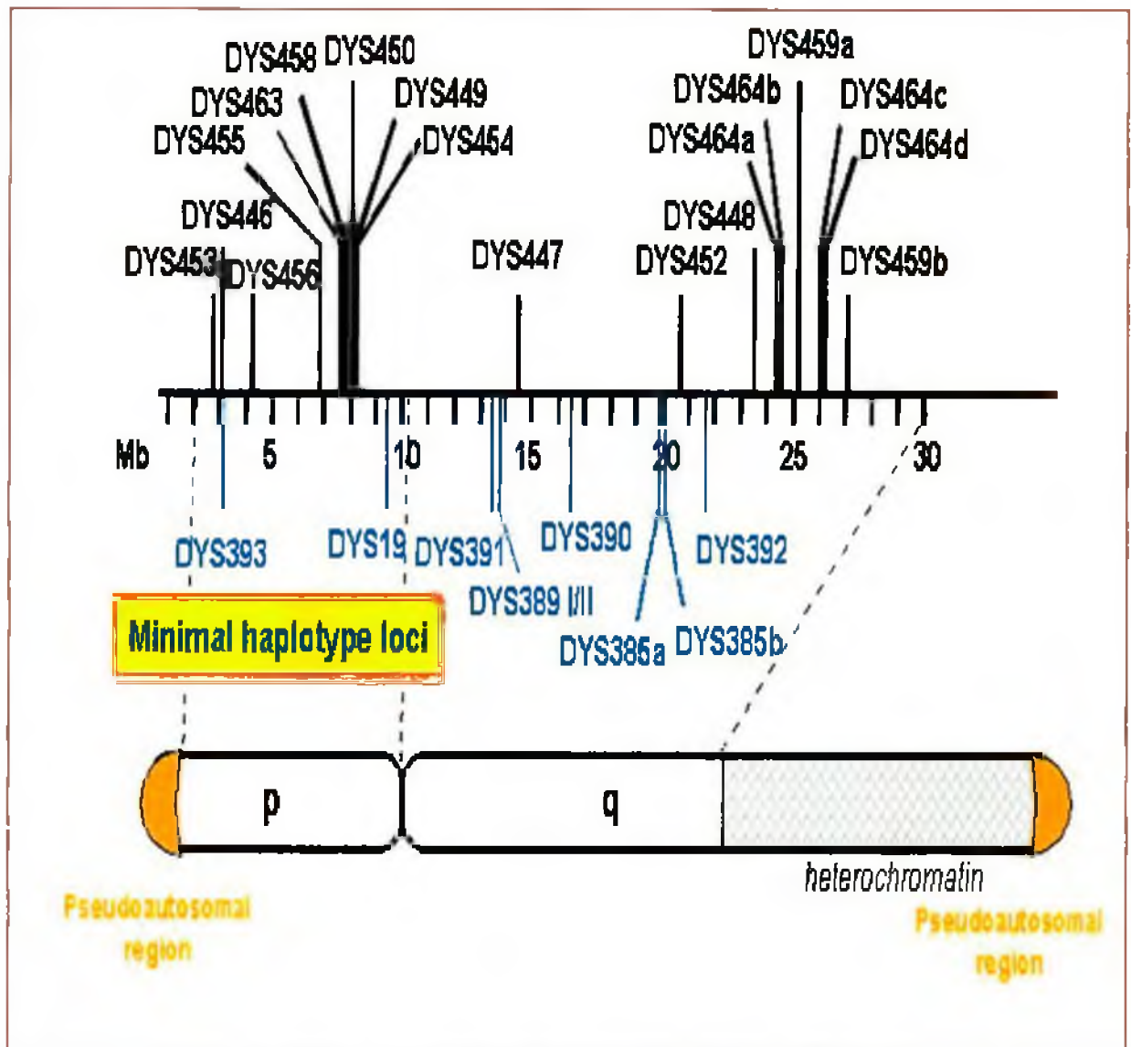
Figure 1.1: Chromosomal locations for commonly used and new Y-STR markers (Michael Hammer, 2002).
