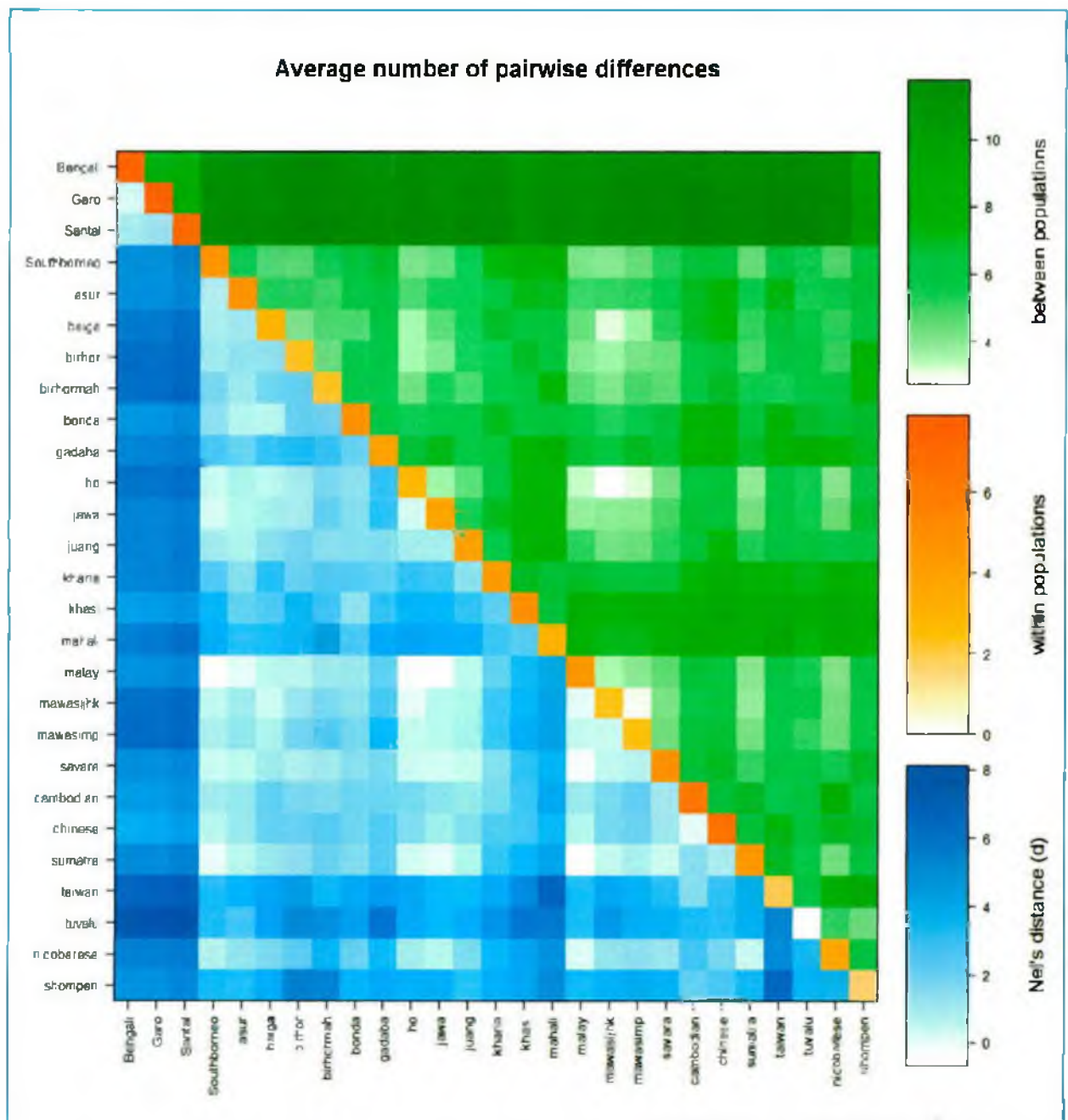
Figure 1.11: Average number of pairwise differences indicates the relationship between different populations: The Nei's distance indicates that Garo, Chinese and Cambodian populations are closely related. On the other hand, Santal, Malay and Khasi population are closely related to each other.
