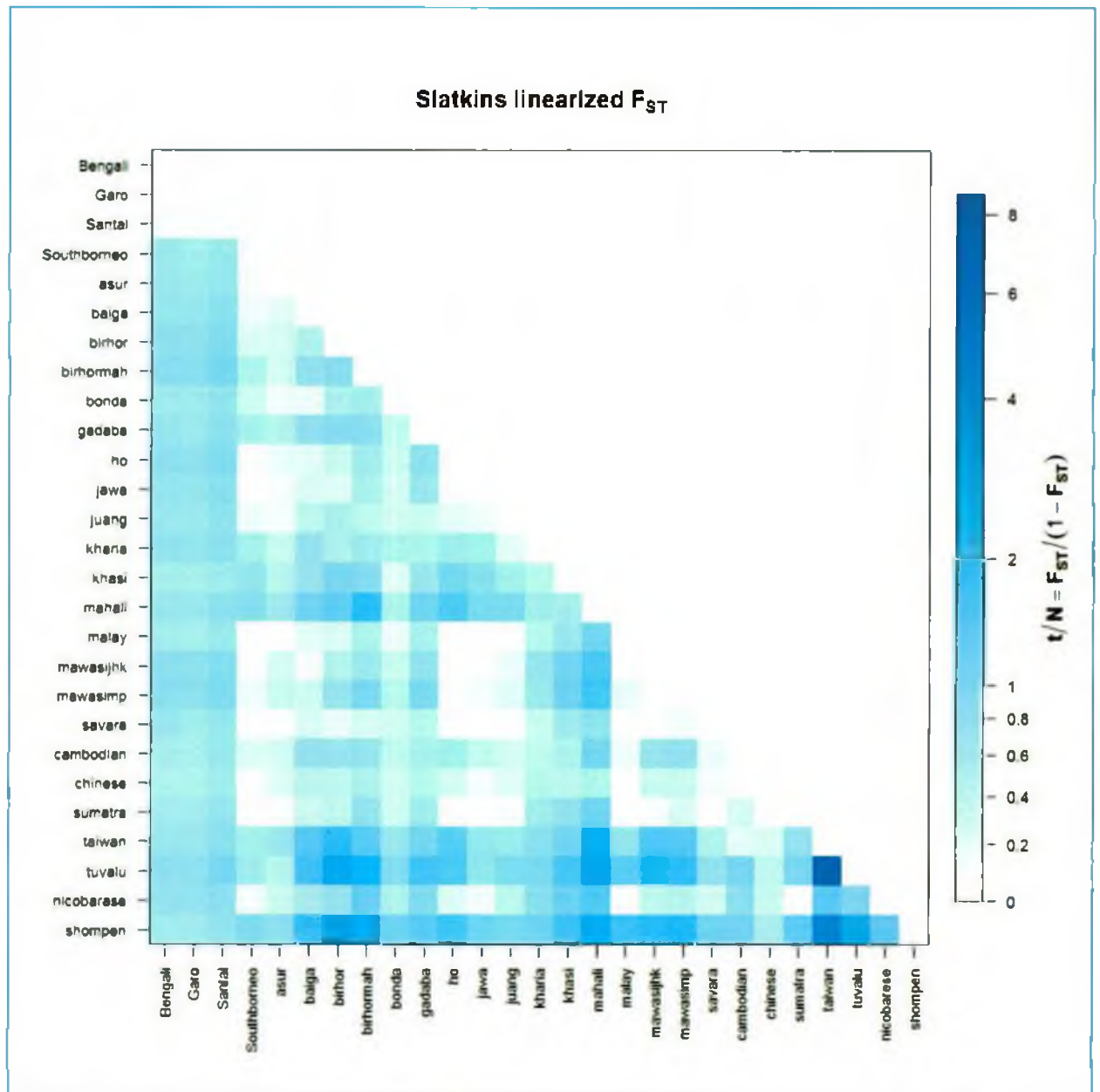
Figure 1.9: Slatkins Linearized F_{ST} value indicates short-term genetic distances between populations: Lower the Slatkins Linearized F_{ST} value, closer the two populations. Results indicates that the Slatkins Linearized F_{ST} value among Garo, Chinese and Cambodian population is ranges from 0.4 to 0.6, which means that these three populations are closely related to each other. On the other hand, Santal, Malay and Khasi population ranges from about 0.5 to 0.7, which means these three populations are closely related to each other.
