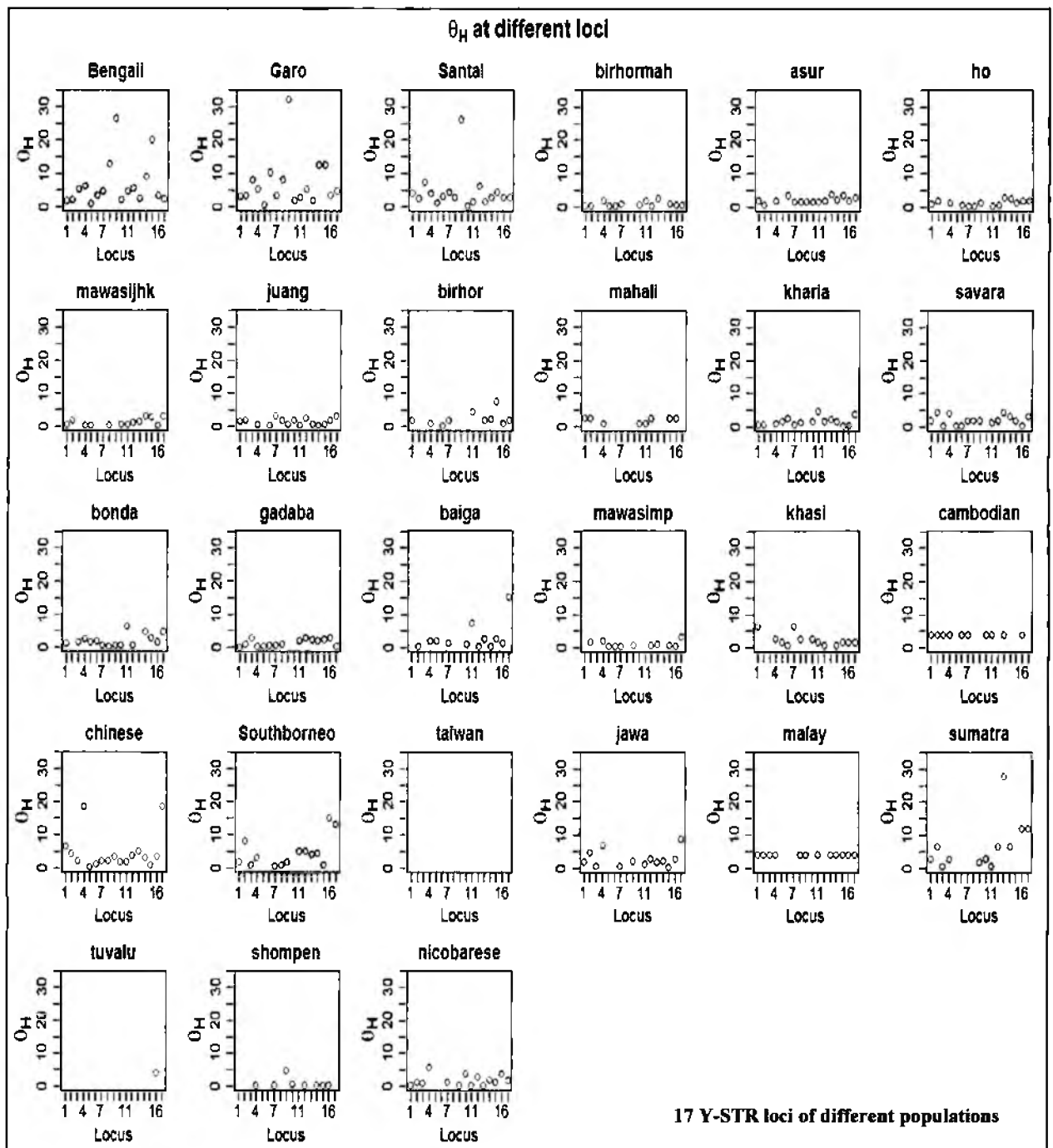
Figure 1.14: Molecular distance at different loci ( \theta_H ) indicates the molecular distance among various populations based on expected heterozygosity: \theta_H value of most of the loci indicates Santal and Khasi populations are closely related. On the other hand, Garo, Chinese and Cambodian populations have close relationship.
