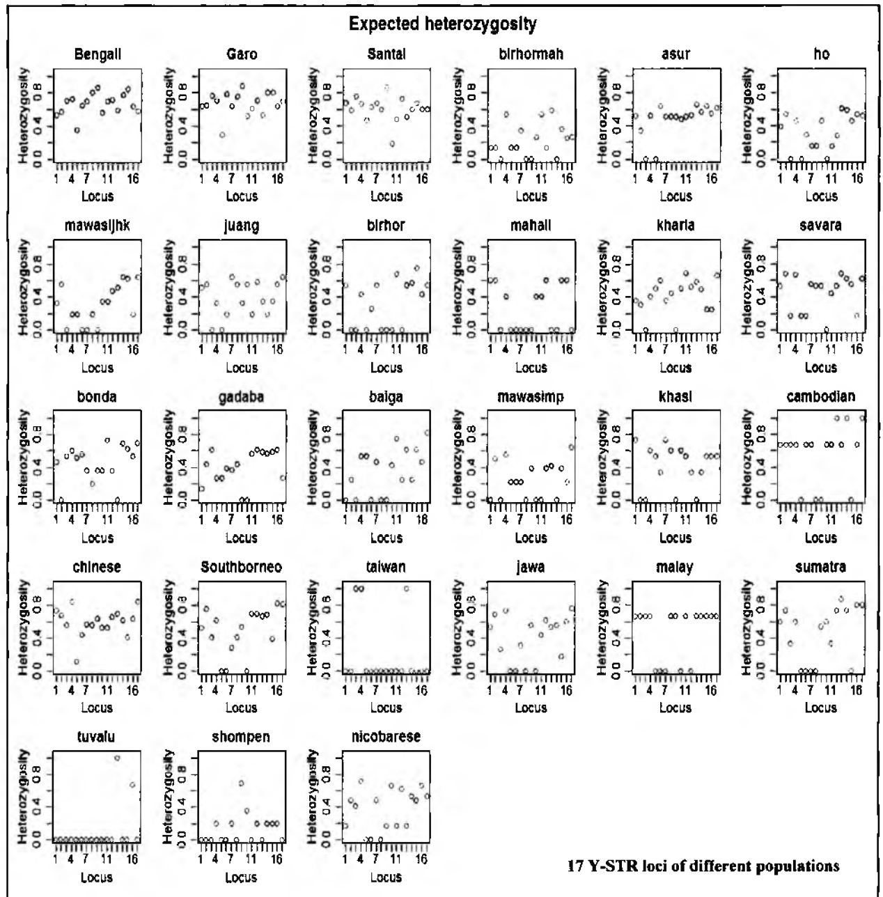
Figure 1.13: Expected heterozygosity indicates the closely relationship between different populations: Expected heterozygosity of most of the loci showed that Garo, Chinese and Cambodian populations have close relationship. Results also indicated that Garo is closely related to Bangladeshi mainstream population. On the other hand, results showed that Santal and Khasi populations are closely related.
