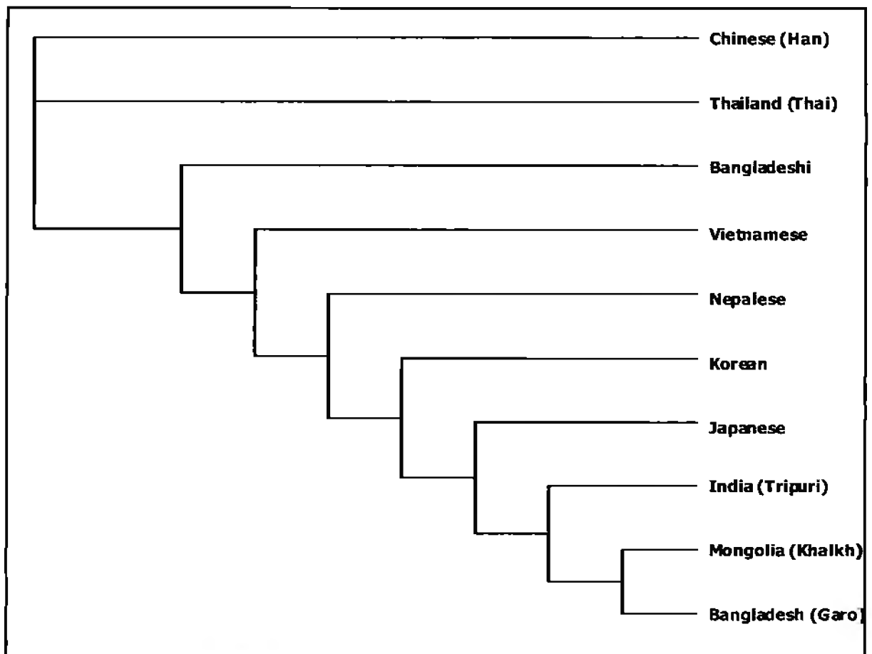
Figure 1.4: Neighbor-Joining tree structure from pairwise genetic distance ( \Phi_{st} value) between Garo population (Bangladesh) and Nine Asian population
