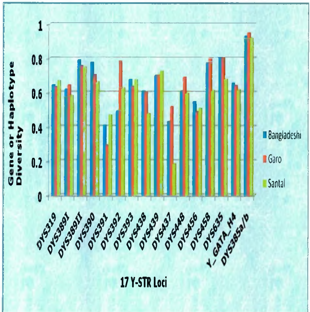
Figure 1.3: Comparison of Gene or Haplotype diversity among three population groups of Bangladesh (Bangladeshi, Garo and Santal)
