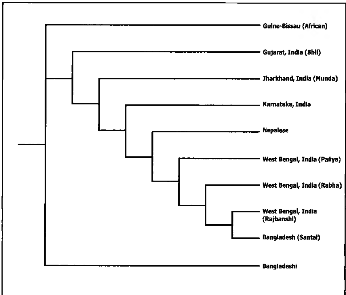
Figure 1.5: Neighbor-Joining tree structure from pairwise genetic distance ( \Phi_{st} value) between Santal (Bangladesh) and Eight Asian and One African population
