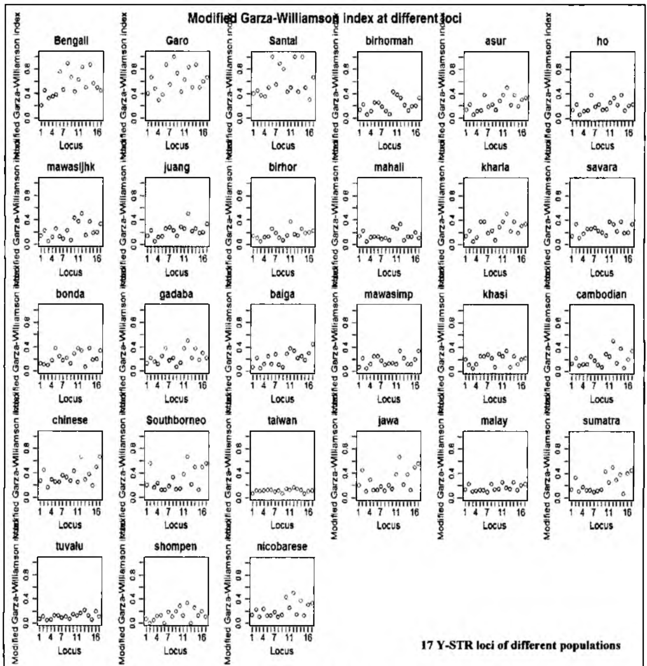
Figure 1.15: Modified Garza-Williamson index at different loci indicates the molecular distance among different populations: Modified Garza-Williamson value of Santal and Nicobarese population ranges from 0.4 to 0.9 means they are closely related. On the other hand, Garo and Chinese population ranges from 0.3 to 0.9 means close relationship between Garo and Chinese population.
