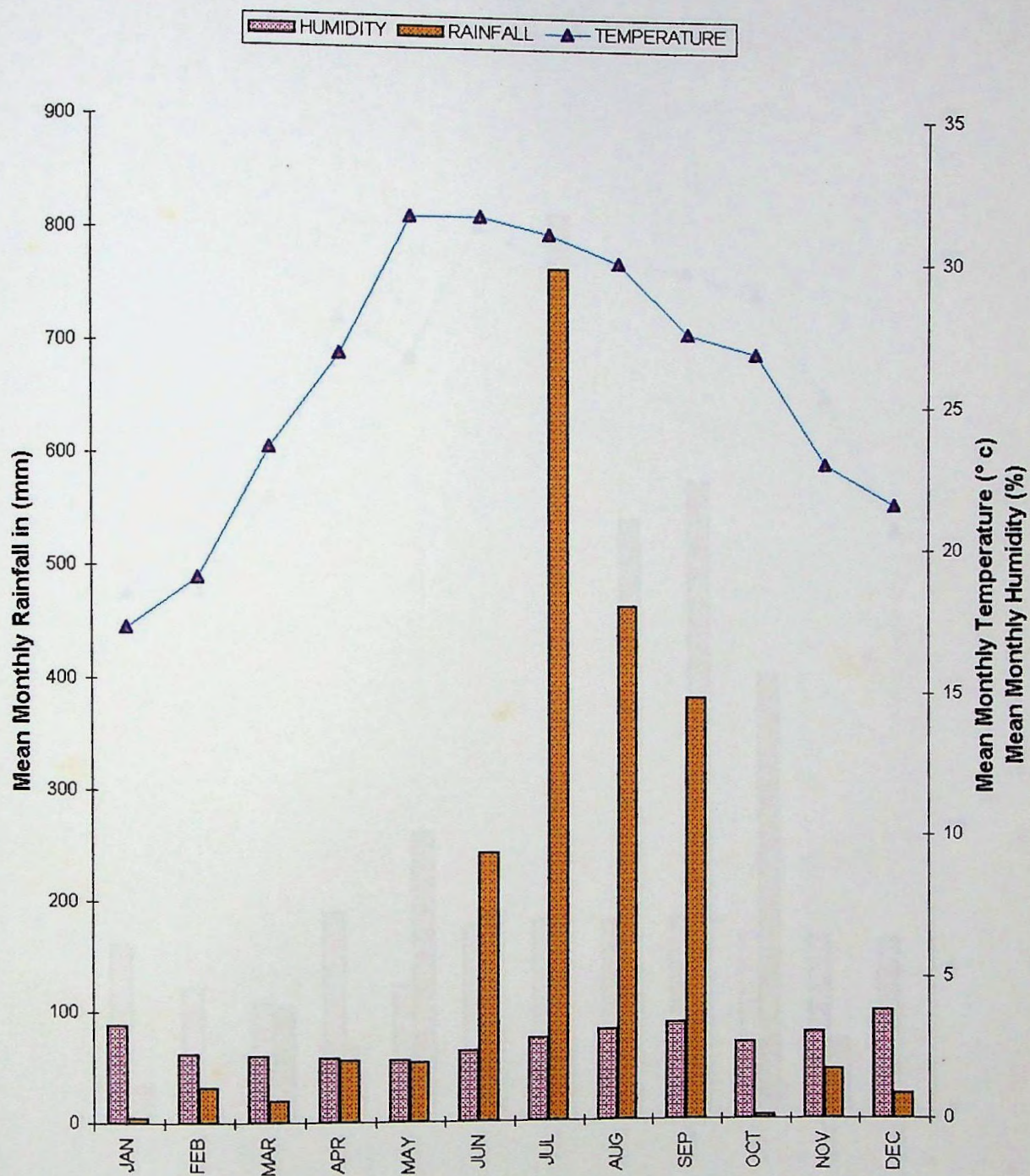
Fig.12 Climatic Diagram for Rajshahi
