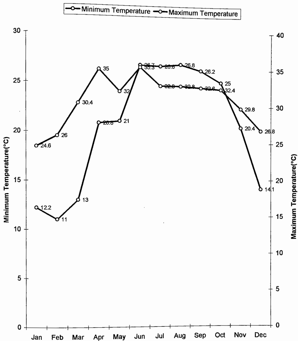
Fig.23 Graphical representation of Maximum and Minimum Temperature
