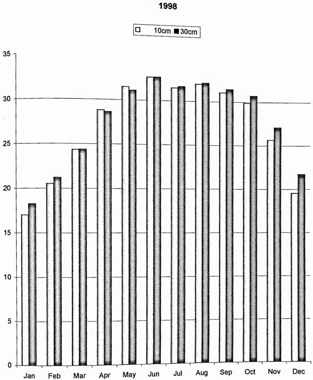
Fig. 43 Graphical representation of Soil Temperature (°C)
