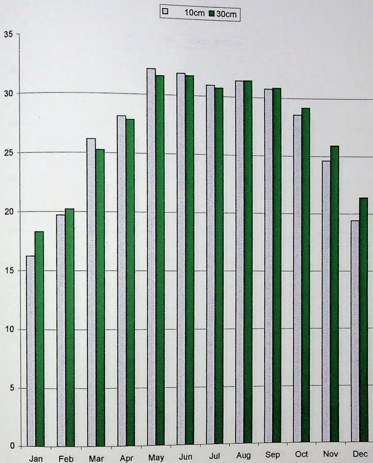
Fig. 42 Graphical representation of Soil Temperature (°C)
