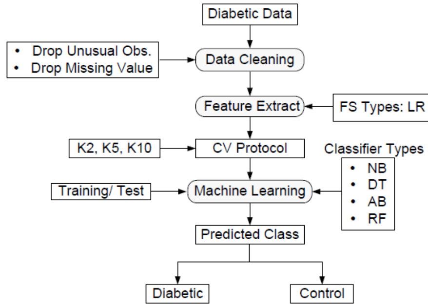
Figure 4.1. Overview of the proposed ML-based framework.
