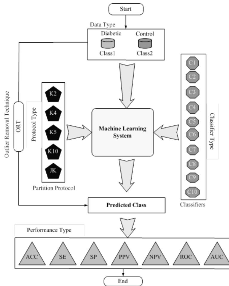
Figure 5.3. Performance of the ML-based system in the presence and absence of outliers.
