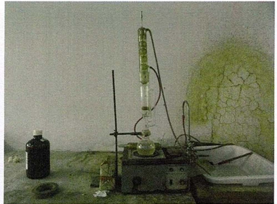
Soxhlet apparatus (Fat)
