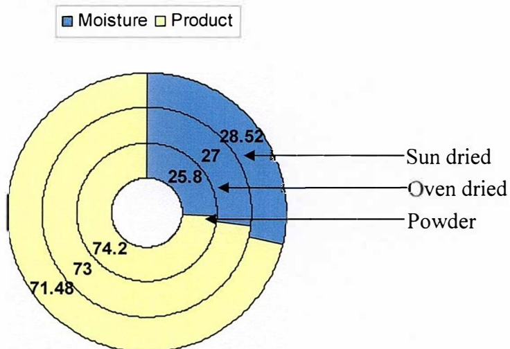
Fig. 3.7. Doughnut diagram showing the moisture content of sun dried fish, oven dried fish and powder production of C. soborna .
