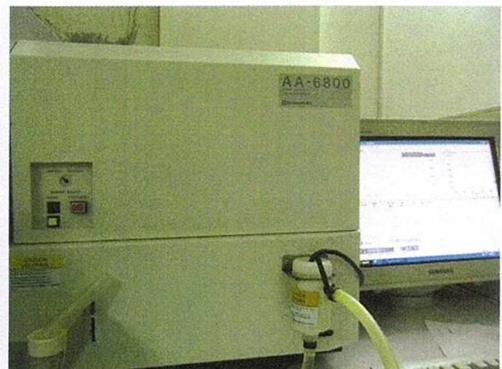
Atomic absorption spectrophotometer (calcium and iron)
