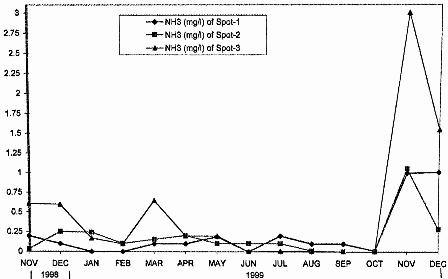
FIGURE NO. 17 : MONTHLY VARIATION OF AMMONIA VALUE OF THREE SAMPLING SPOTS.
