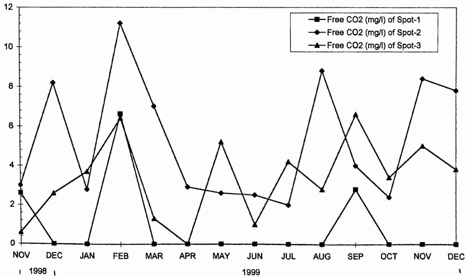
FIGURE NO. 8 : MONTHLY VARIATION OF FREE CARBON DI OXIDE VALUE OF THREE SAMPLING SPOTS.
