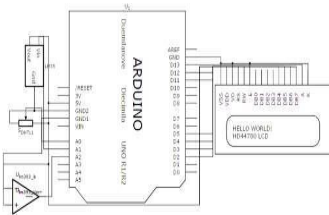
Fig 2.4 Circuit Diagram of Arduino Uno Based Weather Monitoring System [7].
