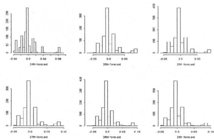
Figure 6.18: Histogram of the bootstrap forecast replicates for GDP per capita in transformed metric. Classical estimate of \theta is used for data generation process (DGP).
