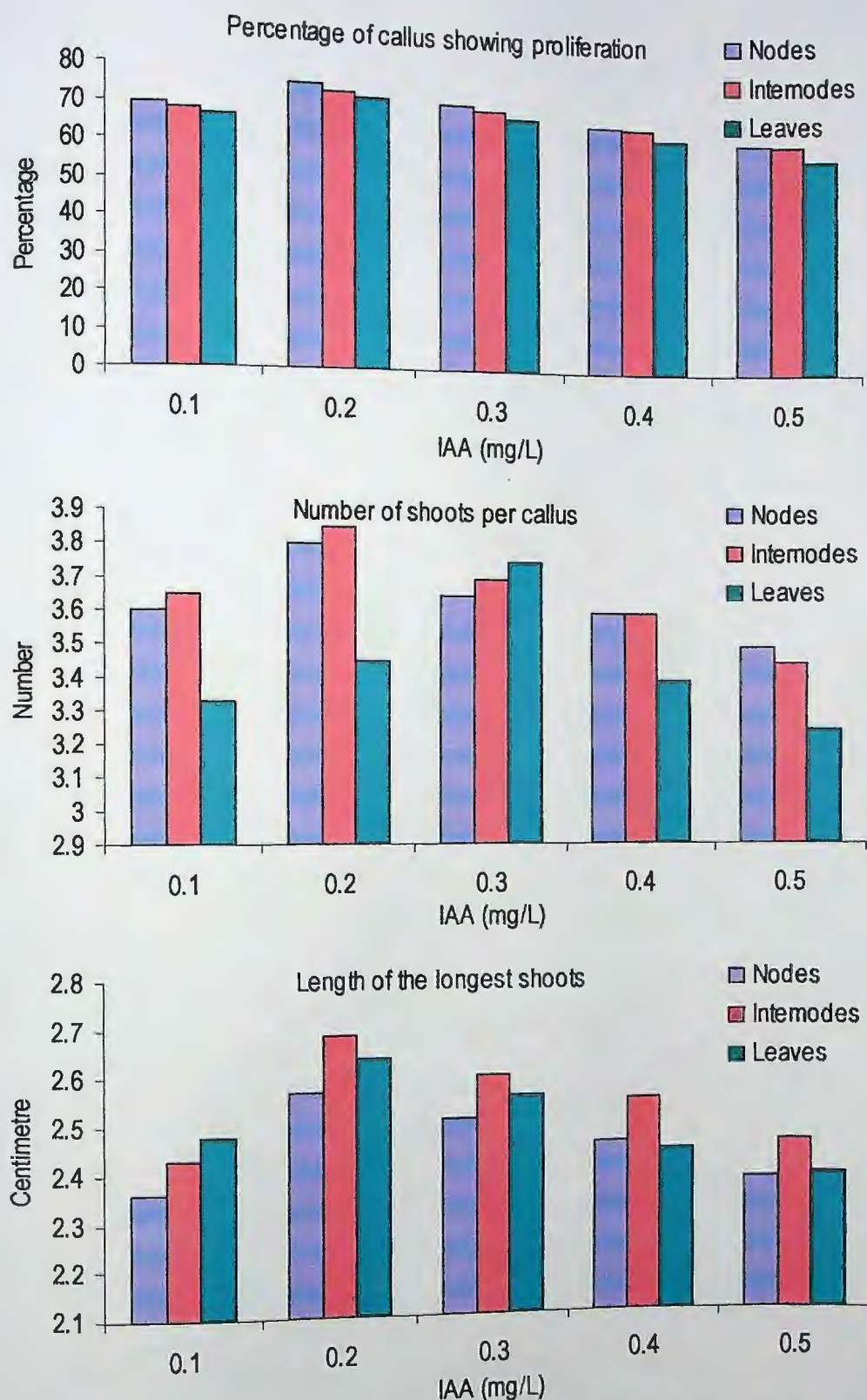
Fig. 28. Effects of BAP (2.0 mg/l) with different concentration of IAA on indirect shoot proliferation from callus of the different explants of Stevia rebaudiana ; percentage proliferation (upper), number of shoots per callus (middle), length of longest shoot (lower).
