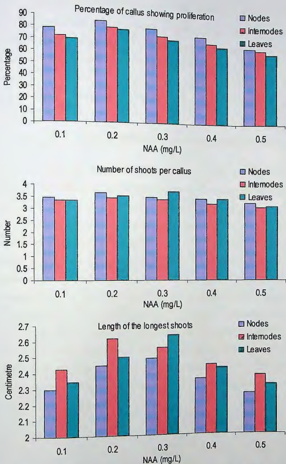
Fig. 37. Effects of BAP (2.5 mg/l) with different concentration of NAA on indirect shoot proliferation from callus of the different explants of Stevia rebaudiana ; percentage proliferation (upper), number of shoots per callus (middle), length of longest shoot (lower).
