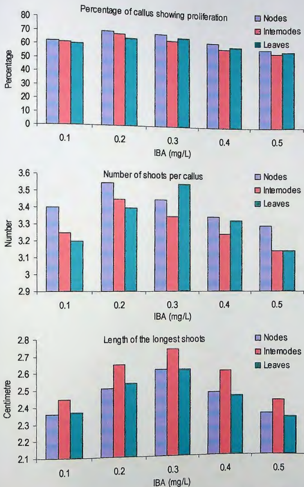
Fig. 31. Effects of BAP (1.5 mg/l) with different concentration of IBA on indirect shoot proliferation from callus of the different explants of Stevia rebaudiana ; percentage proliferation (upper), number of shoots per callus (middle), length of longest shoot (lower).
