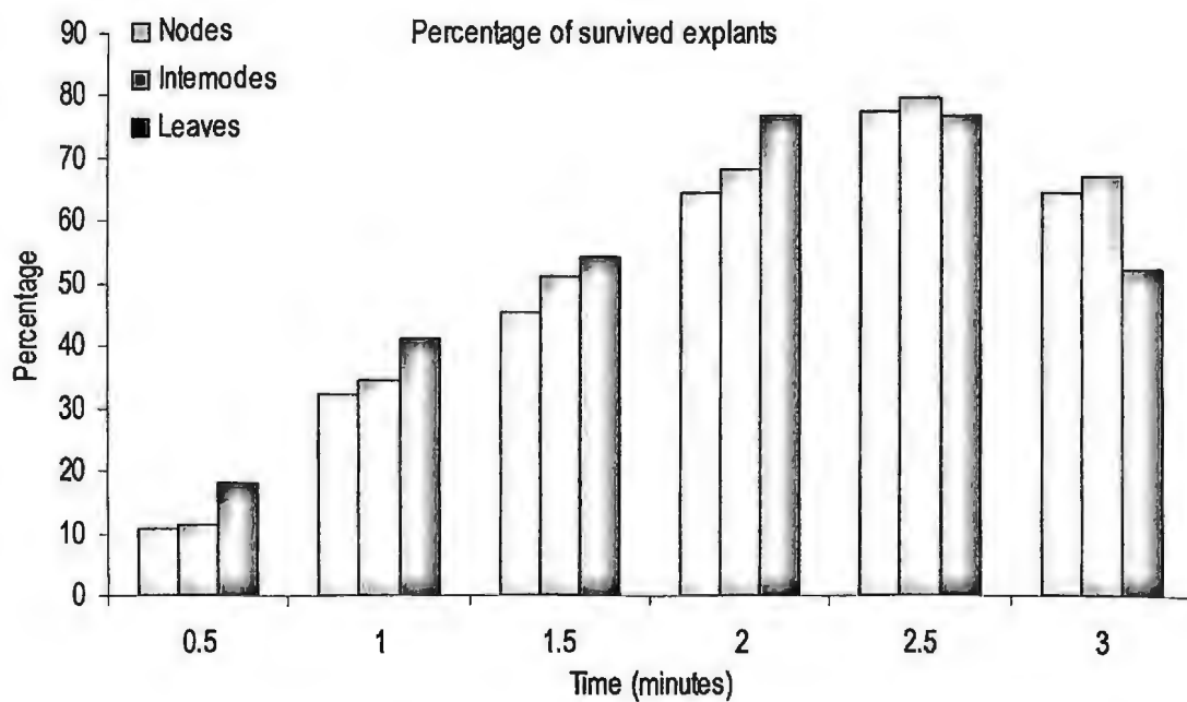
Fig. 2. Effects of \text{HgCl}_2 (0.1%) treatment for different duration of times on surface sterilization of the different explants of Stevia rebaudiana ; percentage of free contamination (upper) and percentage of survived explants (lower).
