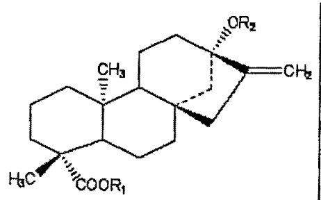
Fig. 1. Structures of diterpene glycosides
