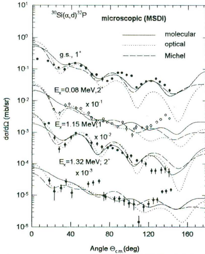
Fig. 5. 47. Comparison of the zero-range microscopic DWBA calculations using the MSDI spectroscopic amplitudes and the molecular, normal optical and Michel potentials in the \alpha -channel for the ^{30}\text{Si}(\alpha, d)^{32}\text{P} reactions at 25 MeV leading to the ground ( 1^+ ), 0.08 ( 2^+ ), 1.15 ( 1^+ ), and 1.32 ( 2^+ ) MeV states of ^{32}\text{P} to the differential cross-section data. The solid, dotted and broken curves are the predictions using the molecular, normal optical and Michel potentials respectively. Data are from [48].
