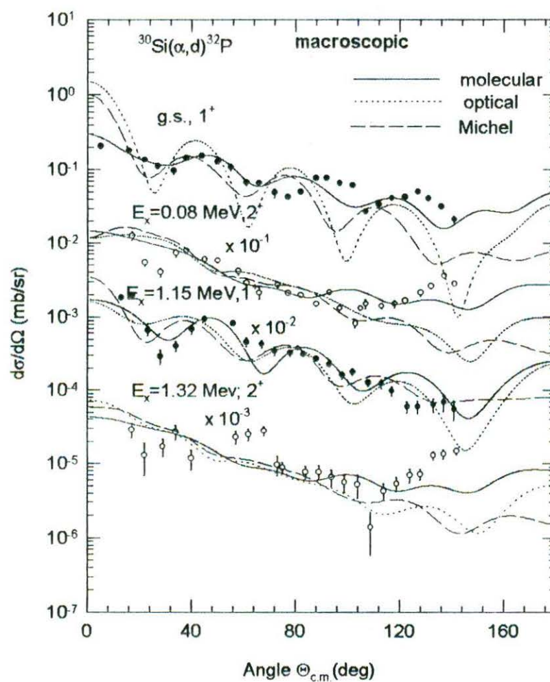
Fig. 5. 38. Comparison of the full finite-range macroscopic DWBA calculations for the ^{30}\text{Si}(\alpha, d)^{32}\text{P} reaction at 25 MeV leading to ground ( 1^+ ), 0.08 ( 2^+ ), 1.15 ( 1^+ ), and 1.32 ( 2^+ ) MeV states of ^{32}\text{P} to the differential cross-section data. The solid, dotted and broken curves are the predictions using the molecular, normal optical and Michel \alpha - ^{29}\text{Si} potentials respectively. Data are from [48].
