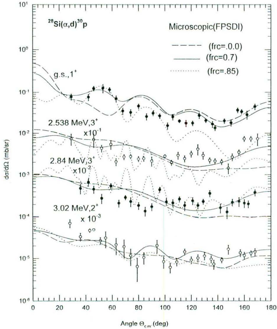
Fig. 5. Comparison of the zero-range microscopic DWBA calculations using the FPSDI spectroscopic amplitudes and the molecular potential in the \alpha -channel for the ^{28}\text{Si}(\alpha, d)^{30}\text{P} reaction at 26 MeV leading to the ground ( 1^+ ), 2.538( 3^+ ), 2.84( 3^+ ) and 3.02 ( 2^+ ) MeV states of ^{30}\text{P} to the differential cross-section data. The solid curves are the predictions using the finite-range (FR) correction with FR parameter R=0.7 fm. The broken and dotted curves are the predictions with R=0.0 and 0.85 fm, respectively. The data are from [17].
