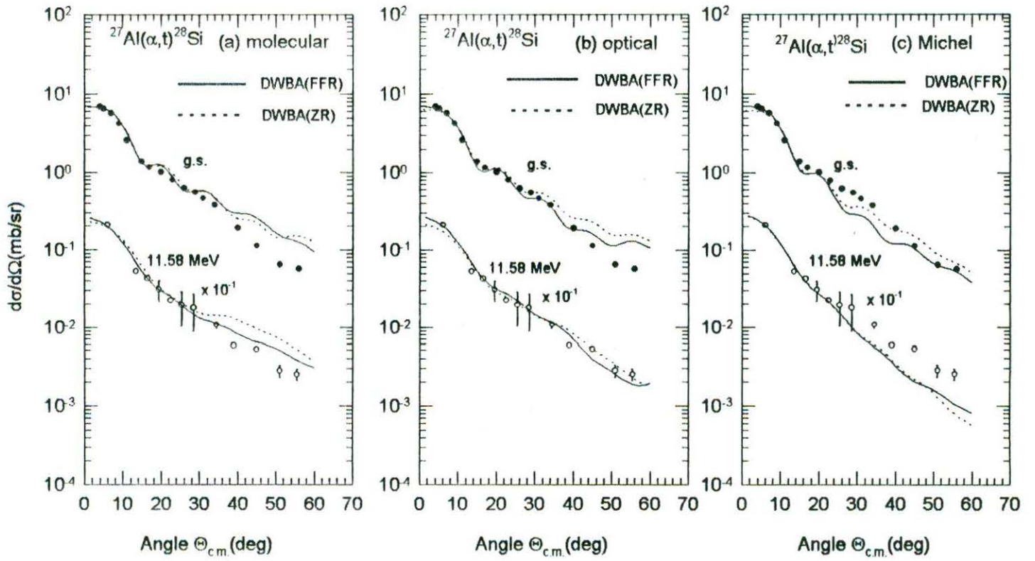
Fig. 5.3. Full finite-range ( solid curves) and zero-range ( dotted curves ) DWBA predictions using (a) molecular, (b) normal optical, and (c) Michel potentials for the g.s. and E_x=11.58 MeV transitions are compared to data. Data are from Yasue et al. [ 44 ]
