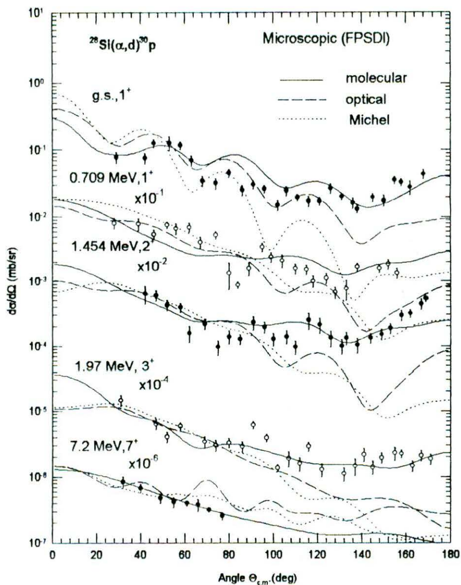
Fig. 5.17. Comparison of zero-range microscopic DWBA calculations with FR correction for the ^{28}\text{Si}(\alpha, d)^{30}\text{P} reaction at 28 MeV leading to the ground ( 1^+ ), 0.709( 1^+ ), 1.454( 2^+ ), 1.93( 3^+ ), and 7.20 ( 7^+ ) MeV states of ^{30}\text{P} to the differential cross-section data. The solid, broken and dotted curves are the predictions using the molecular, optical and Michel \alpha - ^{28}\text{Si} potentials, respectively. Data are from [18]
