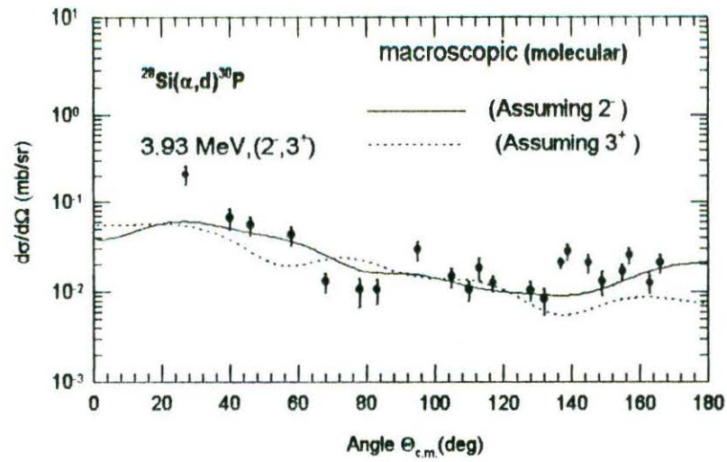
Fig.5.15. Full finite-range macroscopic DWBA calculations using the molecular \alpha - ^{28}\text{Si} potential for the 3.93 MeV state assuming the spin-parity J^\pi = 2^- (solid curve) and 3^+ (dotted curves) are compared to the data. Data are from [18]
