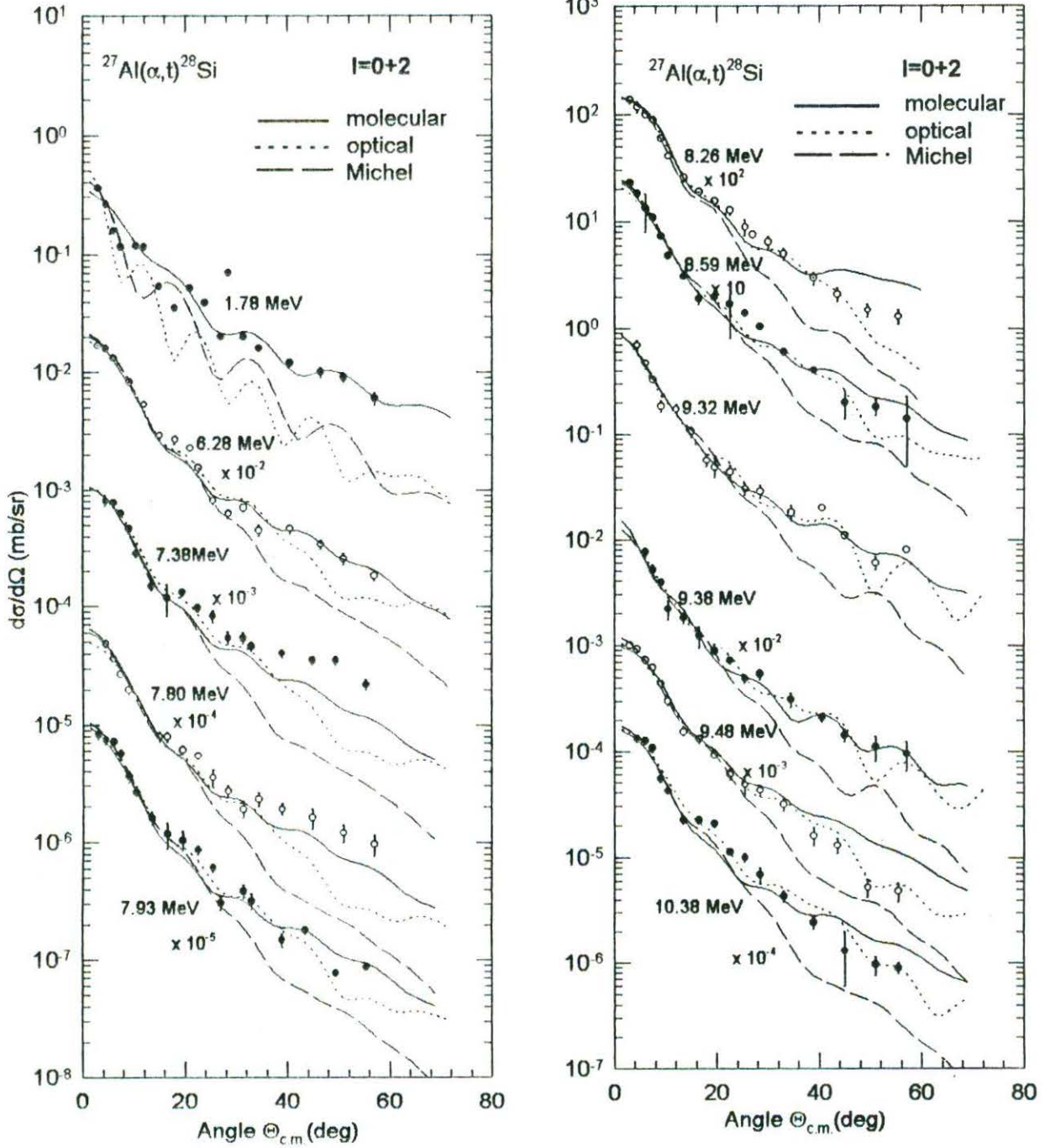
Fig. 5.7. Incoherent sums of full finite-range DWBA predictions using molecular ( solid curves ), normal optical (dotted curves), and Michel ( dashed curves ) potentials for the transitions with I values indicated are compared to data ( filled or open circles). Data are from Yasue et al. [44].
