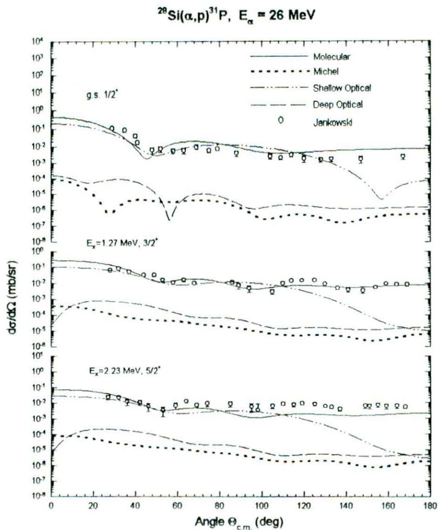
Fig. 5. 49. Zero-range DWBA predictions are compared to the angular distribution of cross-sections for the ^{28}\text{Si}(\alpha, p)^{31}\text{P} reaction at 26 MeV leading to the ground( 1/2^+ ), 1.27 ( 3/2^+ ), and 2.234 ( 5/2^+ ) MeV states. Solid, dotted, dashed and dash-dotted curves are the predictions for the molecular, Michel, deep and shallow normal optical potentials respectively, in the \alpha -channel. Data are from [18].
