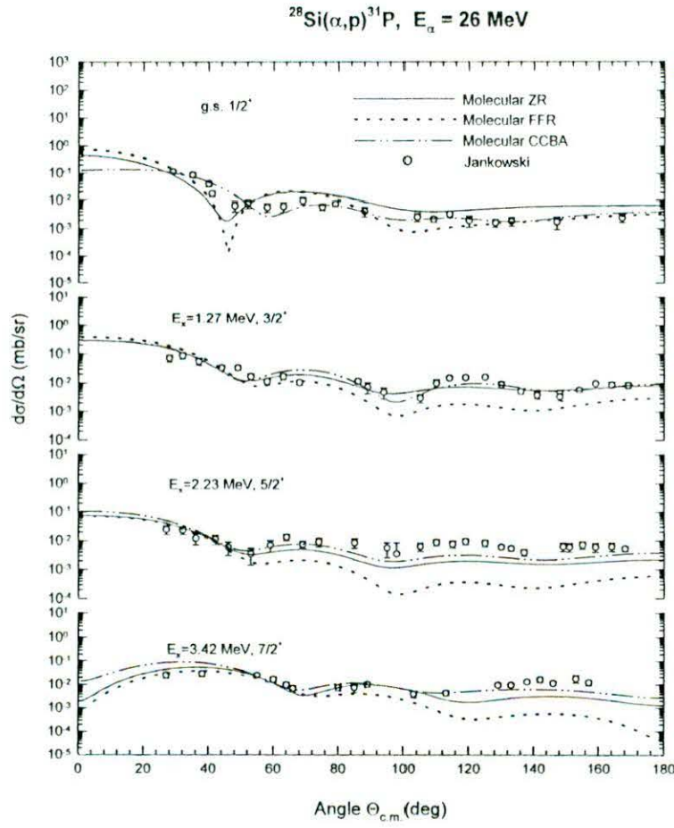
Fig.3. Zero-range (solid), full finite-range(dotted lines) and CCBA (dashed lines) predictions of the transfer reaction using the molecular potential are compared to the data for the ^{28}\text{Si}(\alpha, p)^{31}\text{P} reaction at 26 MeV leading to the ground ( 1/2^+ ), 1.27 ( 3/2^+ ), 2.23 ( 5/2^+ ), 3.42 ( 7/2^+ ) MeV states. The data are from [14].
