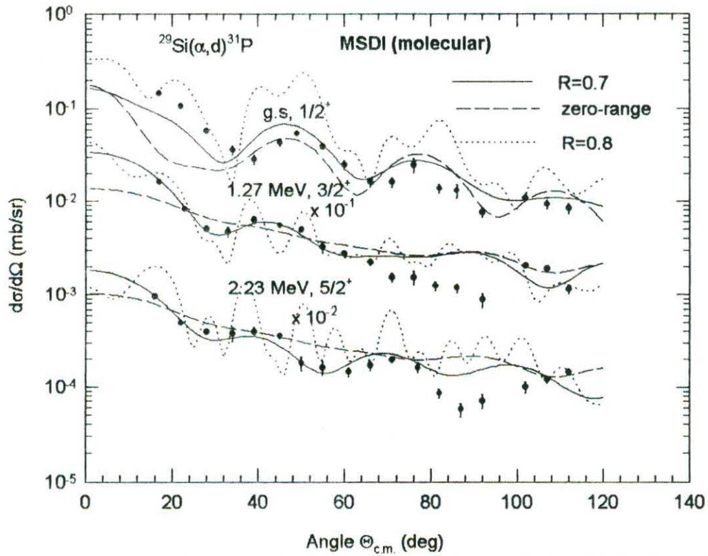
Fig.5. 24. Comparison of the zero-range microscopic DWBA calculations using the MSDI spectroscopic amplitudes and the molecular potential in the \alpha -channel for the ^{29}\text{Si}(\alpha, d)^{31}\text{P} reaction at 25 MeV leading to the ground ( 1/2^+ ), 1.27( 3/2^+ ), and 2.23( 5/2^+ ) MeV states of ^{31}\text{P} to the differential cross-section data. The solid curves are the predictions using the finite-range (FR) correction with R=0.7 fm. The broken and the dotted curves are the predictions with R=0.0 and 0.85 fm, respectively. Data are from [48]
