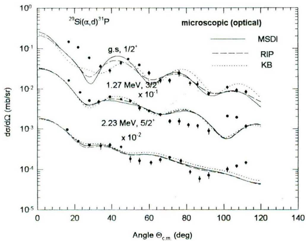
Fig. 5.28. Same as Fig. 5.25 using normal optical potential. Data are from [48].
