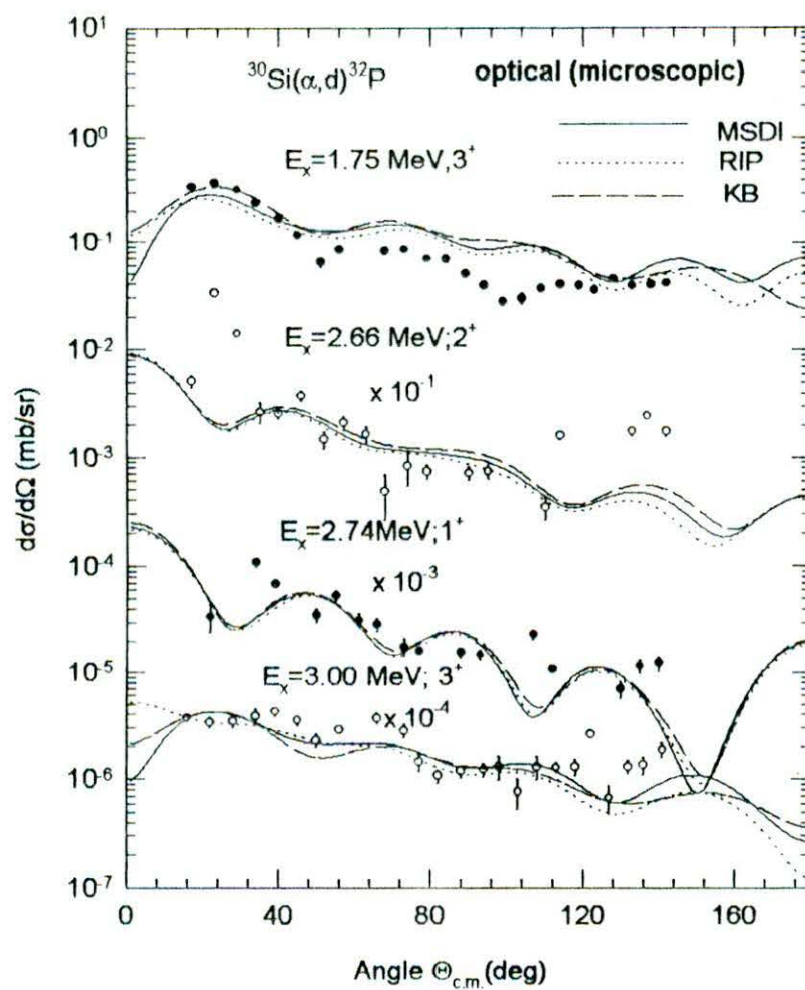
Fig. 5. 44. Same as in Fig. 5.42 using normal optical potential. Data are from [48].
