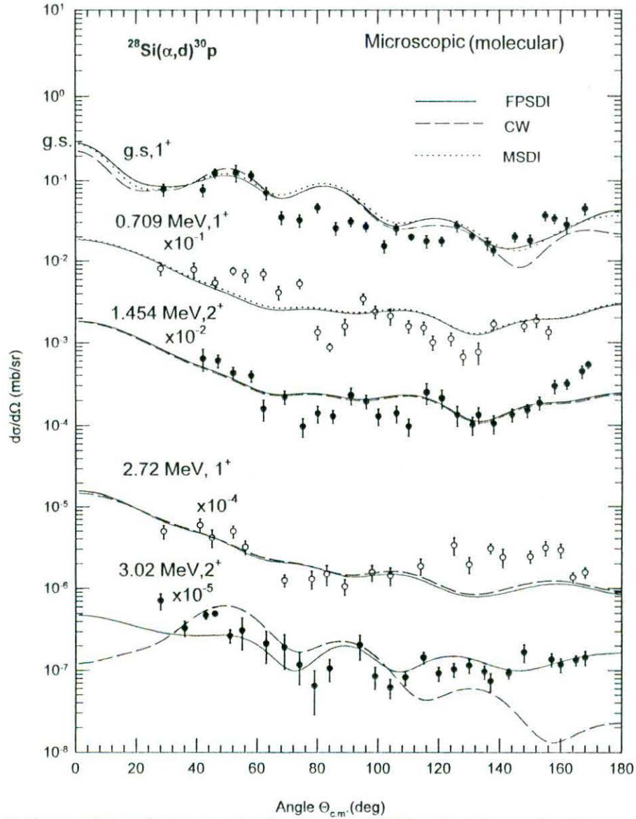
Fig. 7. Comparison of zero-range microscopic DWBA calculations with FR correction and the molecular potential for the ^{28}\text{Si}(\alpha, d)^{30}\text{P} reaction at 26 MeV, leading to the 1^+ and 2^+ states of ^{30}\text{P} to the differential cross-section data. The solid, broken and dotted curves are the predictions using the FPSDI, CW and MSDI spectroscopic amplitudes. The data are from [17].
