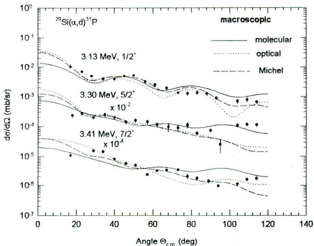
Fig. 5.22. Comparison of the full finite-range macroscopic DWBA calculations for the ^{29}\text{Si}(\alpha, d)^{31}\text{P} reaction at reaction at 25 MeV leading to the 3.13(1/2^+) , 3.30(5/2^+) , 3.41(7/2^+) MeV states of ^{31}\text{P} to the differential cross-section data. The solid, dotted and broken curves are the predictions using the molecular, normal optical and Michel \alpha - ^{29}\text{Si} potentials respectively. Data are from [48].
