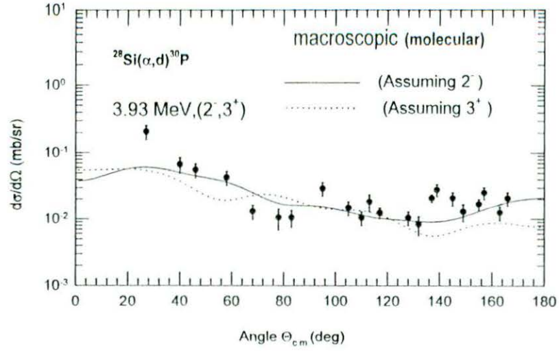
Fig. 4. Full finite-range macroscopic DWBA calculations using the molecular \alpha - ^{28}\text{Si} potential for the 3.93 MeV state assuming the spin-parity J^\pi=2^- (solid curve) and 3^+ (dotted curves) are compared to the data. The data are from [17]
