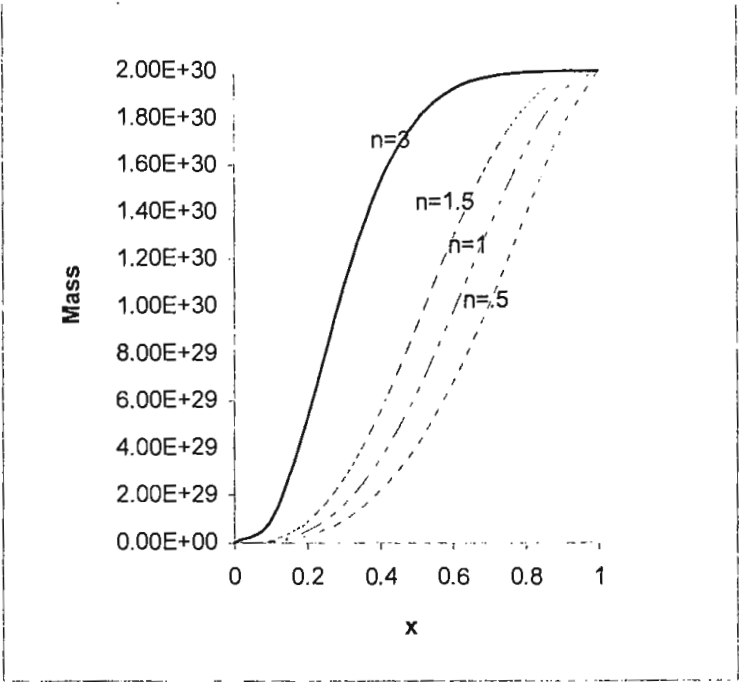
Fig. 3.1: Mass distribution in a protoplanet.
