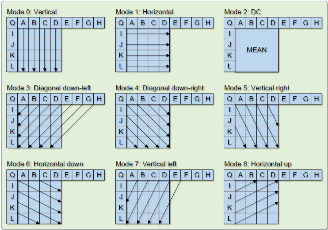
Fig. 2.6 Nine prediction mode of a 4 × 4 block.
