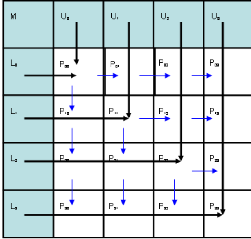
Fig. 3.2 Illustration of Intra 4 \times 4 prediction.
