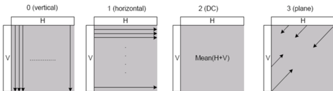
Fig. 2.7 Intra 16 \times 16 prediction modes.
