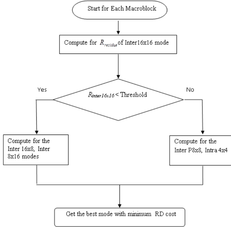
Fig. 5.1 Flow chart of proposed algorithm.
