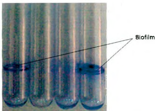
Fig. 3.19. Crystal violet stained biofilms of V. cholerae cells on borosilicate glass tubes after 24h of incubation
