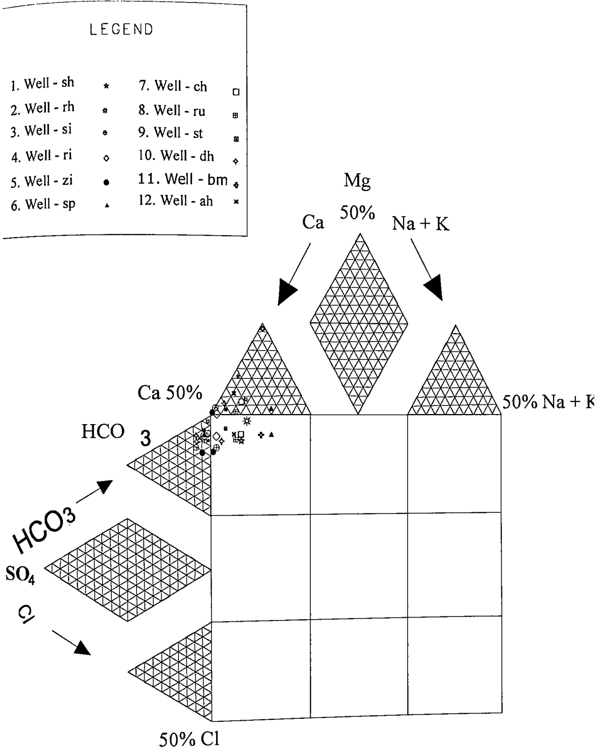
Fig. 5.9: Expanded Durov diagram of groundwater of wells of the study area.
