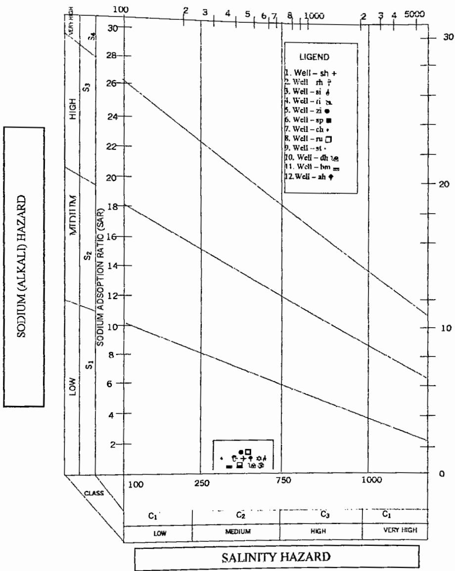
Fig. 5.4: Classification of irrigation water (USDA, 1955).
