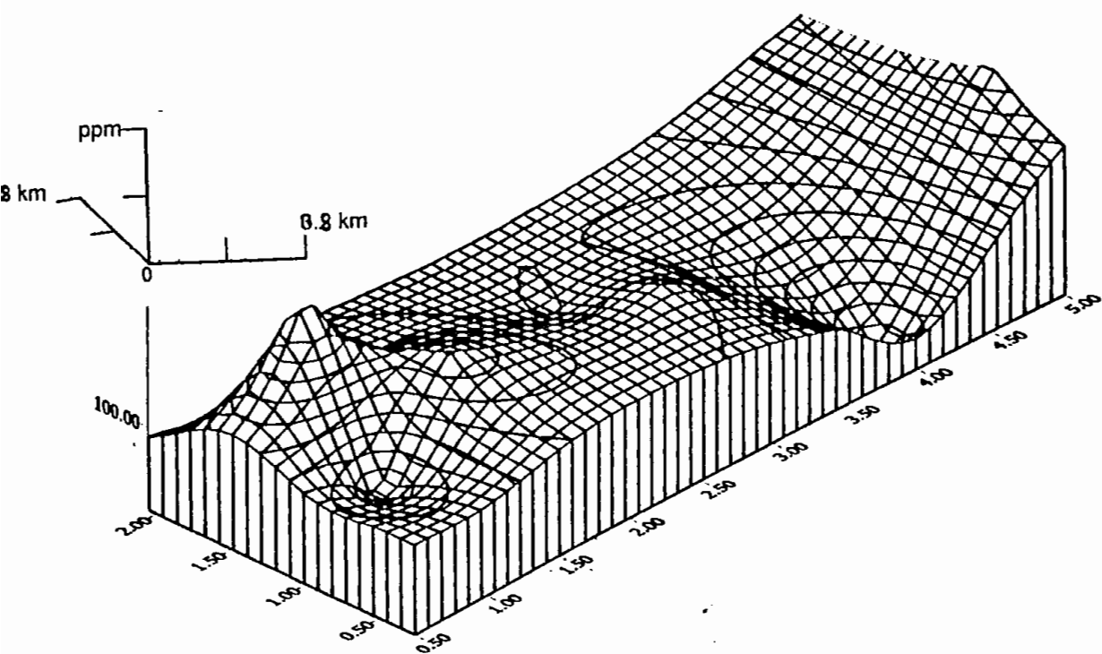
Fig. 5.2.h: 3D view of Calcium distribution in groundwater of the study area.
