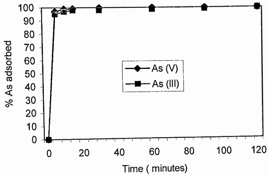
Fig. 6.3: Experimental adsoption of 1ppm arsenate and arsenite on ferric oxyhydroxide suspensions.
