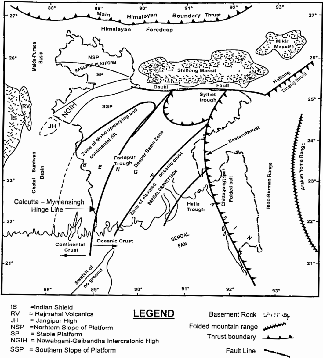
Fig. 2.1: Geotectonic map of Bengal Basin (Chaudhury & Datta 1973, Khan 1991, Khan & Rahman 1992 Khan & Agarwal, 1993).
