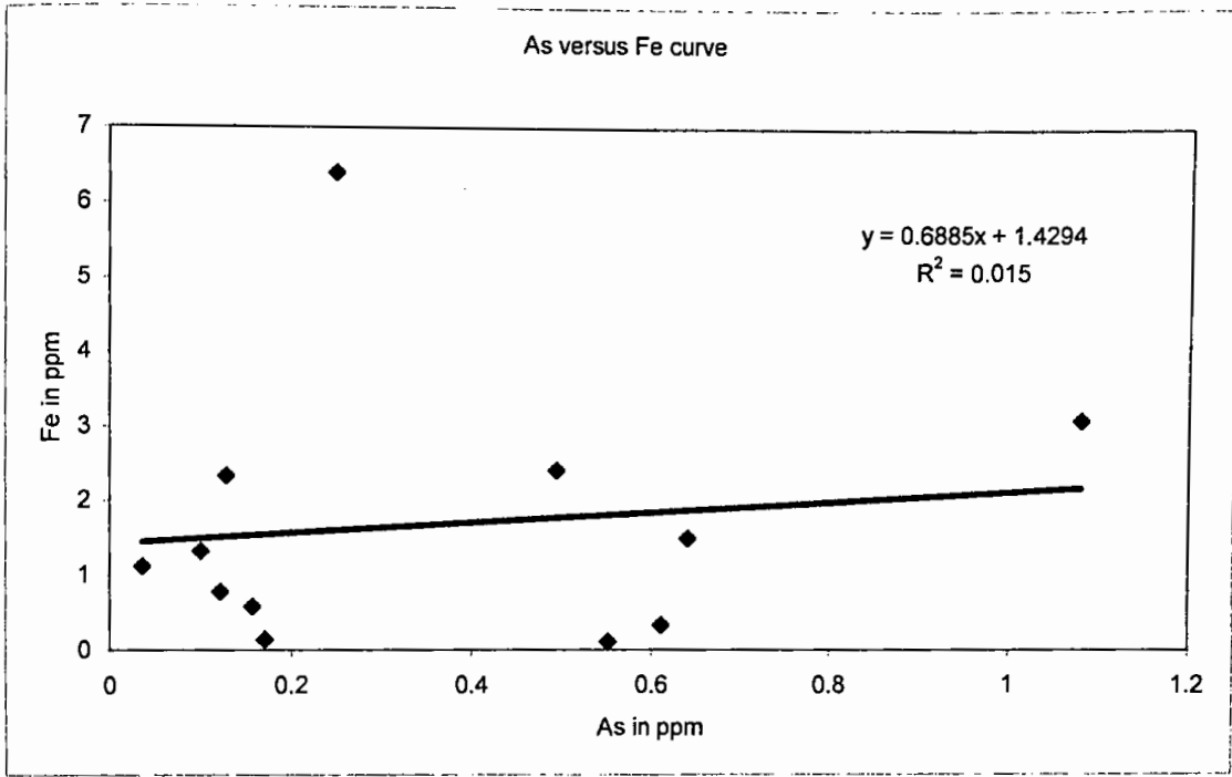
Fig. 5.11.e: Figure showing positive correlation between arsenic and total iron of groundwater of the study area.
