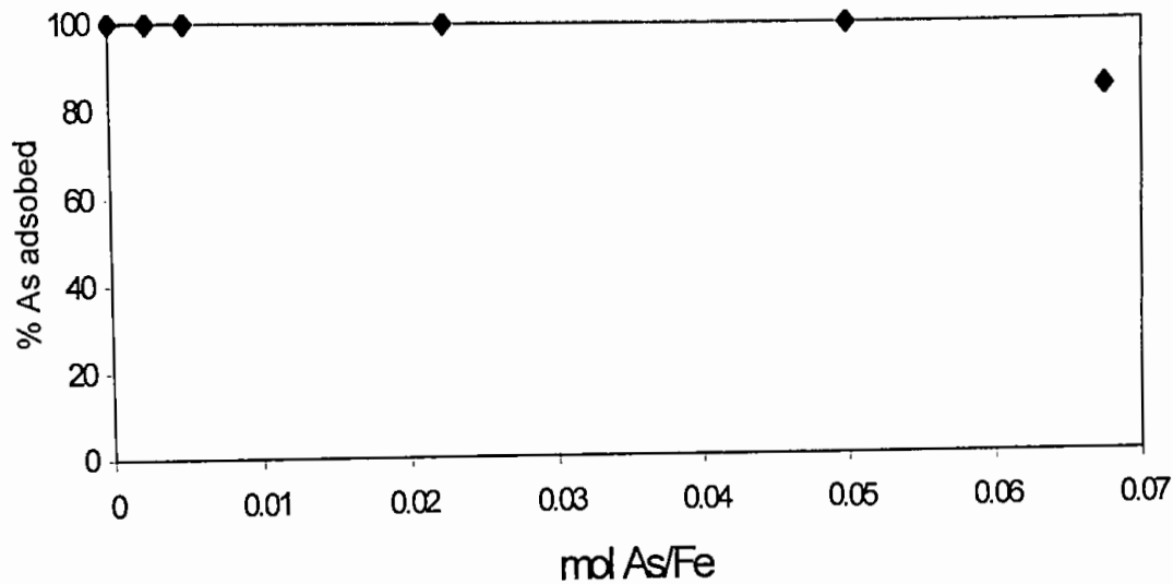
Fig 6.4: Figure showing adsorption is decreasing with increasing As/Fe molar ratio.
