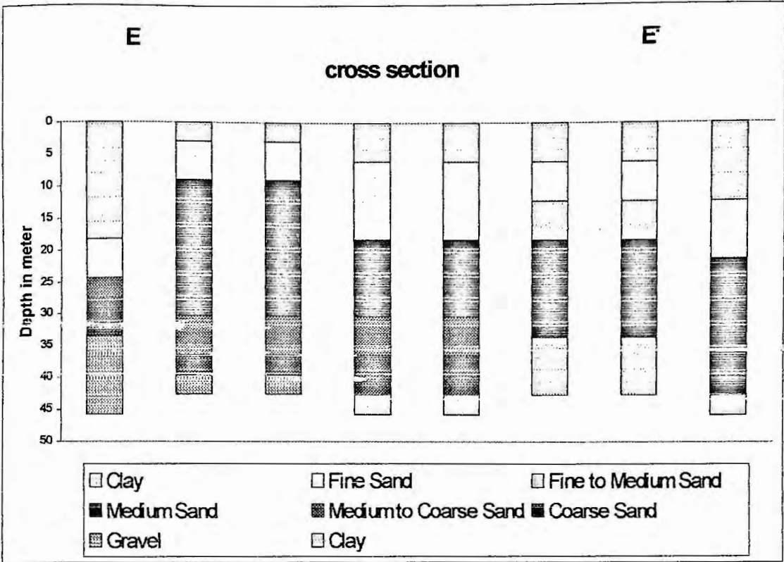
Fig. 4.10: Hydrogeological cross-section along EE'.
