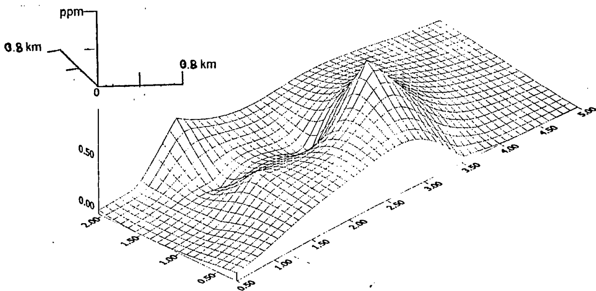
Fig. 5.3.h: 3D view of Sulfate distribution in groundwater of the study area.
