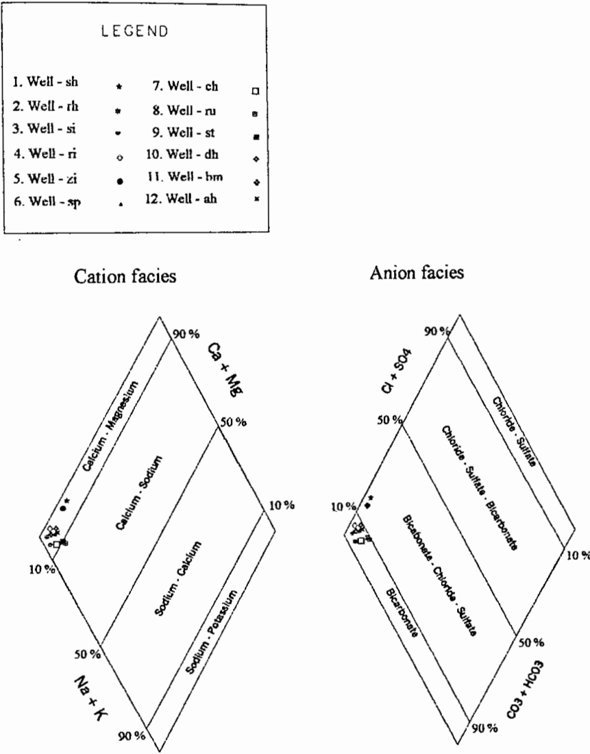
Fig. 5.10 Facies mapping approach of groundwater of the study area.
