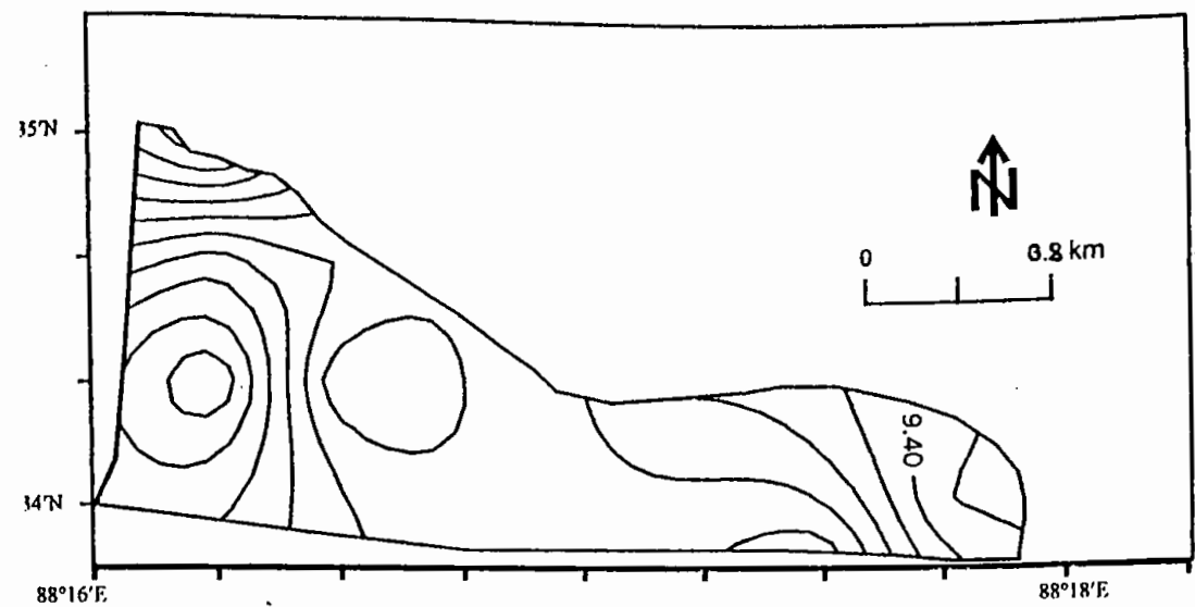
Fig. 5.2.a: Contour map showing pH distribution in groundwater of the study area.
