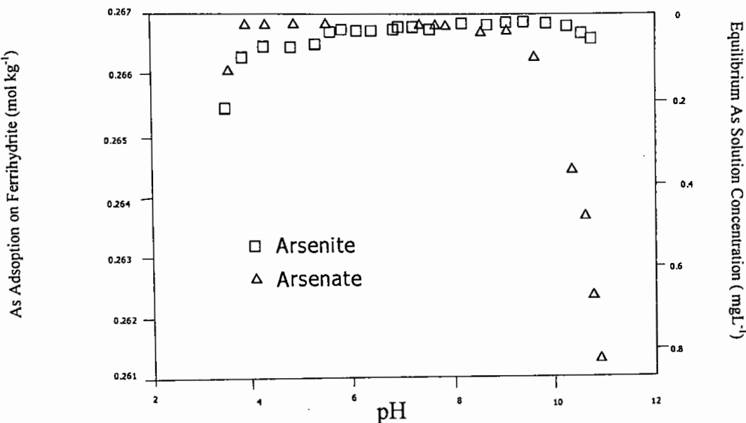
Fig. 6.2.b: Adsorption envelopes for the arsenate and arsenite with 2-line ferrihydrite at 0.1 ionic strength following the 0.267 mol AS kg fer -1 (Raven et al. , 1998).
