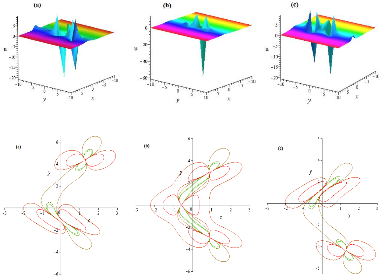
Fig-4.4: Interaction phenomena between rogue wave and solitary wave solution (4.40) for Eq. (4.21) by choosing suitable parameters: a_1 = 0.5, a_4 = 0.1, a_6 = -0.6, a_9 = 1, \lambda = 1, \mu = 2 with three-dimensional plots for different times (a) t = -15 , (b) t = 0 , and (c) t = 15 and corresponding contour plots (bottom) respectively.
