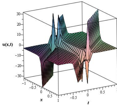
Fig-2.2: Kinky-periodic wave solution for a_4 = 1, b_1 = 0, b_2 = b_3 = w_2 = k_2 = 2, k_1 = 3 of the real part of u_{17,18} .
