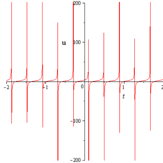
Fig-1.4: Doubly-periodic wave solution for b_0 = 2, k_1 = 1, k_2 = 2 of u_{41,42} . Fig-1.4(a): 2D plot shows the wave propagation pattern at x = 0 .
