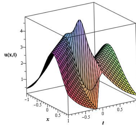
Fig-2.3: Single soliton wave solution for a_4 = 1, b_1 = 0, b_2 = b_3 = w_2 = k_2 = 2, k_1 = 3 of the real part of u_{11,12} .
