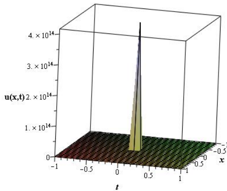
Fig-2.3: Single soliton wave solution for a_4 = 1, b_1 = 0, b_2 = b_3 = w_2 = k_2 = 2, k_1 = 3 of the real part of u_{11,12} .
