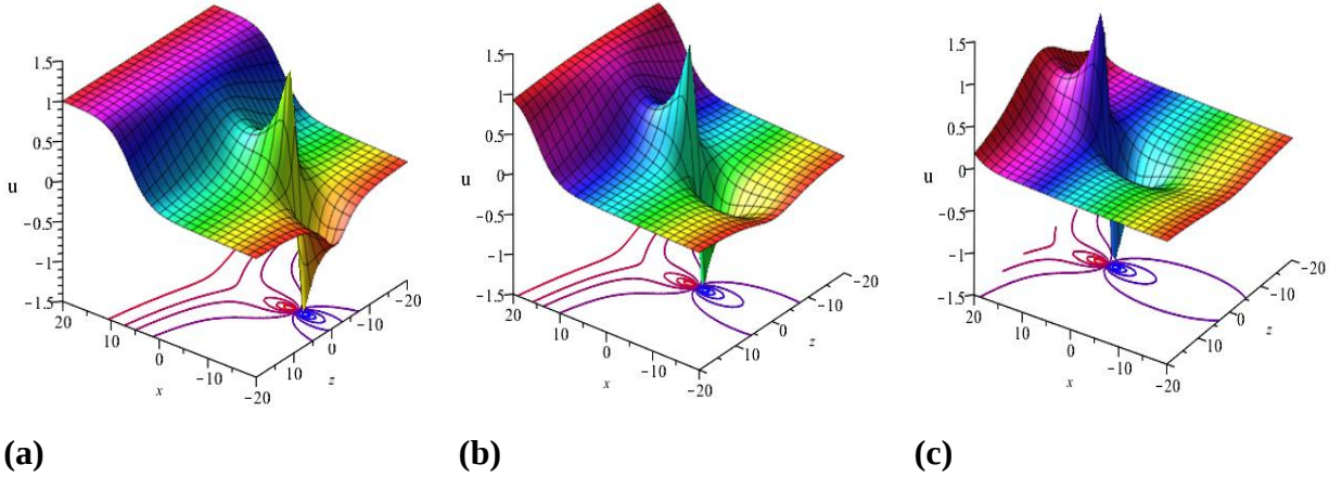
Fig-6.2: Profile of solution (4.93) for Eq. (4.85) with a_1 = a_7 = 1, a_5 = 3, a_8 = a_{10} = 2, a_{11} = 1.5, \lambda = 1.25 (a) t = -1.5 , (b) t = 0 , and (c) t = 1.5 respectively for y = 0 .
