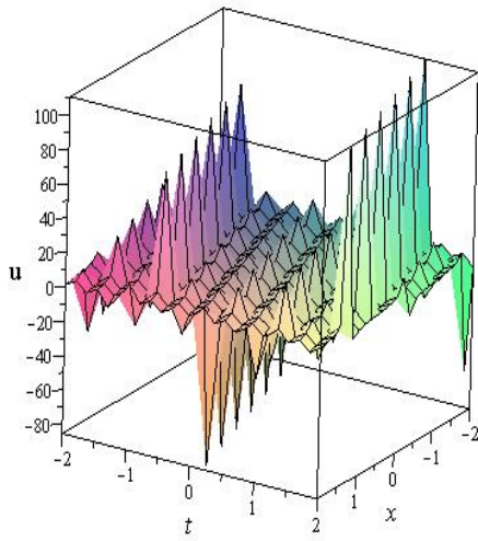
Fig-1.4: Doubly-periodic wave solution for b_0 = 2, k_1 = 1, k_2 = 2 of u_{41,42} . Fig-1.4(a): 2D plot shows the wave propagation pattern at x = 0 .
