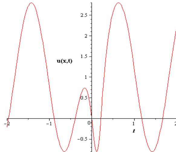
Fig-1.5: Bell-periodic wave solution for b_0 = 1, k_1 = 1, k_2 = 3 of the real part of u_{57,58} . Fig-1.5(a): 2D plot shows the wave propagation pattern x = 0 .
