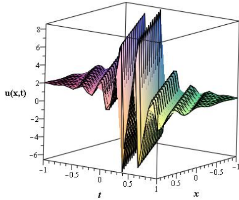
Fig-1.2: Kinky-periodic wave solution for b_0 = 1, k_1 = 1, k_2 = 5 of the real part of u_{17,18} . Fig-1.2(a): 2D plot shows the wave propagation pattern at x = 0 .
