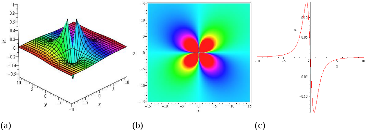
Fig-5.6: Lump solution u in (4.68) for Eq. (4.49) by choosing suitable parameters: p_1 = 1.2 , l_2 = 0.8 , m_1 = -0.8 , and m_2 = 0.4 . (a) 3-D plot of u (b) density plot of u (c) 2-D plot of u .
