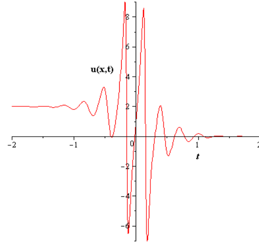
Fig-1.2: Kinky-periodic wave solution for b_0 = 1, k_1 = 1, k_2 = 5 of the real part of u_{17,18} . Fig-1.2(a): 2D plot shows the wave propagation pattern at x = 0 .
