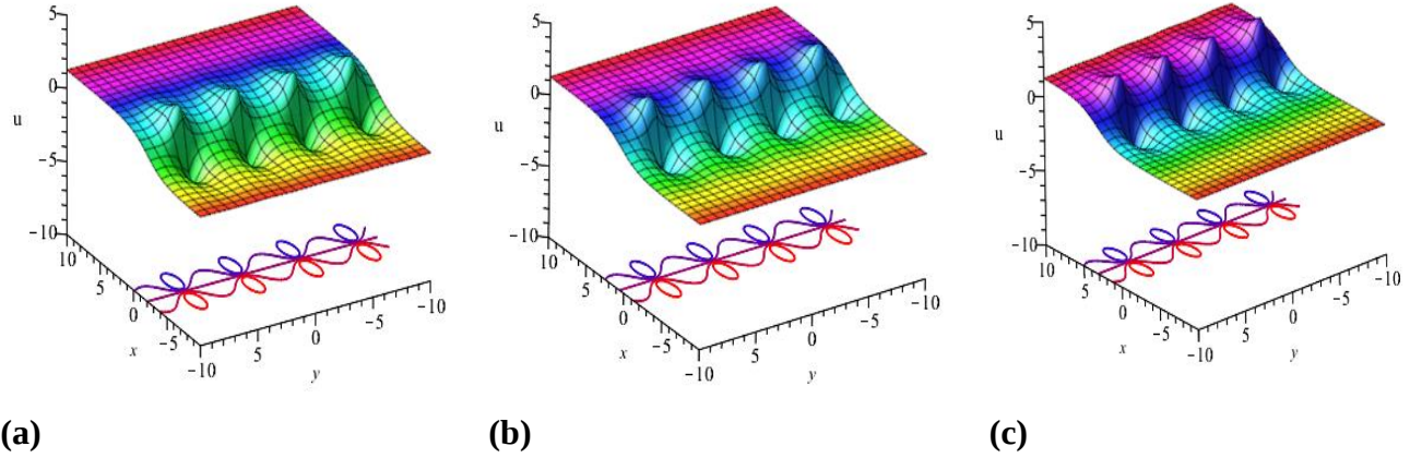
Fig-6.4: Profile of solution (4.104) for Eq. (4.85) with a_2 = b_2 = 1 , r_1 = 2.5 , h_1 = 0.5 , h_2 = 1.2 , p_1 = 0.25 , p_2 = 1.25 (a) t = -1 , (b) t = 0 , and (c) t = 1 respectively taking z = 2 .
