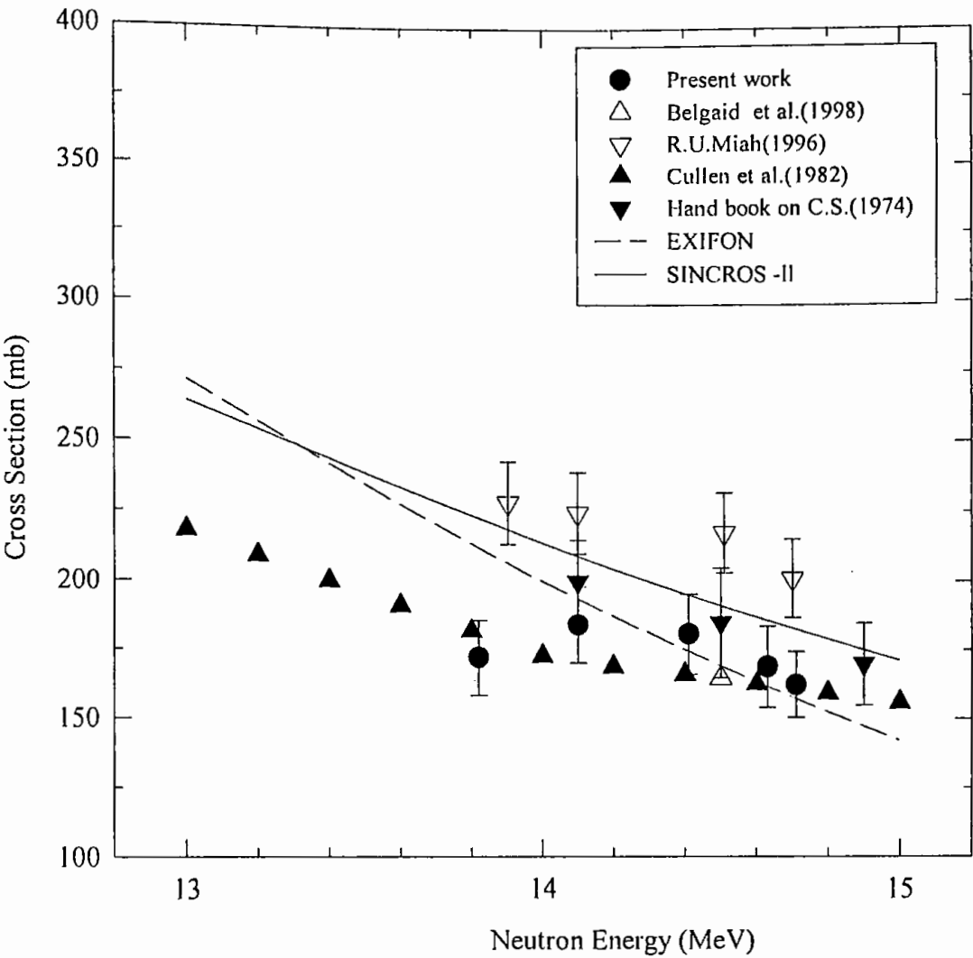
Fig. 3.6 The excitation function of ^{64}\text{Zn}(n,p)^{64}\text{Cu} reaction.
