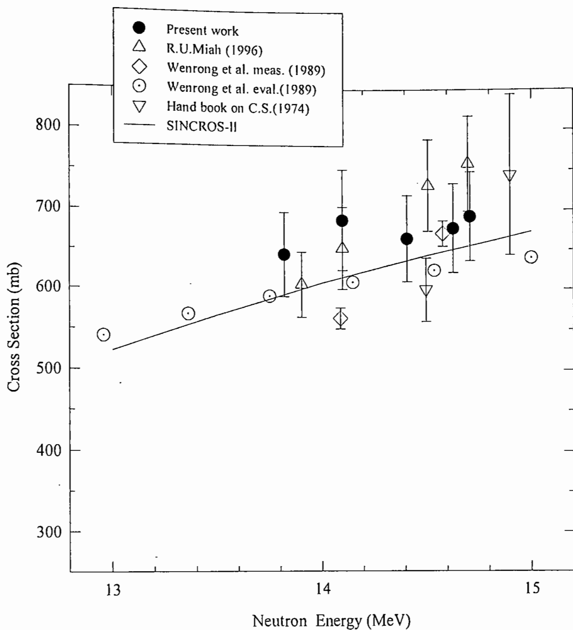
Fig. 3.7 The excitation function of ^{70}\text{Zn} (n,2n) ^{69\text{m}}\text{Zn} reaction.
