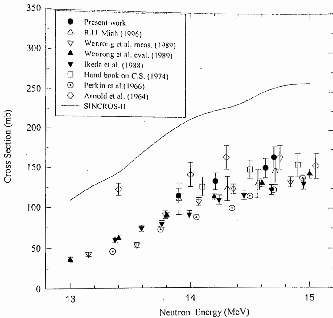
Fig.3.15 The excitation function of ^{45}\text{Sc}(n,2n)^{44\text{m}}\text{Sc} reaction
