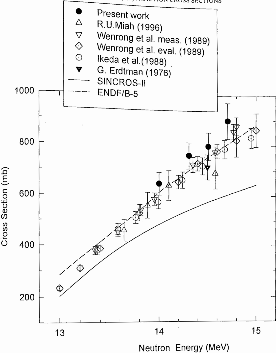
Fig.3.17 The excitation function of ^{90}\text{Zr}(n,2n)^{89}\text{Zr} reaction.
