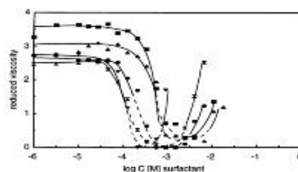
Fig. 4: Reduced viscosities of solutions of starch (0.01 wt. %, \text{DS}=0.80 ) and SDS/CTAB mixture. The molar ratios of the surfactants were 1:0 (▼), 3:1 (◆), 1:1 (●), 1:3 (▲) and 1:5 (◆). The two-phase domain is indicated by the dotted line.
