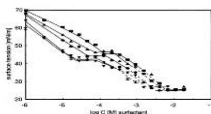
Fig. 5: Surface tensions of solutions of potato starch (0.01 wt.%, \text{DS}=0.80 ) and SDS/CTAB mixture. The molar ratios of the surfactants were 1:1 (●), 3:1 (◆), 1:0 (▼), 1:3 (▲) and 1:5 (◆). The two-phase domain is indicated by the dotted line.
