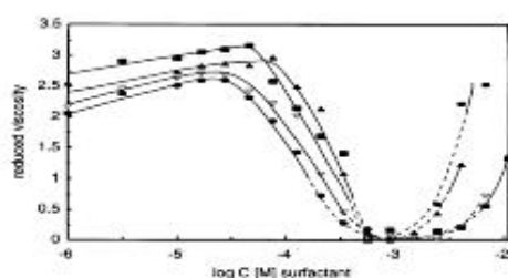
Fig. 3: Reduced viscosities of solutions of potato starch (0.01 wt.%, \text{DS}=0.80 ) and NaOct/ second surfactant mixtures. The surfactants were NaOct (●), NaOct/CTAB (▼), NaOct/SDS (◆) and NaOct/Tween-20 (▲). The molar ratio of the surfactants in the surfactant mixtures was 1:1. The two-phase domain is indicated by the dotted line.
