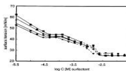
Fig. 6: Surface tension of solutions of potato starch (0.01 wt.%, \text{DS}=0.80 ) and NaOct/second surfactant mixtures. The surfactants were NaOct (●), NaOct/CTAB (▼), NaOct/SDS (◆) and NaOct/ Tween-20 (▲). The molar ratio of the surfactants in the surfactant mixtures was 1:1. The two-phase domain is indicated by the dotted line.
