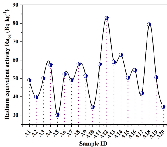
Fig. 4. Variation of radium equivalent activity for collected samples.
