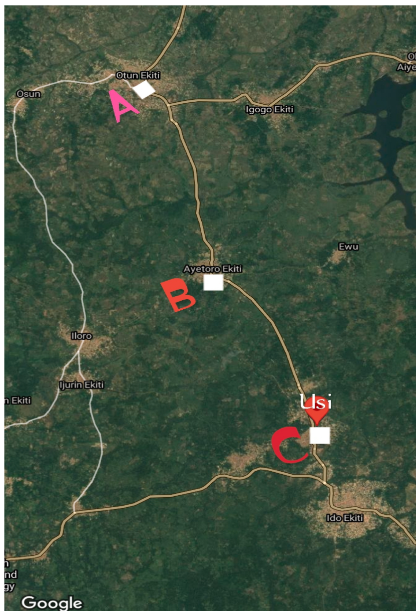
Fig. 1. Geological illustration of study area.
