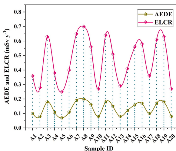
Fig. 6. variation of annual effective dose equivalent and excess lifetime cancer risk for the collected samples.
