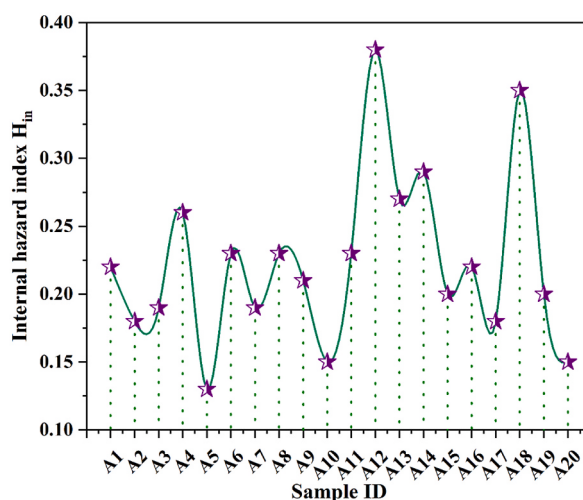
Fig. 7. variation of internal hazard index of collected samples.
