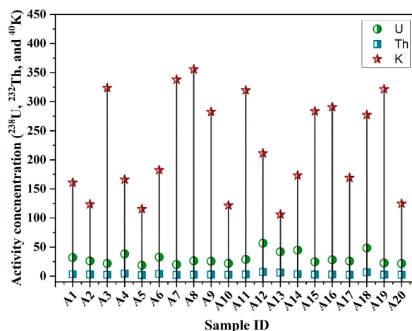
Fig. 3. Variation of the activity concentration of the collected samples.
