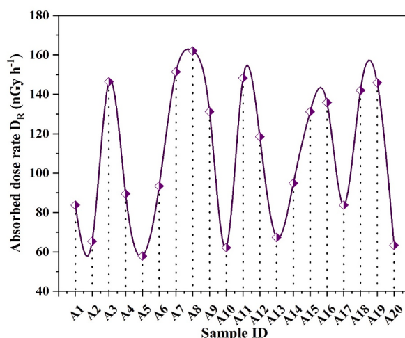
Fig. 5. Variation of Absorbed dose rate in collected samples.
