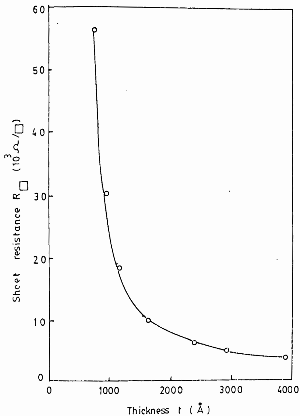
Figure 5.10: Thickness dependent of sheet resistance R_{\square} of ZnO films.
