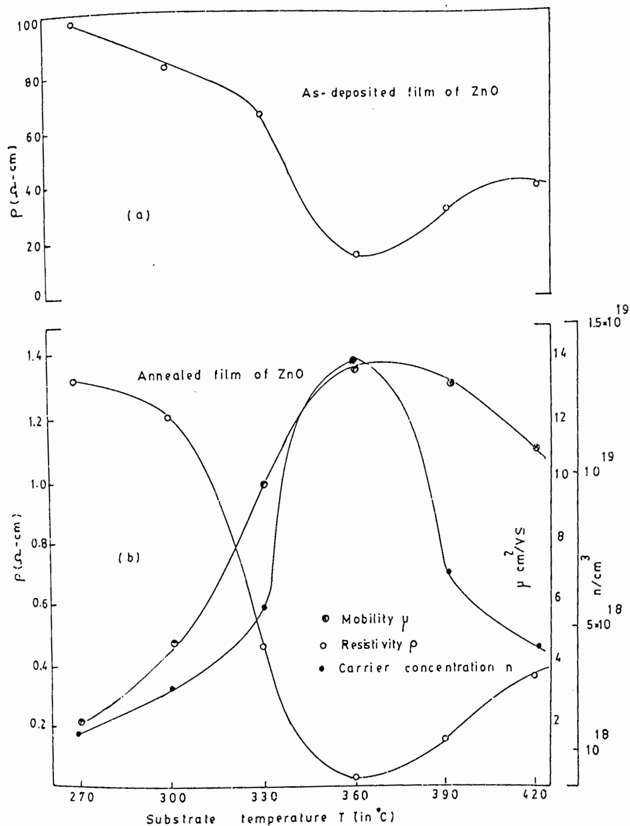
Figure 52(a): The plot of resistivity \rho vs. substrate temperature T of as-deposited ZnO films. (b): The plot of resistivity \rho , carrier concentration n and mobility \mu of vacuum heat treated ZnO films.
