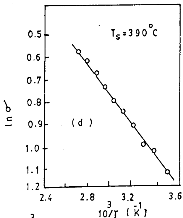
Figure 5.2 2: Plot of \ln \sigma vs. 10/T for four typical as-deposited \text{ZnO}/\text{In} films.
