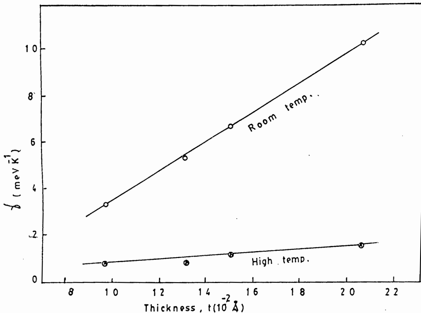
Figure 5.28: The variation of temperature coefficient of activation energy, b , as a function of thickness, t , of ZnO thin films at room temperature and high temperature.
