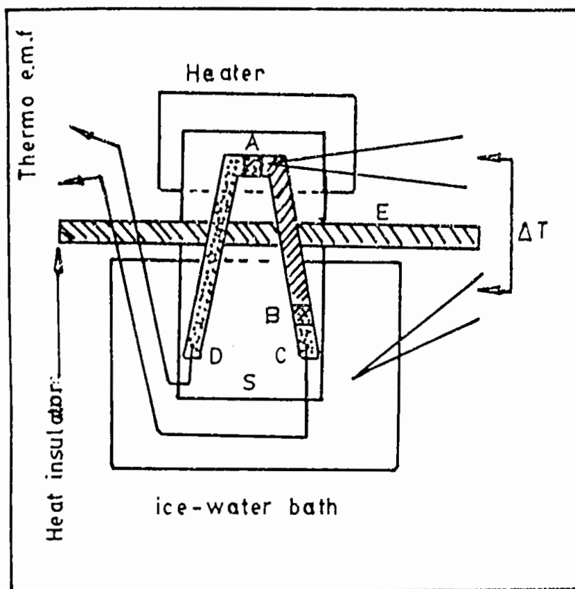
Figure 4.7: Schematic diagram of thermopower measuring apparatus AB; ZnO film; DA and BC; lead films; S, substrate; E; heat insulating barrier; \Delta T is the temperature difference between hot and cold ends.
