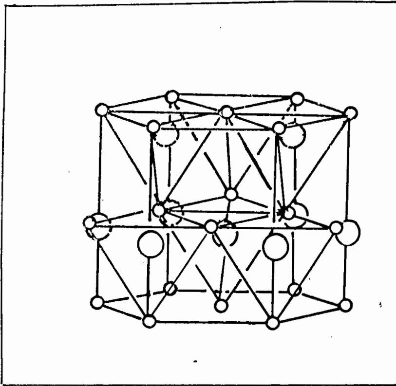
Figure 2.1 The wurtzite lattice of \text{ZnO} . Larger circles indicate zinc atoms and small circles indicate oxygen atoms.
