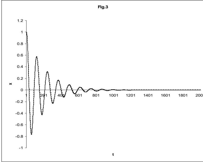
Fig 7.3: Perturbation solution (dotted line) with corresponding numerical solution (solid line) are plotted with initial conditions a = 1.004295 , \varphi = -.092516 [x(0) = 1.00000, \dot{x}(0) = 0.00000] for e = .1 , \omega_0 = 1 , h = .05 , k = .1 \cos \tau
