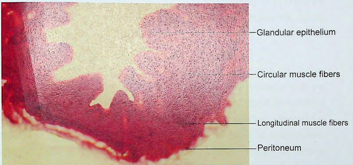
Plate 32: TS of stomach of D. limella (2.5×10)
