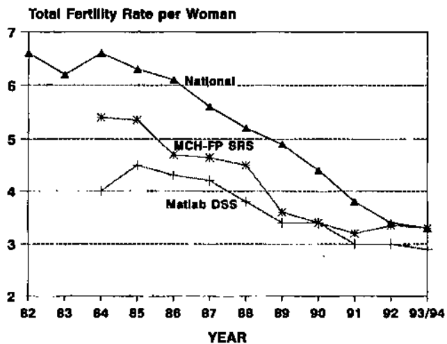
Fig. 2. TFR in Bangladesh: 1975-1994
