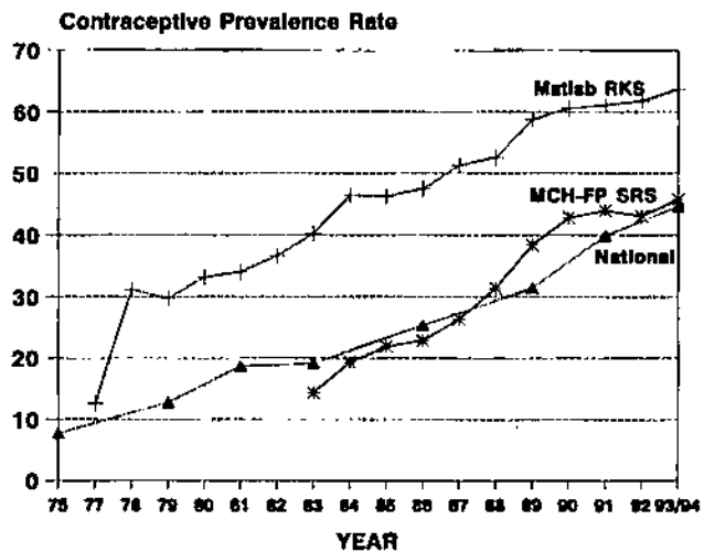
Fig. 1. CPR in Bangladesh: 1975-1994
