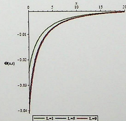
(b) 2D plot
