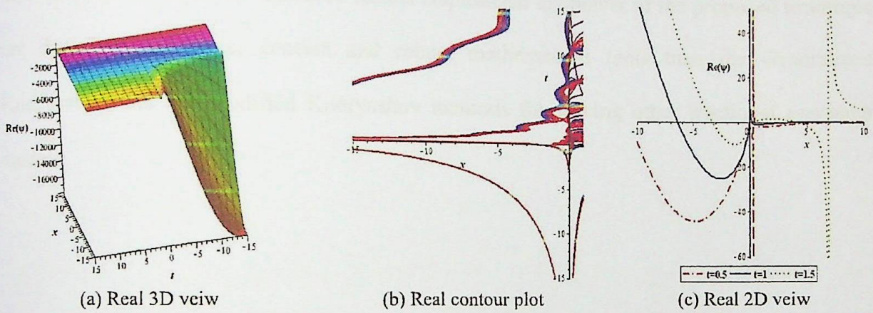
Fig-7.12: Represent the wave solution \psi(x,t) of Eq. (7.59) for \alpha = \beta = B = 0.25 , A = 1, K = 1 , w = -1, \Theta = 1, \rho = \Xi = 2, \nu = 0.5, \lambda = 1, E = 6 , and for 2D graph t = 0.5, 1, 1.5 .
