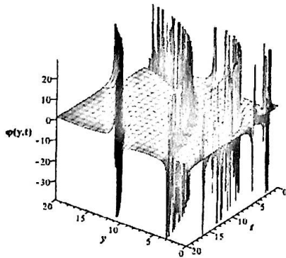
(a) 3D View of Eq.(4.52)
