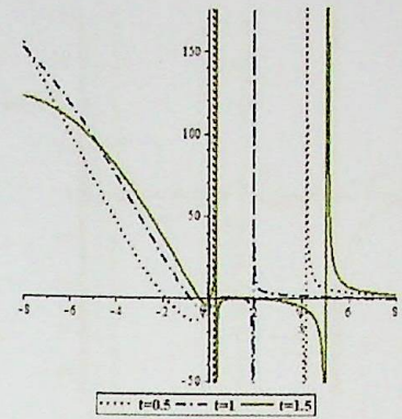
(c) Real 2D veiw
