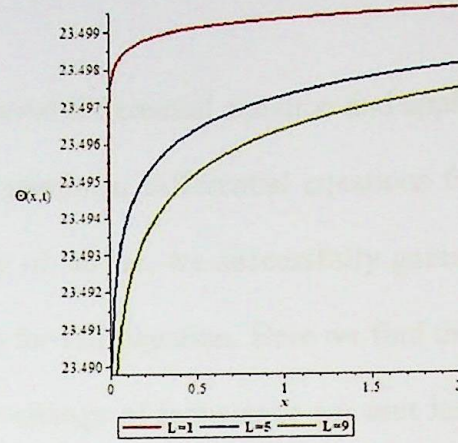
(b) 2D plot
