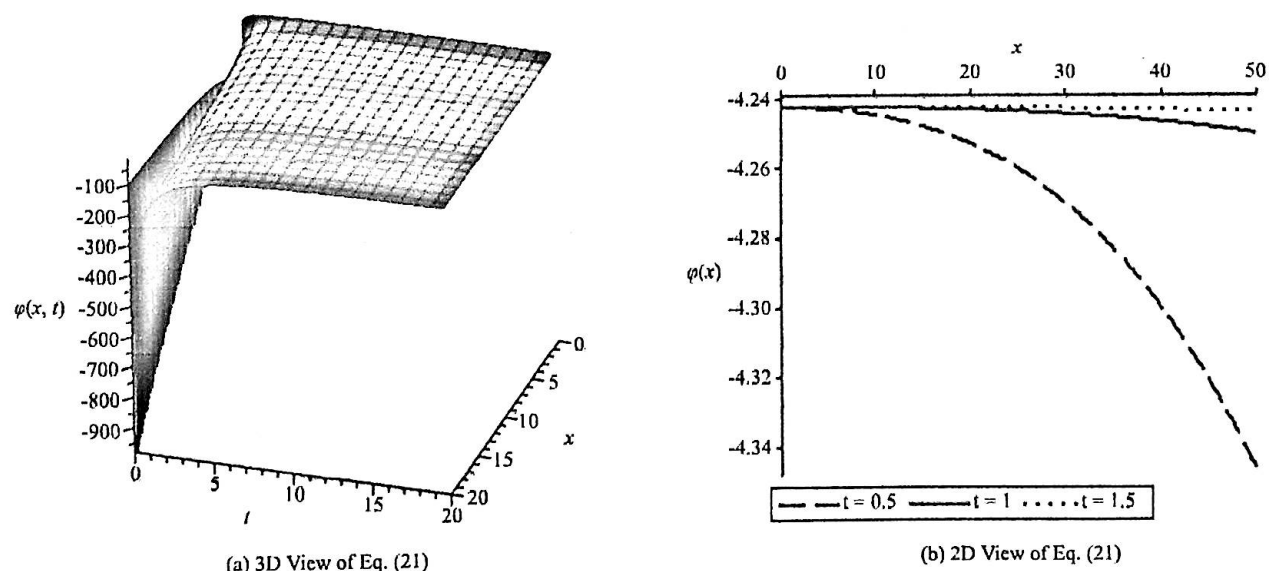
Figure 1. Represent the solitary wave \varphi(x, t) in Eq. (21) for the physical parametric values, d = 0.5 , \beta = 1/6 , c = 1 , s = 1 : (a) 3D surface, (b) 2D graphs at t = 0.5, 1, 1.5 .
