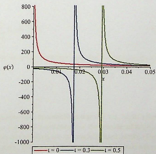
(b) 2DView of Eq. (48)
