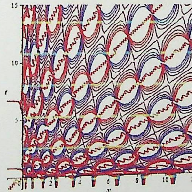
(b) Real contour plot
