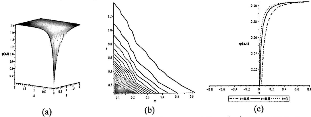
Fig-6.4: (a) Represent the imaginary part of the solitary wave solution \varphi(x, t) of Eq. (6.57) for the physical parametric values \alpha = 0.67 , k_1 = 0.5 , k_2 = 1 , \nu = 2 , A = 1 , B = 2 and t = 0.5, 0.8, 1 for 2D graph.
