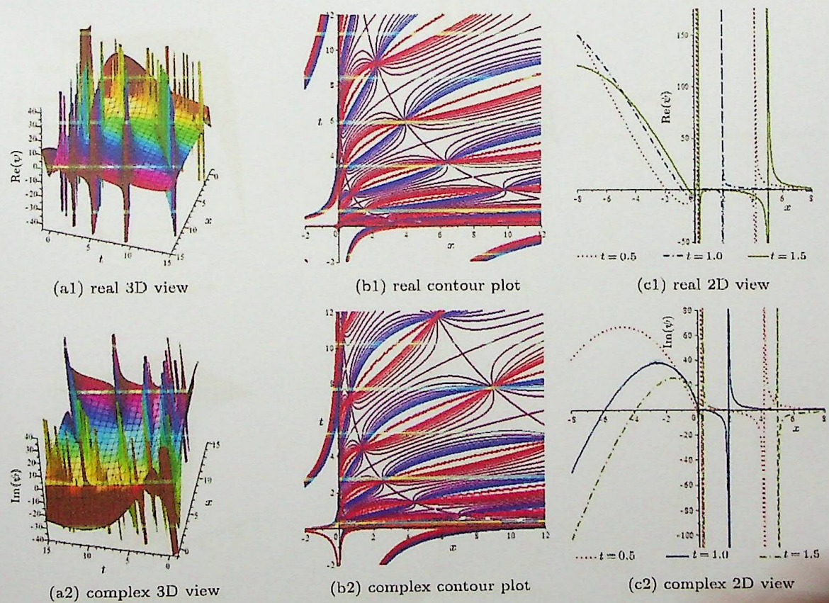
Fig. 8. Solitary wave solution \psi(x,t) of Eq. (49) for d=2 , \alpha=\beta=0.25 , A=K=\lambda=\Theta=\sigma=1 , w=-1 , \rho=2 , E=2 , v=3 , E=6 , and t=0.5, 1 , and 1.5 for 2D graph.
