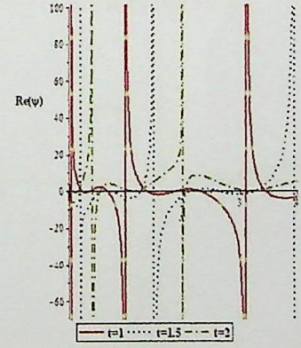
(c) Real 2D veiw
