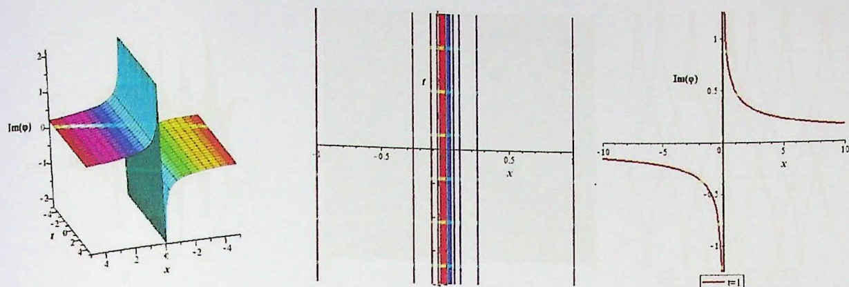
(b) Imaginary contour shape
