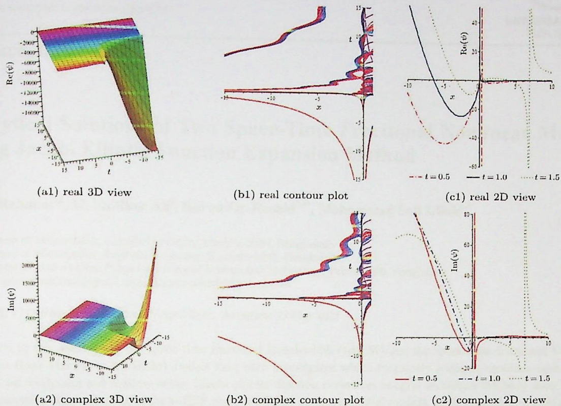
Fig. 13. Solution \psi(x, t) of Eq. (61) for d=2 , \alpha=\beta=B=0.25 , A=K=1 , w=-1 , \Theta=1 , \rho=\Xi=2 , v=12 , \lambda=1 , and E=6 , and for 2D graph, t=0.5, 1 , and 1.5 .
