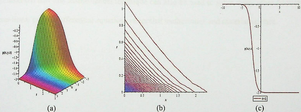
Fig-5.5: Represent the imaginary part of the solution p(x, y, t) of Eq. (5.17) for the physical parametric values A = 1 , \gamma = 3/4 , k = 2 , \ell_1 = 1 , \nu = -2 , \rho = 1 , \phi_1 = 1 , y = 0 and t = 1 for 2D graph.
