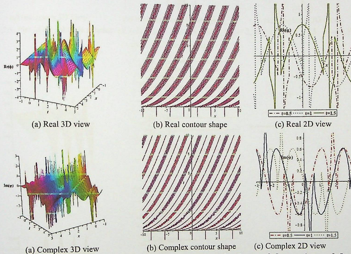
Fig-7.4: Represent the solitonic solution \varphi(x,t) of Eq. (7.36) for d = 2, \varphi_1 = 0.5, \varphi_0 = 1, \gamma = 0.5, k = 0.8 and t = 0.5, 1, 1.5 for 2D graph
