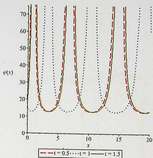
(b) 2D View of Eq. (27)
