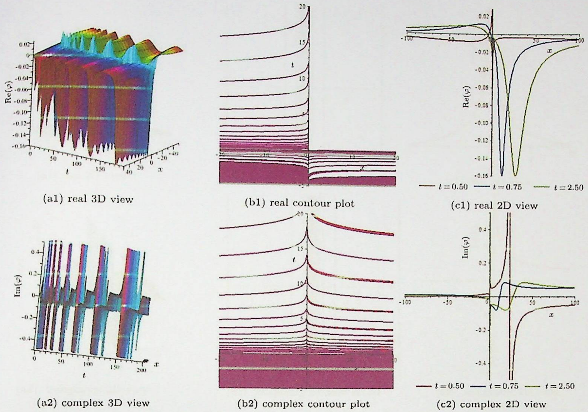
Fig. 3. (a), (b) Real and complex 3D surface and contour plot of solution \phi(x, t) of Eq. (30) for k = -2 , \beta = 0.1 , f_2 = 1 , \nu = 3 , A = 2 , B = -1 , and k_2 = 2 , and (c) 2D plot for t = 0.5, 0.75 , and 2.5 with parametric values above.
