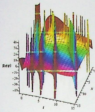
(a) Real 3D veiw
