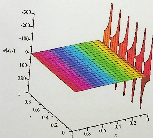
(a) 3D View of Eq. (48)
