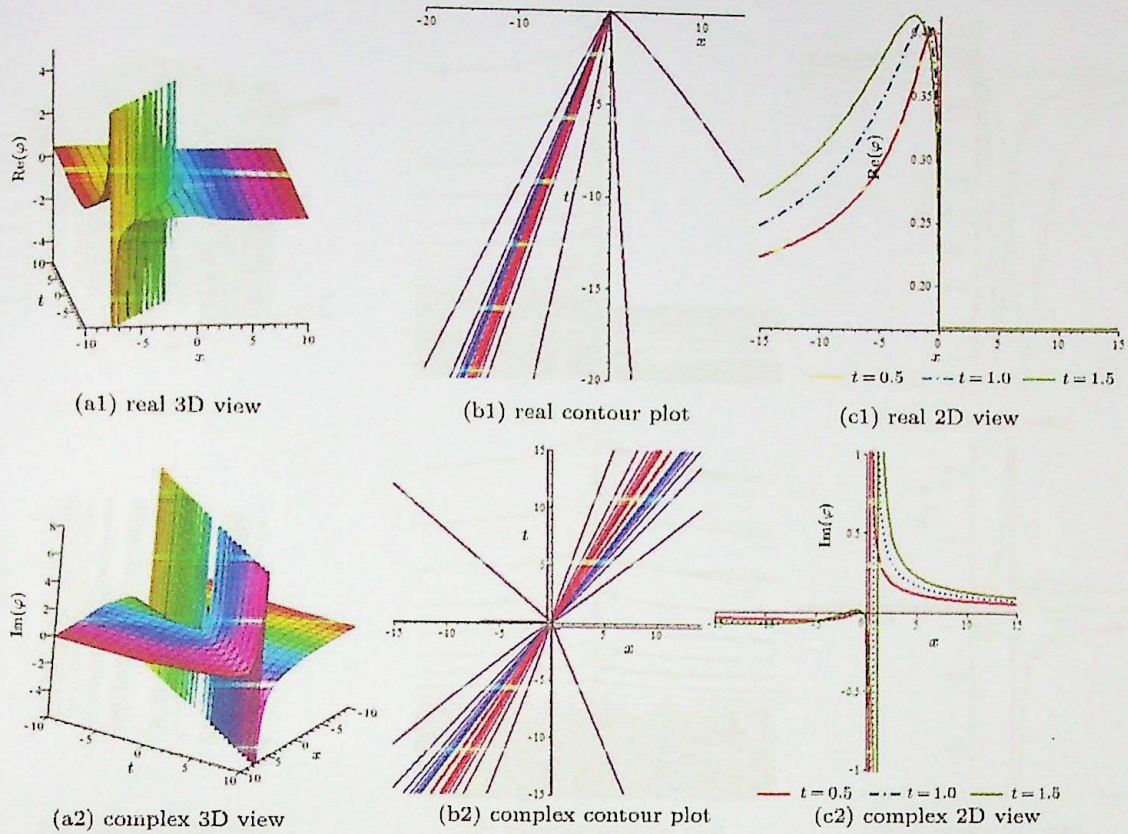
Fig. 1. (a), (b) Real and complex three-dimensional (3D) surface and contour plot of solution \phi(x, t) of Eq. (12) for k = 2 , \beta = 0.1 , \nu = 0.5 , A = 1 , and B = -1 , and (c) two-dimensional (2D) plot for t = 0.5, 1 and 1.5 with parametric values above.
