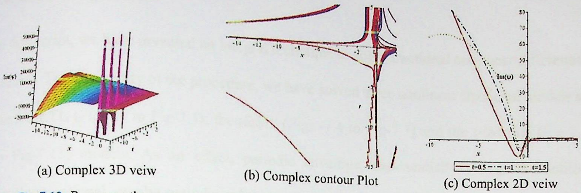
Fig-7.12: Represent the wave solution \psi(x,t) of Eq. (7.59) for \alpha = \beta = B = 0.25 , A = 1, K = 1 , w = -1, \Theta = 1, \rho = \Xi = 2, \nu = 0.5, \lambda = 1, E = 6 , and for 2D graph t = 0.5, 1, 1.5 .
