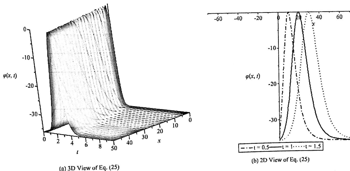
Figure 3. Represent the bell type solitary wave \varphi(x, t) in Eq. (25) for the physical parametric values, d = 1 , \beta = 3/5 , c = 3 , \varepsilon = 0.25 : (a) 3D surface and (b) 2D graphs for and t = 0.5, 1, 1.5 .
