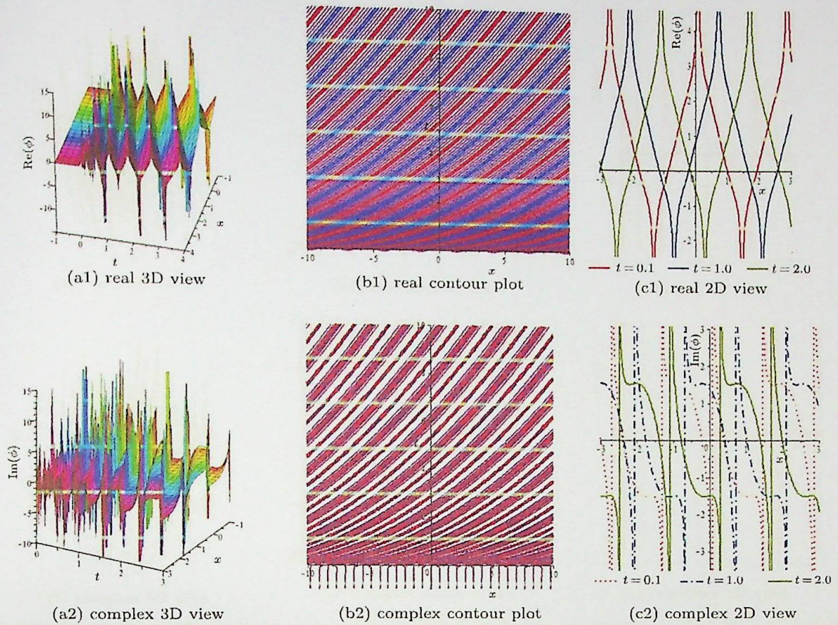
Fig. 7. Solitonic solution \phi(x,t) of Eq. (42) for d=2 , g_1=0.5 , g_0=1 , \gamma=0.5 , and k=0.8 and t=0.1, 1 , and 2 for 2D graph.
