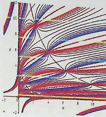
(b) Real contour plot
