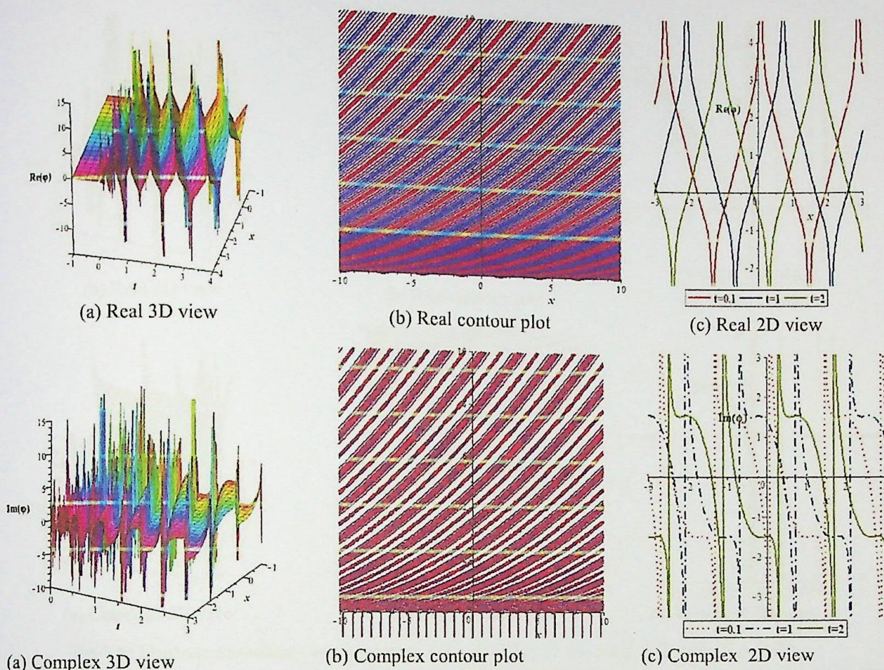
Fig-7.7: Represent the solitonic solution \varphi(x, t) of Eq. (7.42) for d = 2 , \wp_1 = 0.5 , \wp_0 = 1 , \gamma = 0.5 , k = 0.8 and t = 0.1, 1, 2 for 2D graph.
