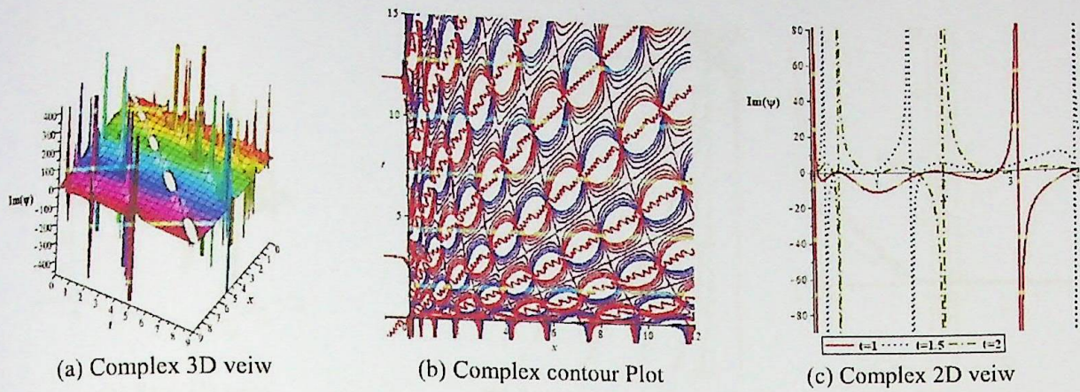
Fig-7.9: Represent the solitonic solution \psi(x, t) of Eq. (7.52) for d = -2, \alpha = 0.5, \beta = B = 0.75, A = 2, K = 5, w = -1, \Theta = 3, \rho = 1, \Xi = 4, \nu = 1, \lambda = 1, E = 6, \sigma = 3 , and t = 1, 1.5, 2 for 2D graph.
