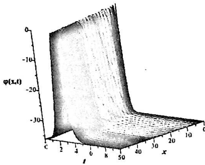
(a) 3D View of Eq.(4.25)
