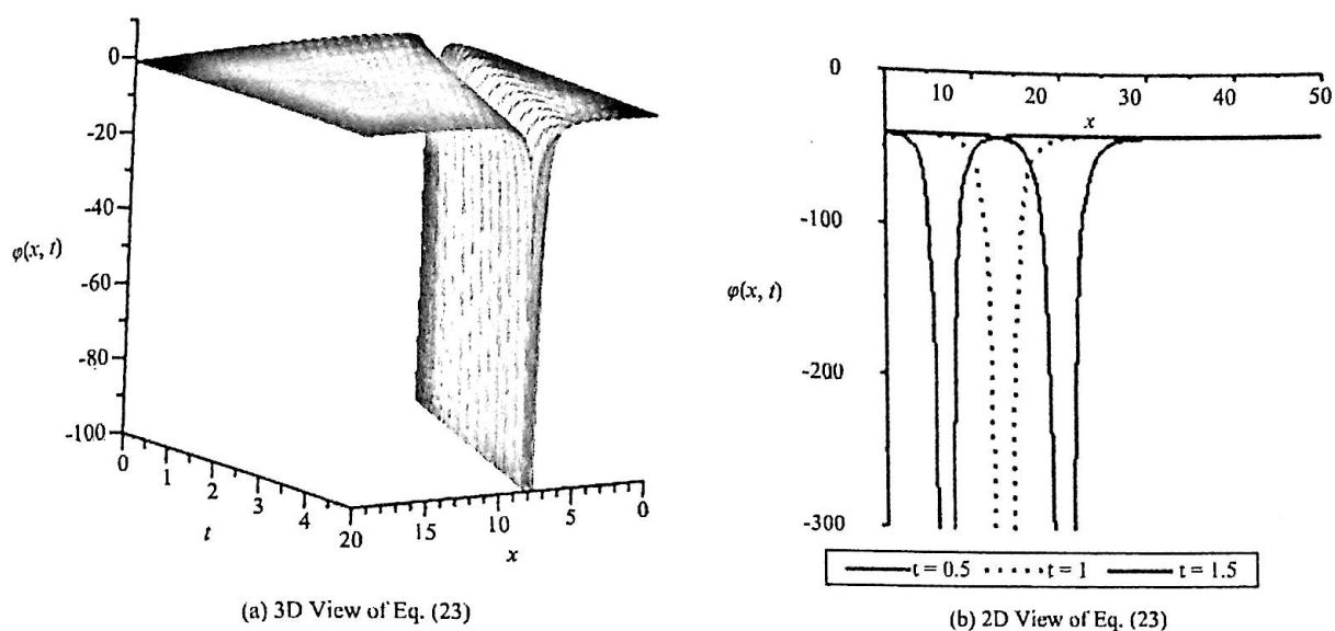
Figure 2. Represent the solitary wave \varphi(x, t) in Eq. (23) for the physical parametric values, d = 0.5 , \beta = 3/4 , c = 5 , \varepsilon = 2 : (a) 3D surface and (b) 2D graphs at t = 0.5, 1, 1.5 .
