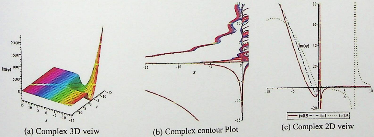
Fig-7.13: Represent the solution \psi(x,t) of Eq. (7.61) for d = 2, \alpha = \beta = B = 0.25 , A = K = 1 , w = -1, \Theta = 1, \rho = \Xi = 2, \nu = 12, \lambda = 1, E = 6 , and for 2D graph t = 0.5, 1, 1.5
