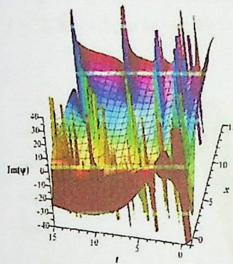
(a) Complex 3D veiw
