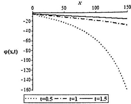
(b) 2D View of Eq.(4.21)
