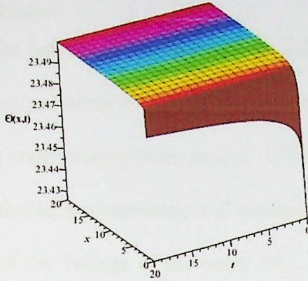
(a) 3D surface
