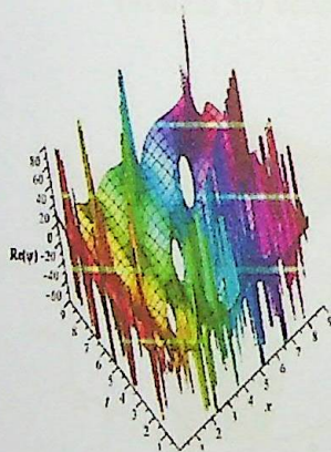
(a) Real 3D view
