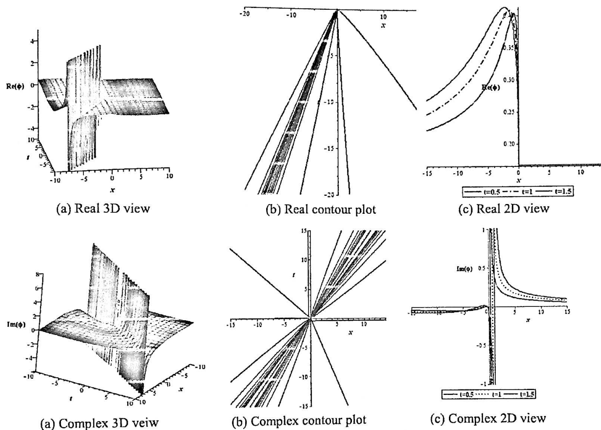
Fig-7.1. (a), (b) Real and complex 3D surface and contour plot of solution \phi(x, t) of Eq.(7.12) for k = 2, \beta = 0.1, v = 0.5, A = 1 , and B = -1 and (c) 2D plot for t = 0.5, 1 , and 1.5 with parametric values above
