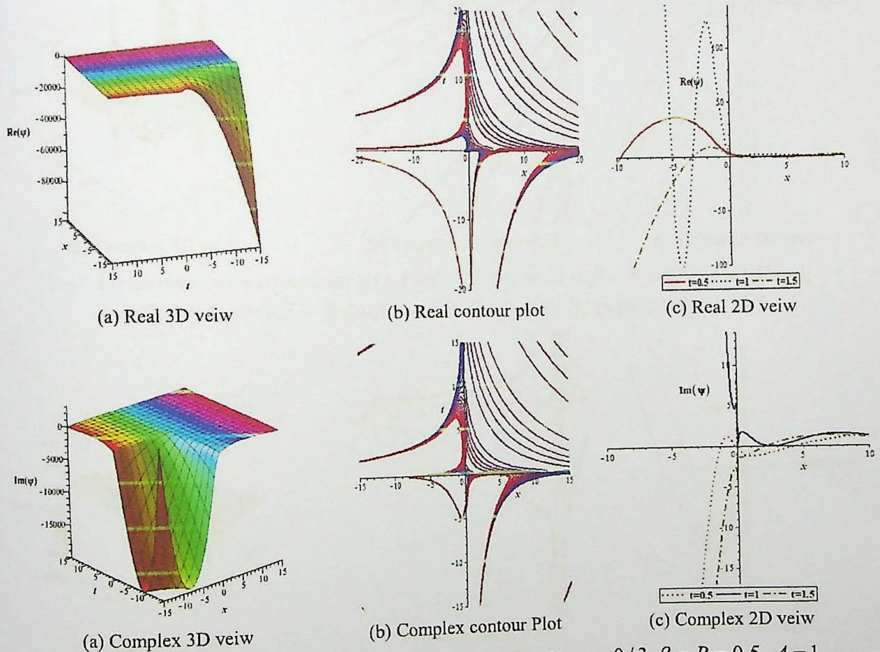
Fig-7.10: Represent the solitonic solution \psi(x, t) of Eq. (7.54) for \alpha = 0/3, \beta = B = 0.5, A = 1, K = 1, w = -1, \Theta = 1, \rho = 2, \Xi = 2, \nu = 0, \lambda = 1, E = 6 and for 2D graph t = 0.5, 1, 1.5 .
