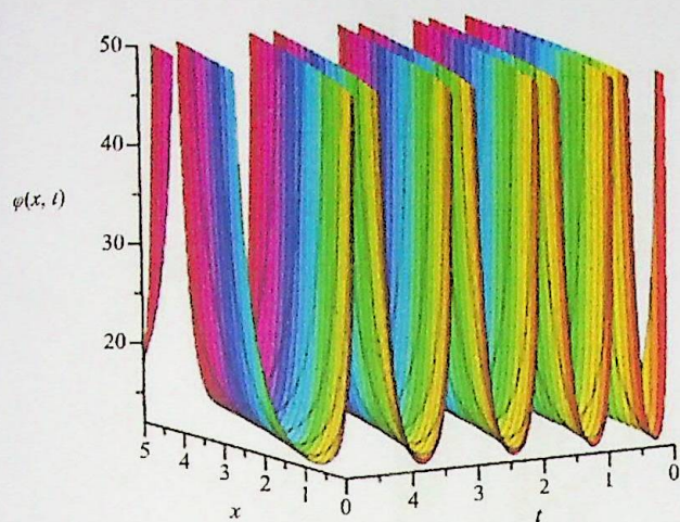
(a) 3D View of Eq. (27)
