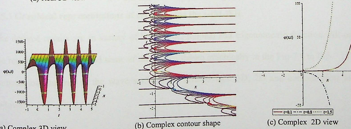
Fig-7.6: Represent the solitonic solution \varphi(x, t) of Eq. (7.39) for d = -2, \rho_1 = 2, \rho_0 = 1, \gamma = 4/5, k = 1 and t = 0.1, 0.8, 1.5 for 2D graph.
