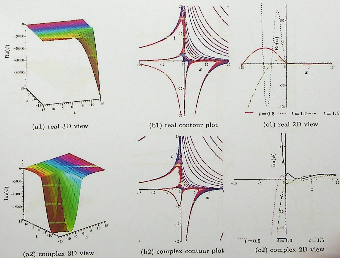
Fig. 10. Solitonic solution \psi(x, t) of Eq. (54) for \alpha = 0/3 , \beta = B = 0.5 , A = 1 , K = 1 , w = -1 , \Theta = 1 , \rho = 2 , \Xi = 2 , v = 0 , \lambda = 1 , and E = 6 and for 2D graph t = 0.5, 1 , and 1.5 .
