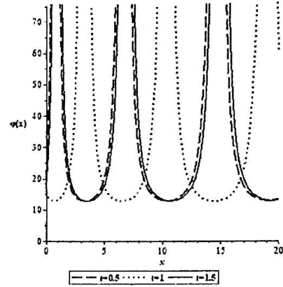
(b) 2D View of Eq.(3.27)
