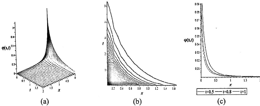
Fig-6.3: (a) Represent the solitary wave solution \varphi(x, t) of Eq. (6.48) for the physical parametric values \alpha = 0.5 , k_1 = 0.5 , k_2 = 1 , \nu = 2 , A = 1 , B = 0.8 , and t = 0.5, 0.8, 1 for 2D graph.
