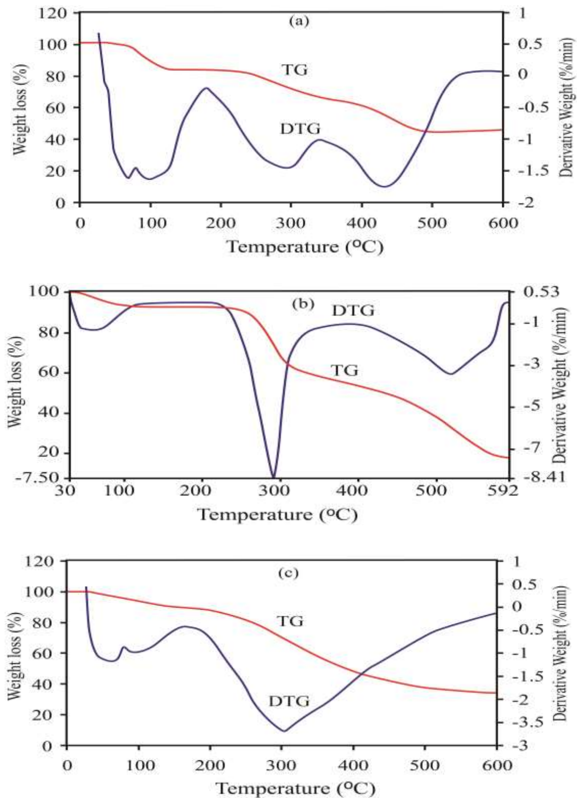
Figure 3.7: TG and DTG curve of (a) Aloe vera , (b) Chitosan, and (c) Silk sericin
